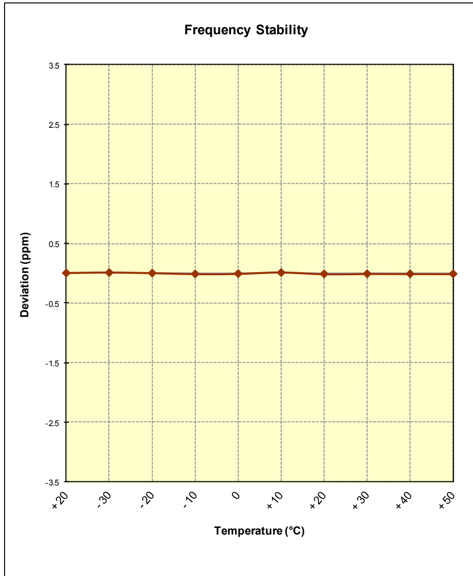
Figure 6-9. Frequency Stability Graph (PCS GSM Mode – Ch. 661)
