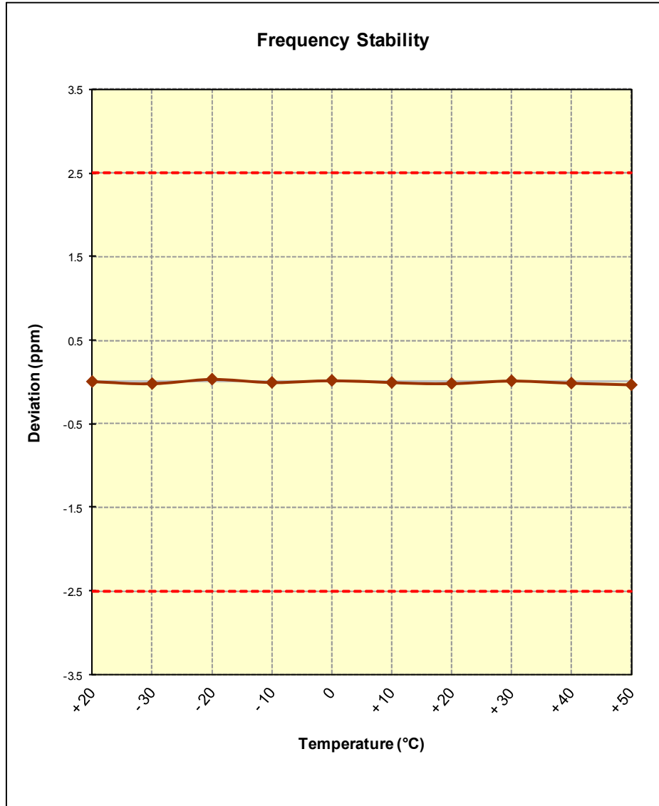
Figure 6-7. Frequency Stability Graph (Cellular GSM Mode – Ch. 190)
