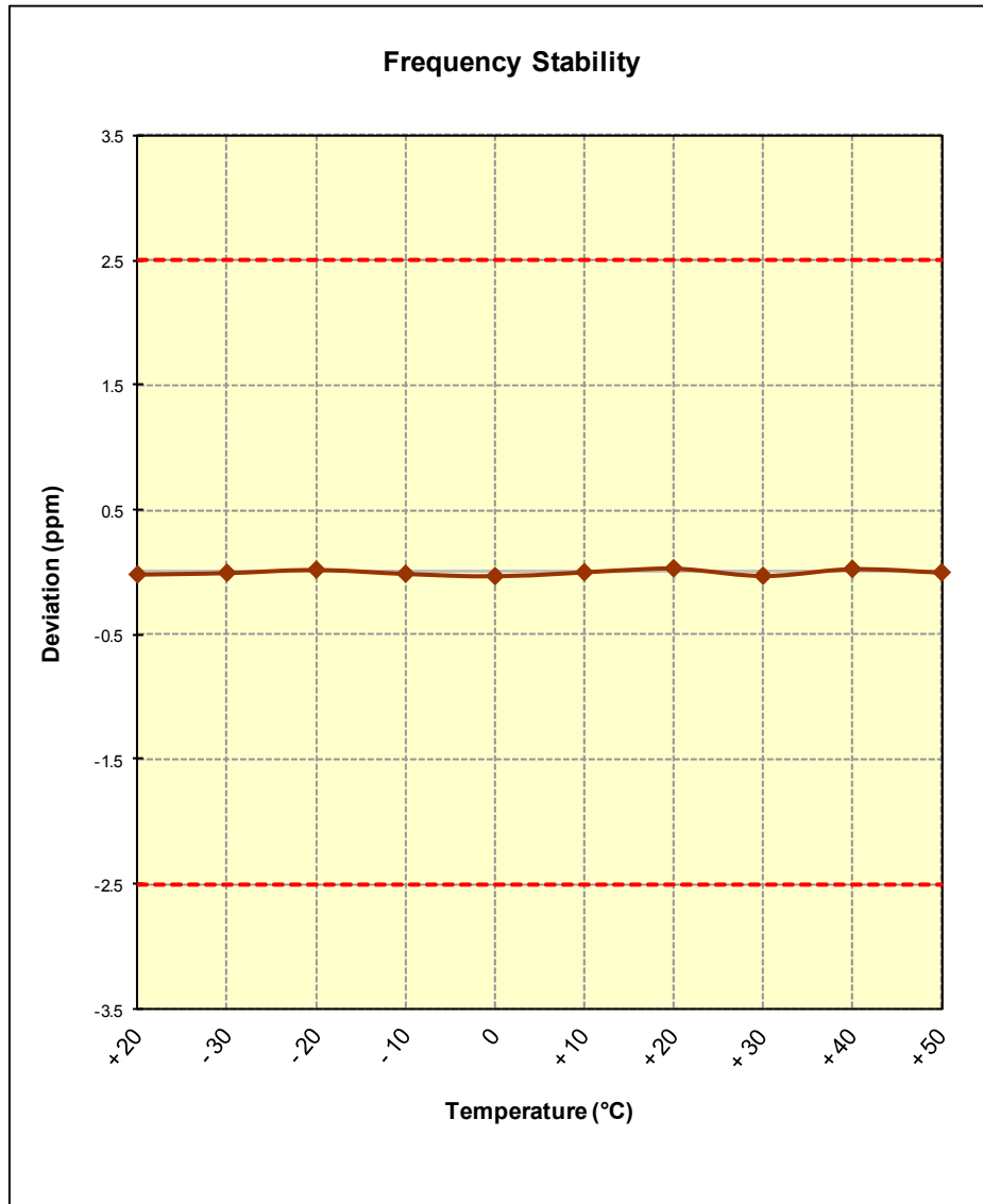
Figure 6-8. Frequency Stability Graph (Cellular WCDMA Mode – Ch. 4183)
