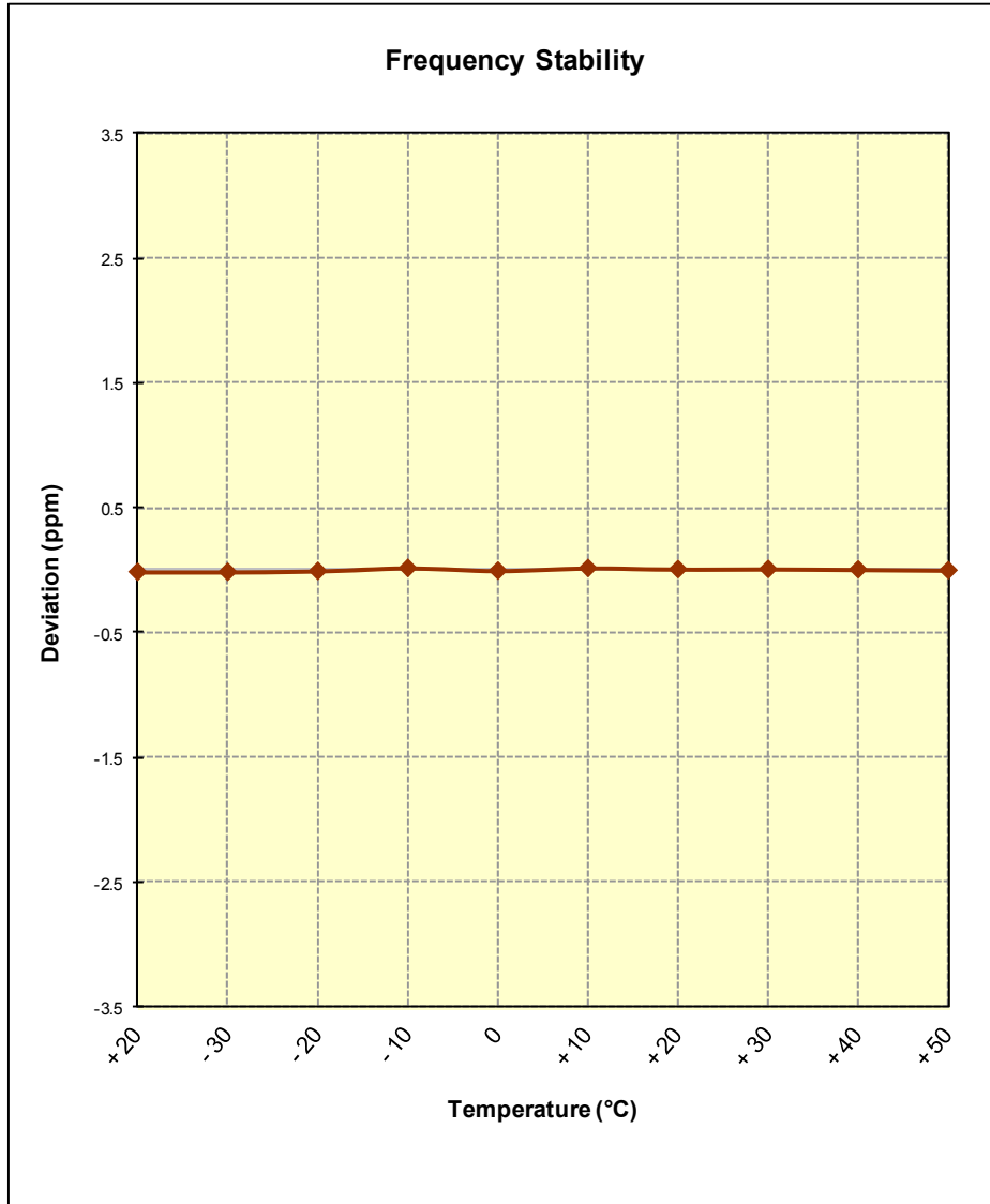
Figure 6-10. Frequency Stability Graph (PCS WCDMA Mode – Ch. 9400)
