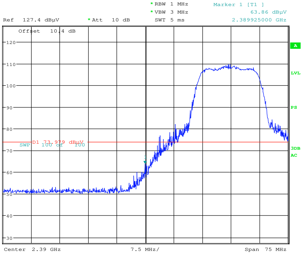
Plot 6-60. Radiated Restricted Lower Band Edge Measurement (Peak)
