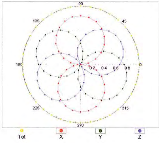
f=600 MHz,TEM
