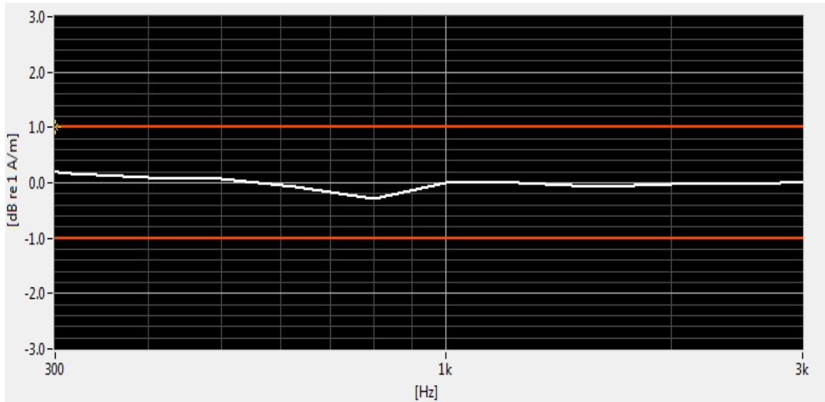
Figure 7-3 Helmholtz Coil Validation for Frequency Response
