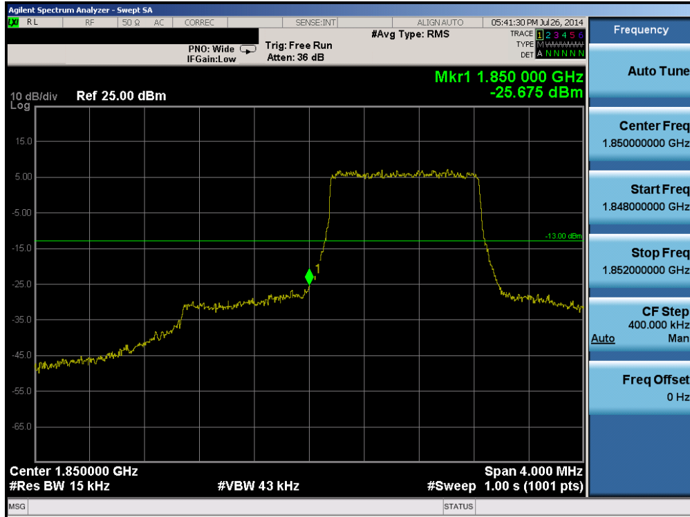
Plot 6-214. Lower Band Edge Plot (Band 2 – 1.4MHz QPSK – RB Size 6)
