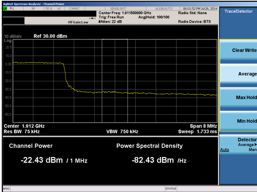
Plot 6-229. Upper Extended Band Edge Plot (Band 2 – 10.0MHz QPSK – RB Size 50)
