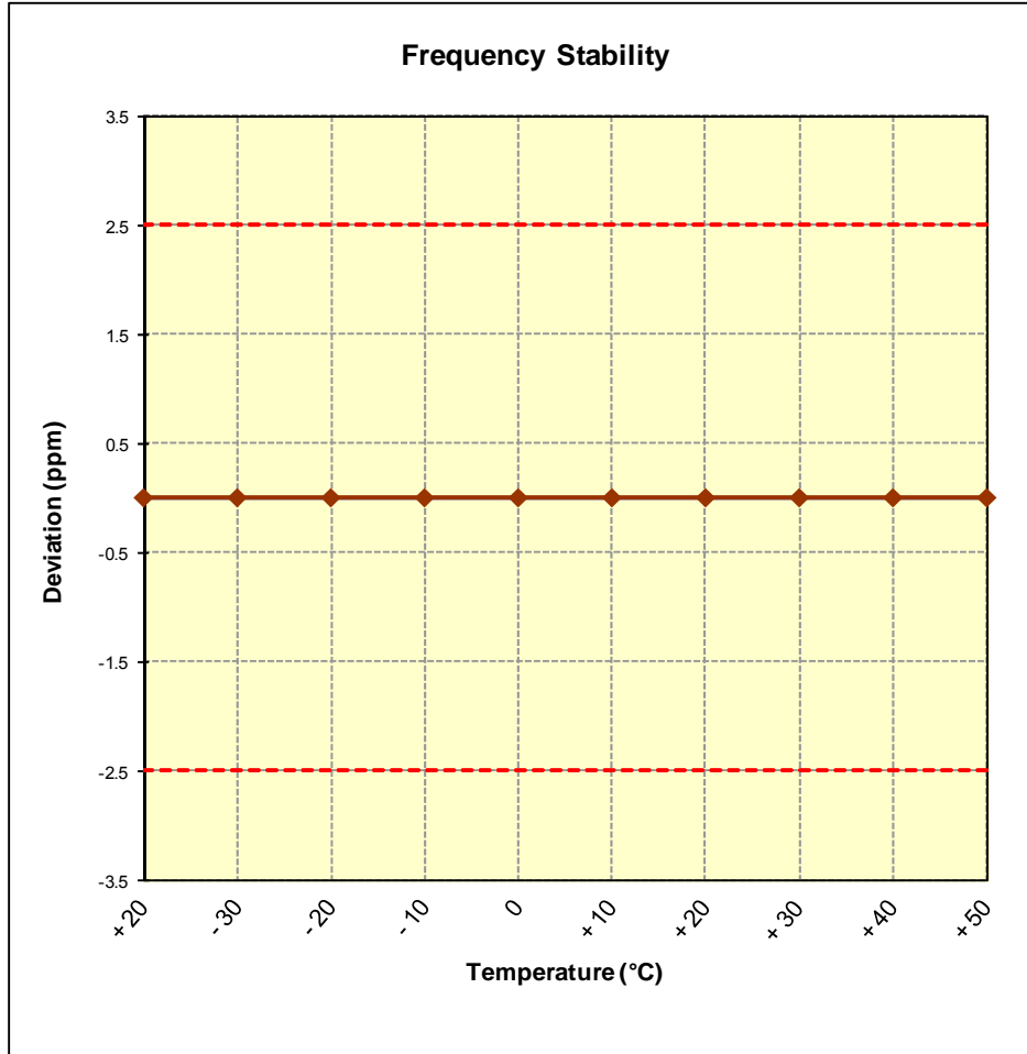
Figure 6-8. Frequency Stability Graph (Band 17)
