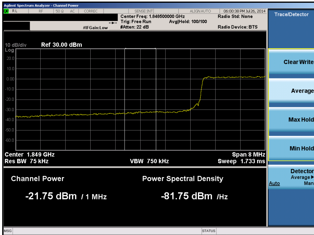
Plot 6-227. Lower Extended Band Edge Plot (Band 2 – 10.0MHz QPSK – RB Size 50)
