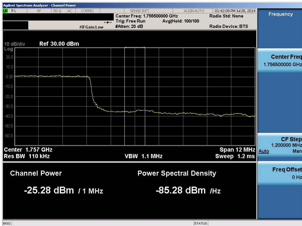
Plot 6-209. Upper Extended Band Edge Plot (Band 4 – 15.0MHz QPSK – RB Size 75)
