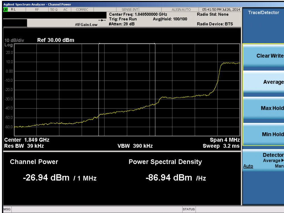
Plot 6-215. Lower Extended Band Edge Plot (Band 2 – 1.4MHz QPSK – RB Size 6)
