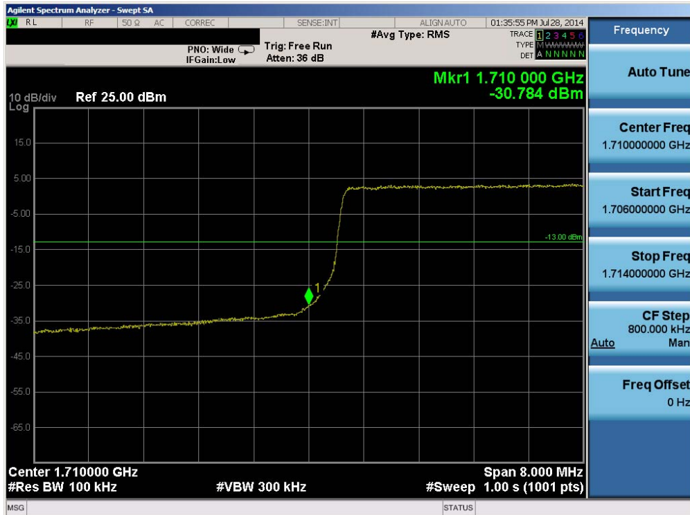
Plot 6-202. Lower Band Edge Plot (Band 4 – 10.0MHz QPSK – RB Size 50)
