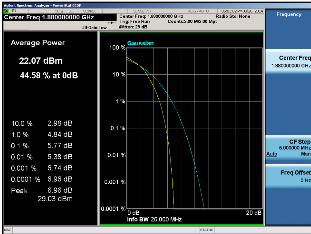
Plot 6-247. PAR Plot (Band 2 – 15.0MHz 16-QAM – RB Size 75)
