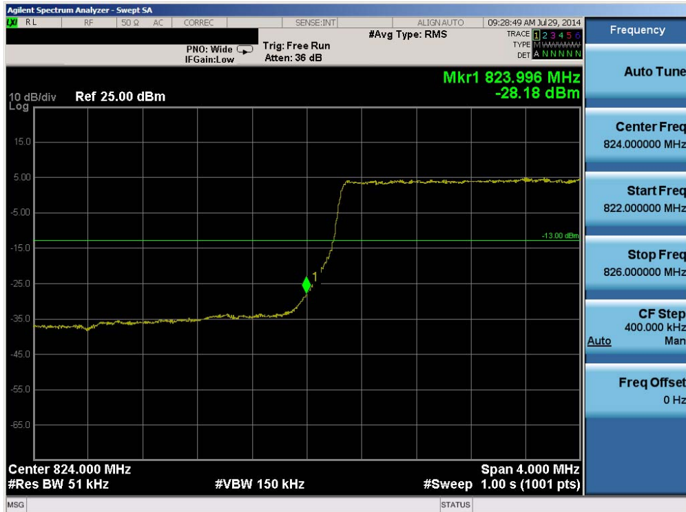
Plot 6-184. Lower Band Edge Plot (Band 5 – 5.0MHz QPSK – RB Size 25)
