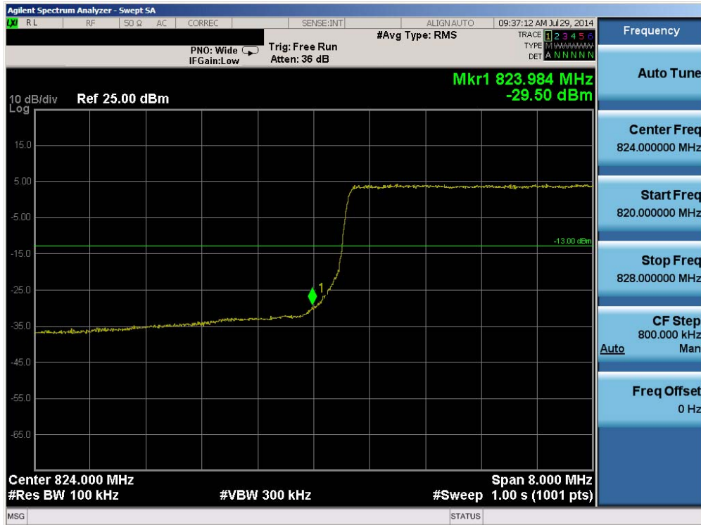
Plot 6-188. Lower Band Edge Plot (Band 5 – 10.0MHz QPSK – RB Size 50)
