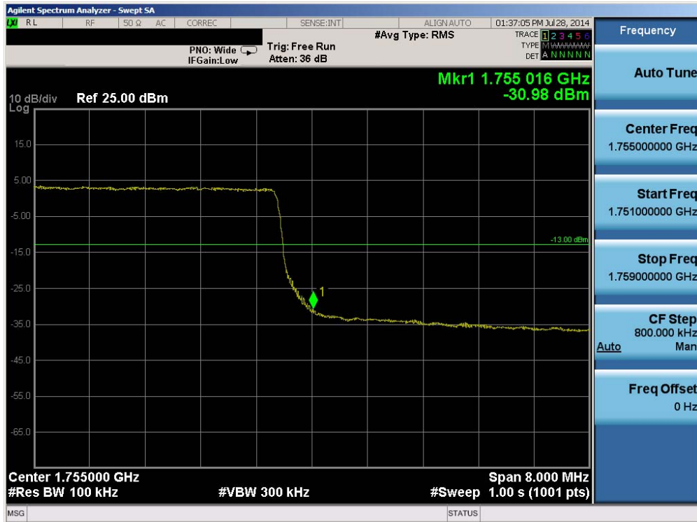
Plot 6-204. Upper Band Edge Plot (Band 4 – 10.0MHz QPSK – RB Size 50)
