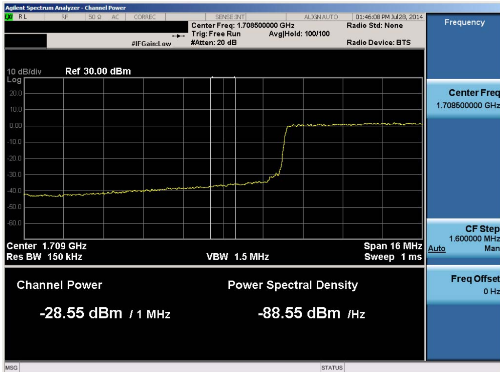
Plot 6-211. Lower Extended Band Edge Plot (Band 4 – 20.0MHz QPSK – RB Size 100)
