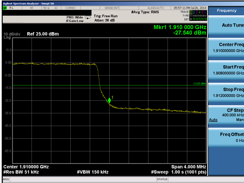
Plot 6-224. Upper Band Edge Plot (Band 2 – 5.0MHz QPSK – RB Size 25)
