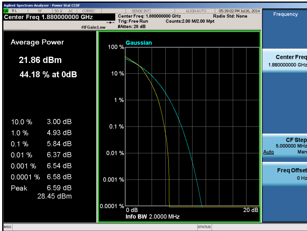
Plot 6-239. PAR Plot (Band 2 – 1.4MHz 16-QAM – RB Size 6)
