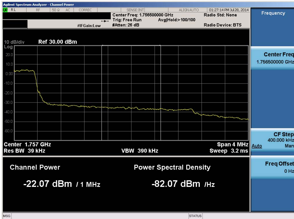
Plot 6-197. Upper Extended Band Edge Plot (Band 4 – 3.0MHz QPSK – RB Size 15)
