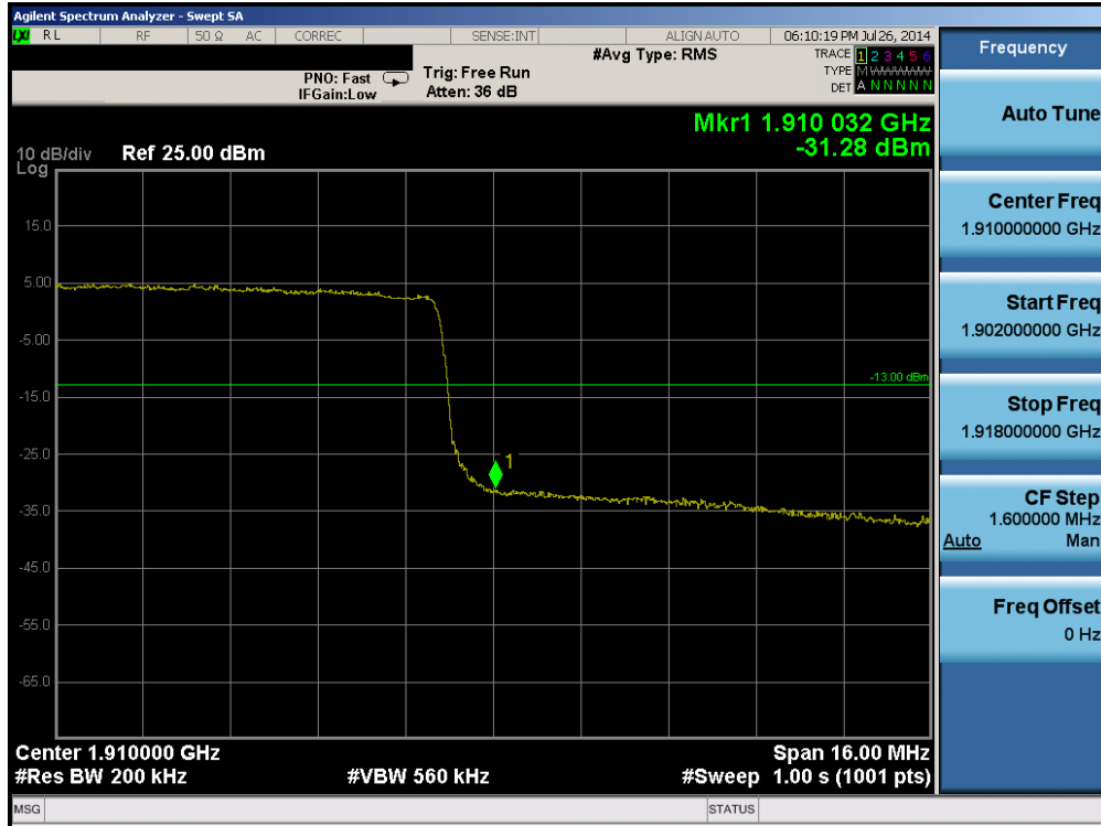
Plot 6-236. Upper Band Edge Plot (Band 2 - 20.0MHz QPSK - RB Size 100)
