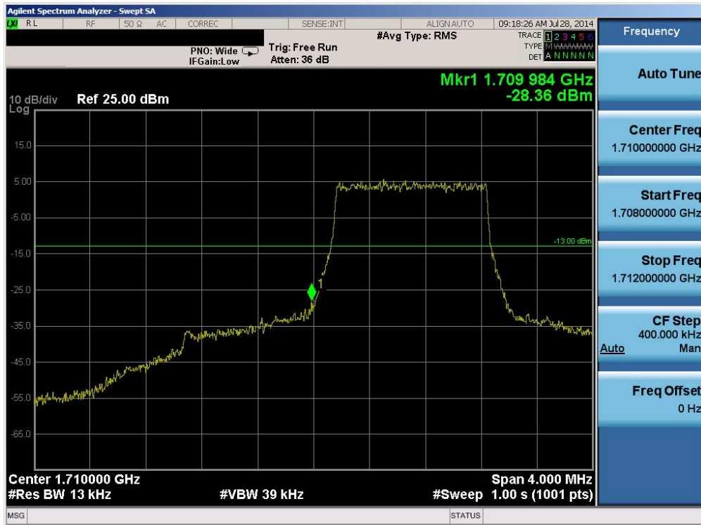
Plot 6-190. Lower Band Edge Plot (Band 4 – 1.4MHz QPSK – RB Size 6)
