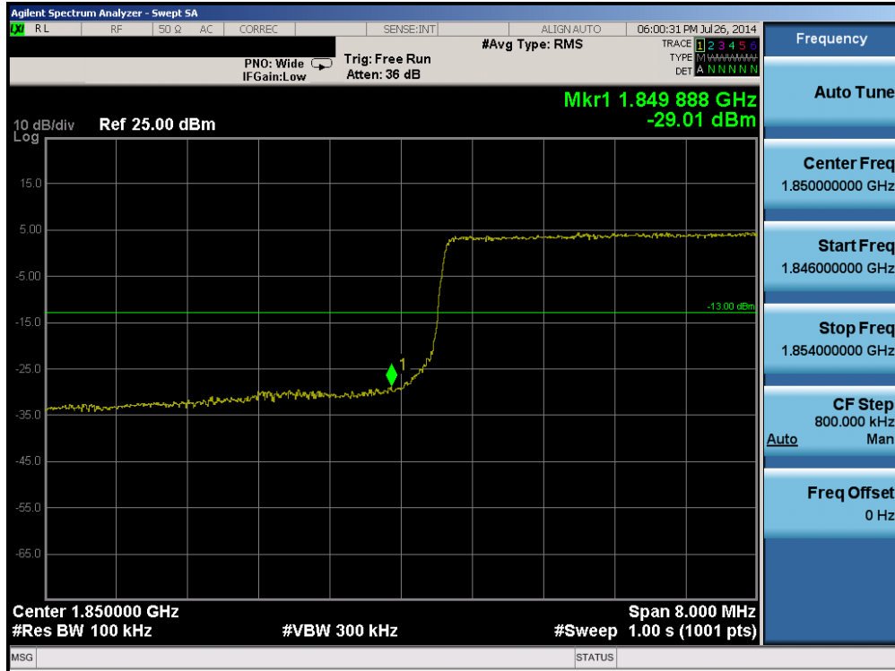
Plot 6-226. Lower Band Edge Plot (Band 2 – 10.0MHz QPSK – RB Size 50)
