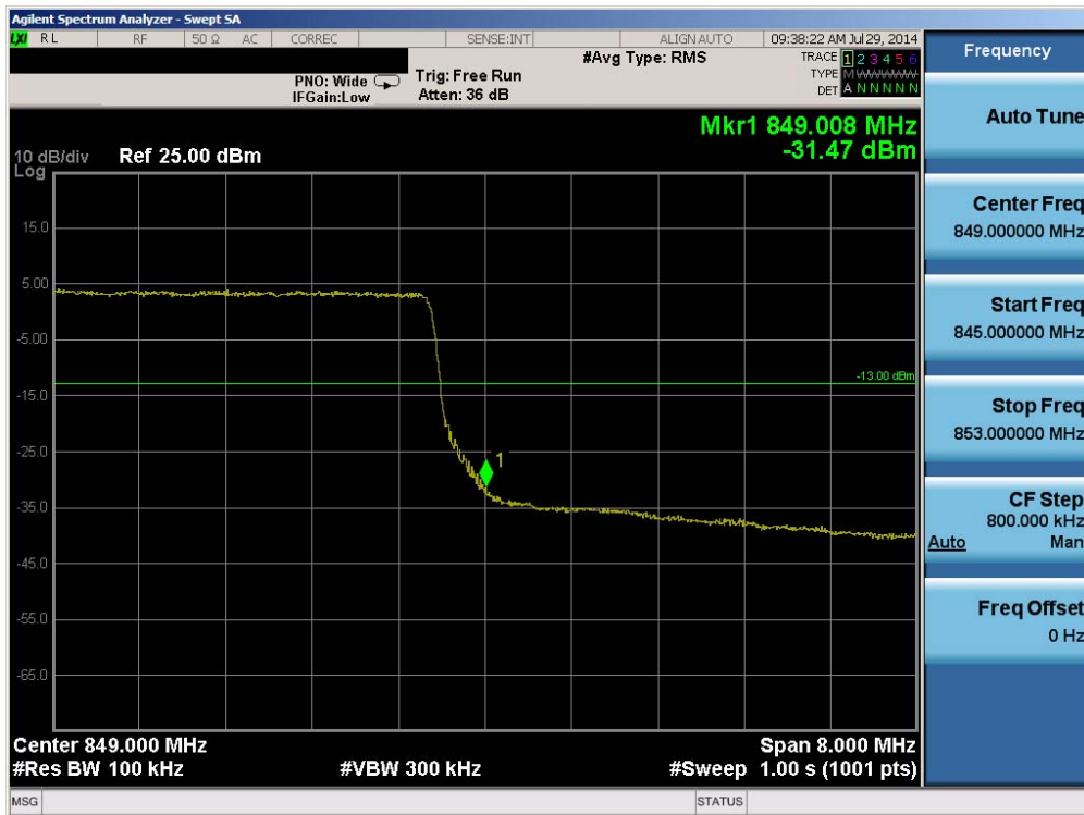
Plot 6-189. Upper Band Edge Plot (Band 5 – 10.0MHz QPSK – RB Size 50)
