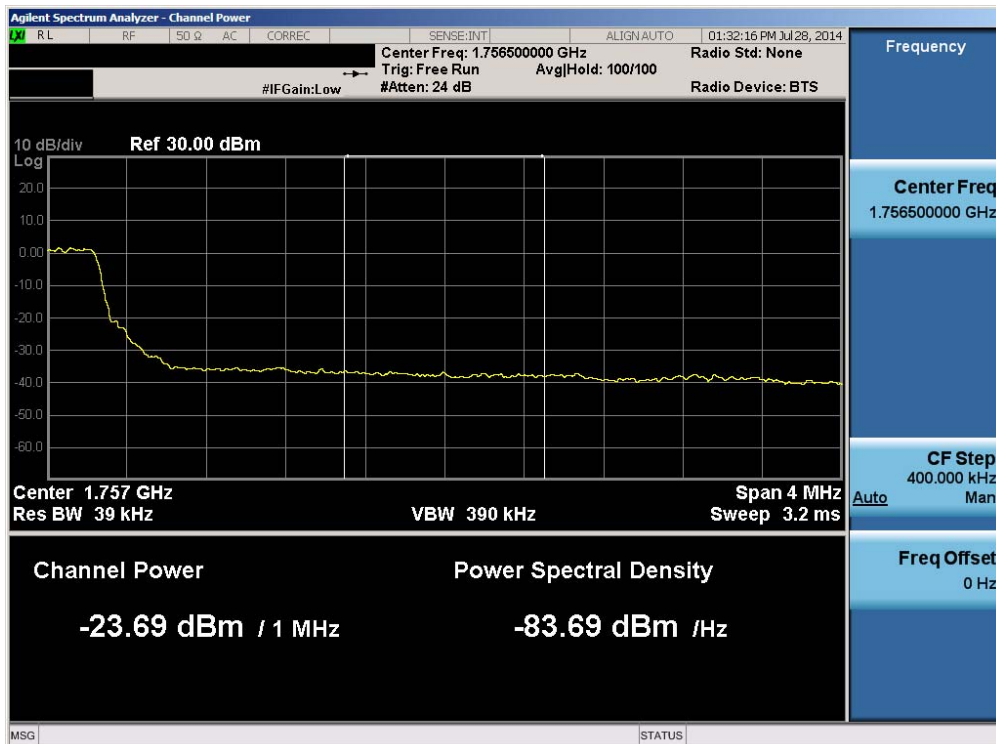
Plot 6-201. Upper Extended Band Edge Plot (Band 4 – 5.0MHz QPSK – RB Size 25)
