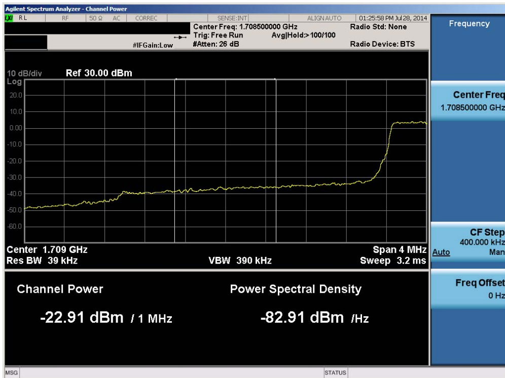
Plot 6-195. Lower Extended Band Edge Plot (Band 4 – 3.0MHz QPSK – RB Size 15)
