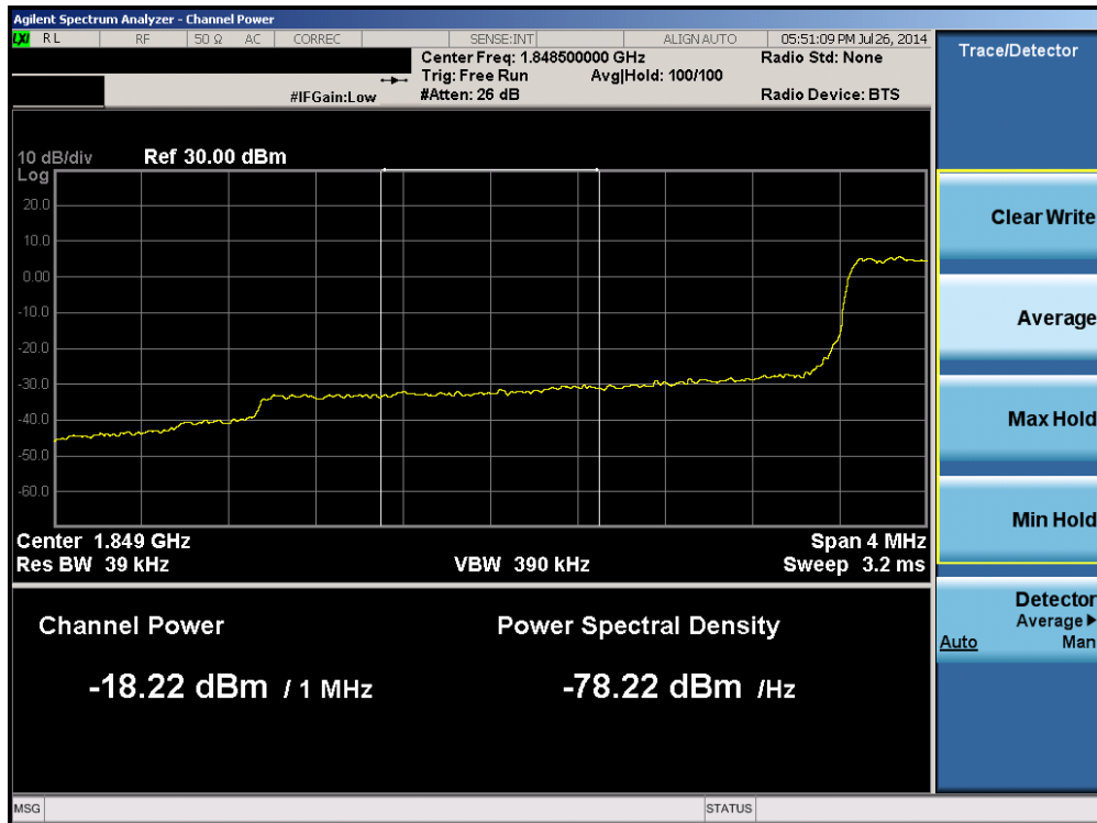
Plot 6-219. Lower Extended Band Edge Plot (Band 2 – 3.0MHz QPSK – RB Size 15)
