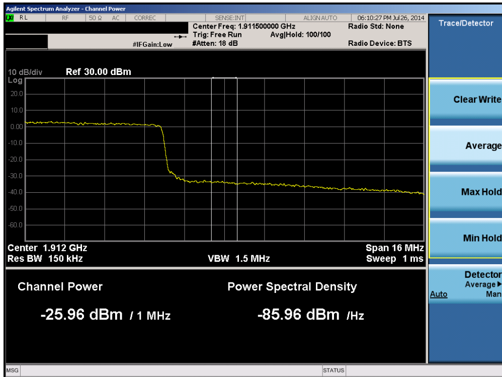
Plot 6-237. Upper Extended Band Edge Plot (Band 2 - 20.0MHz QPSK - RB Size 100)
