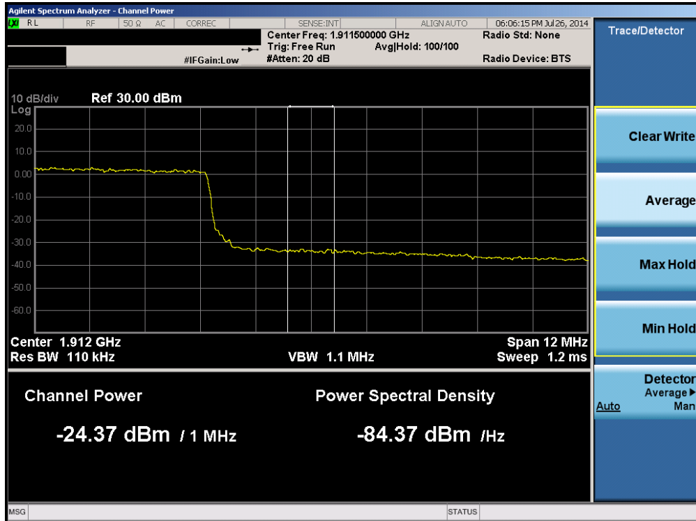
Plot 6-233. Upper Extended Band Edge Plot (Band 2 – 15.0MHz QPSK – RB Size 75)
