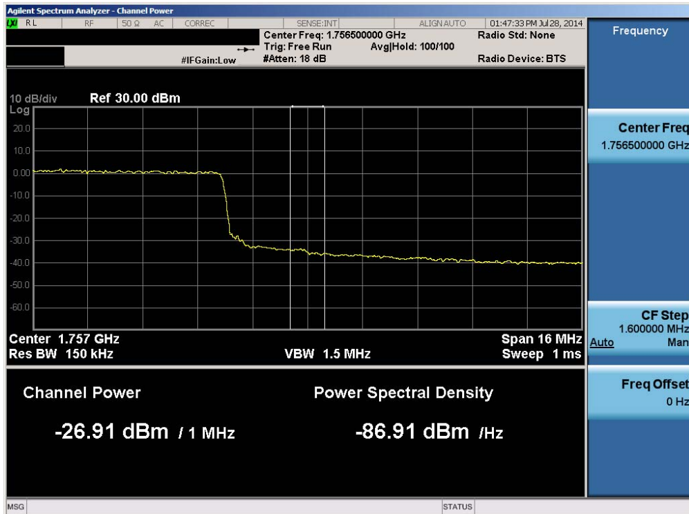
Plot 6-213. Upper Extended Band Edge Plot (Band 4 – 20.0MHz QPSK – RB Size 100)
