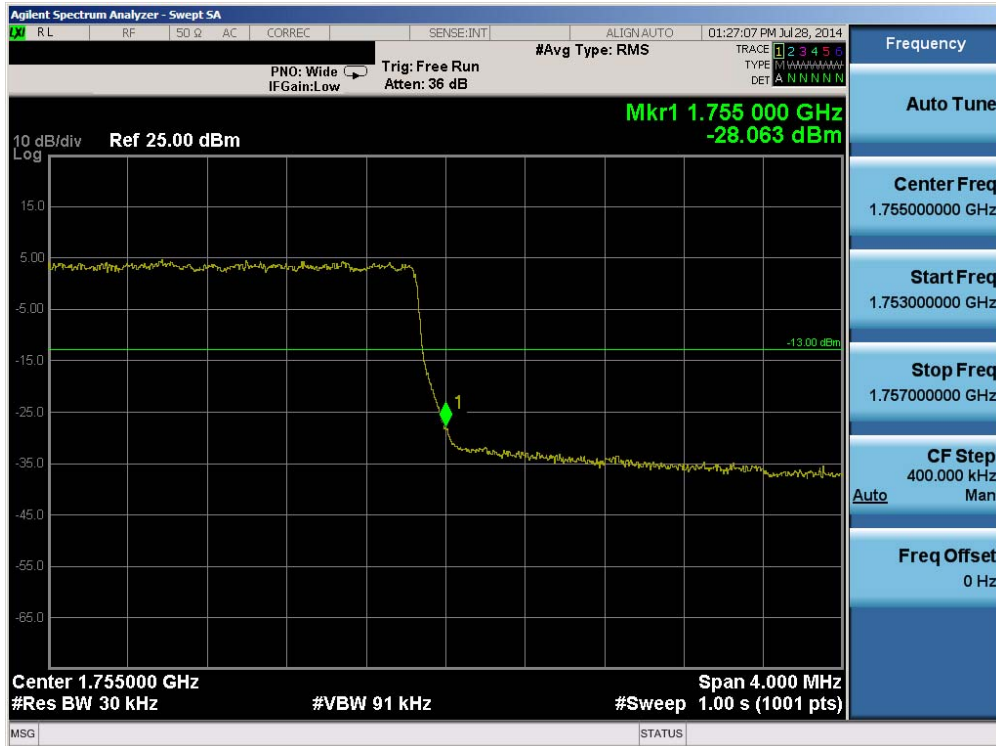
Plot 6-196. Upper Band Edge Plot (Band 4 – 3.0MHz QPSK – RB Size 15)
