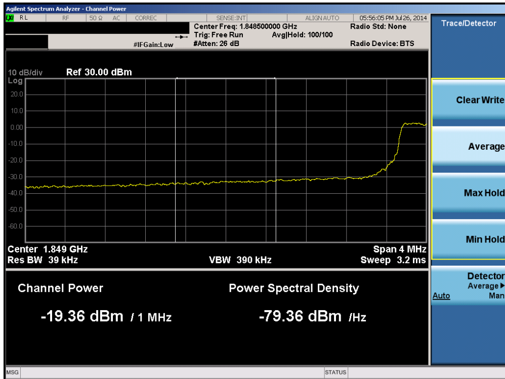
Plot 6-223. Lower Extended Band Edge Plot (Band 2 – 5.0MHz QPSK – RB Size 25)
