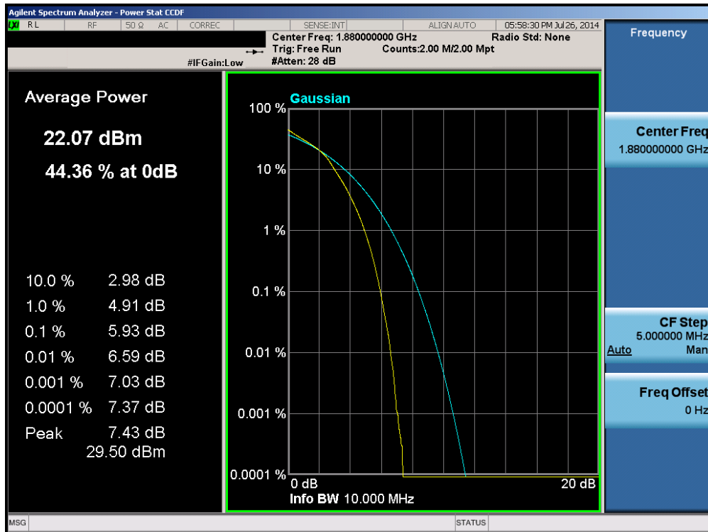
Plot 6-245. PAR Plot (Band 2 – 10.0MHz 16-QAM – RB Size 50)
