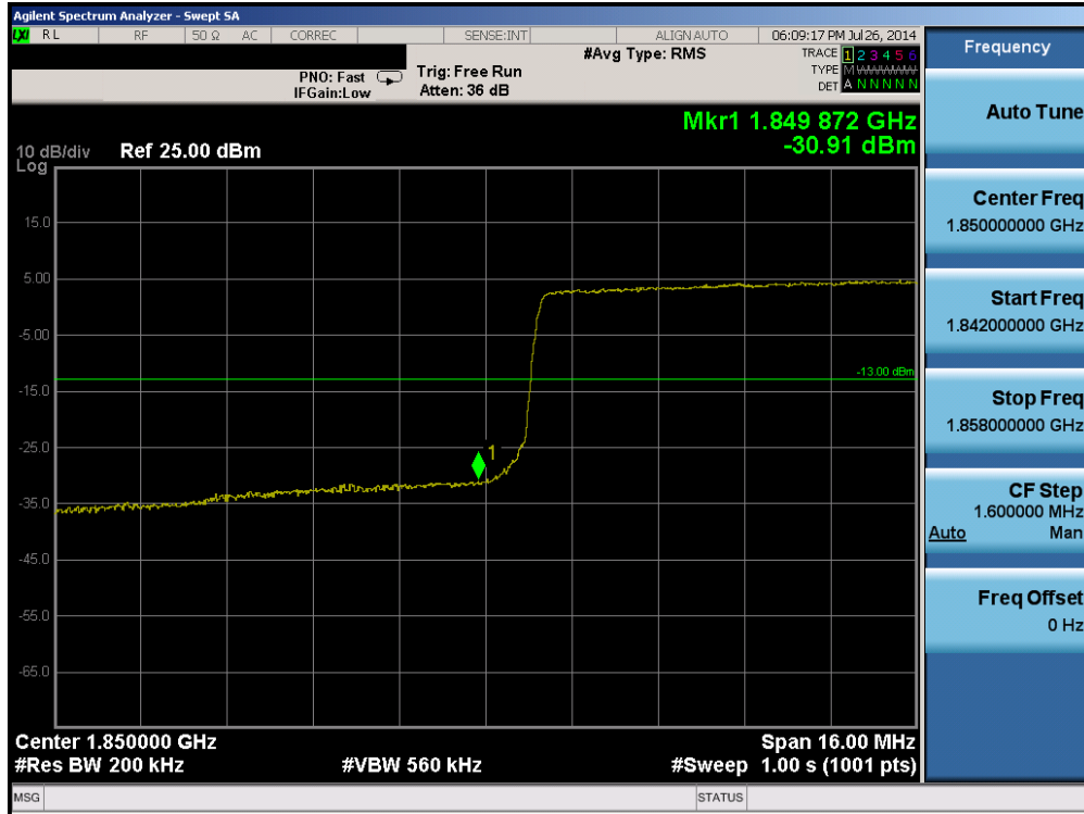
Plot 6-234. Lower Band Edge Plot (Band 2 – 20.0MHz QPSK – RB Size 100)
