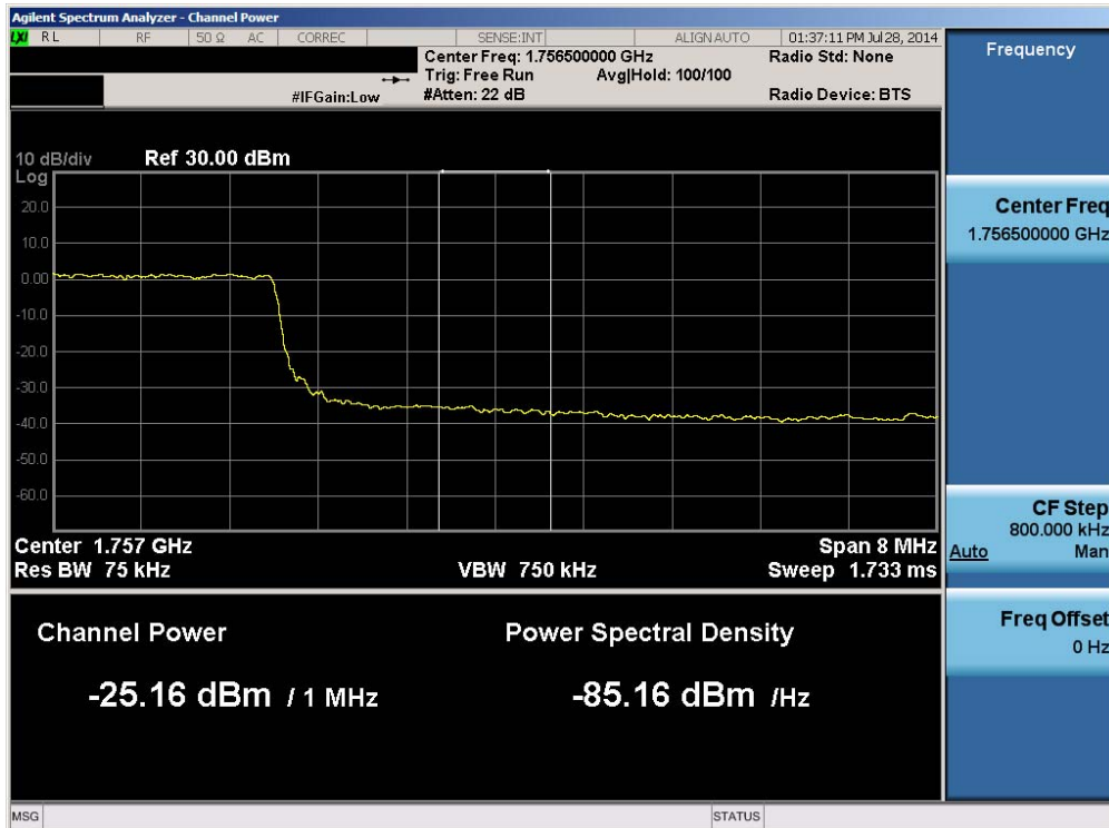
Plot 6-205. Upper Extended Band Edge Plot (Band 4 – 10.0MHz QPSK – RB Size 50)
