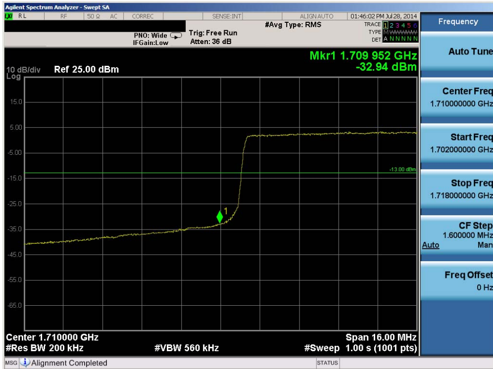
Plot 6-210. Lower Band Edge Plot (Band 4 – 20.0MHz QPSK – RB Size 100)
