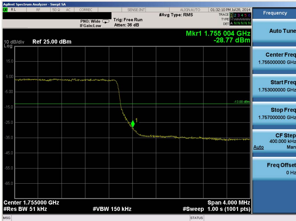
Plot 6-200. Upper Band Edge Plot (Band 4 – 5.0MHz QPSK – RB Size 25)
