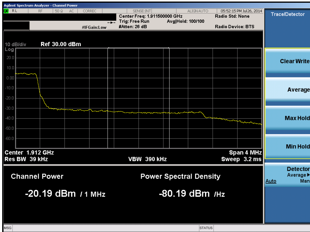
Plot 6-221. Upper Extended Band Edge Plot (Band 2 – 3.0MHz QPSK – RB Size 15)
