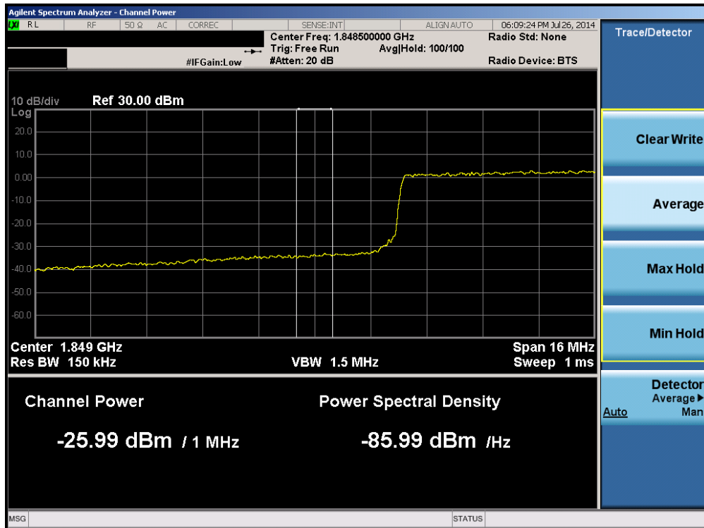
Plot 6-235. Lower Extended Band Edge Plot (Band 2 – 20.0MHz QPSK – RB Size 100)
