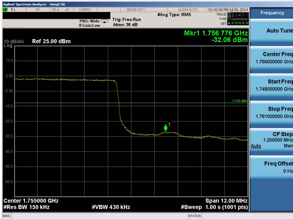
Plot 6-208. Upper Band Edge Plot (Band 4 – 15.0MHz QPSK – RB Size 75)
