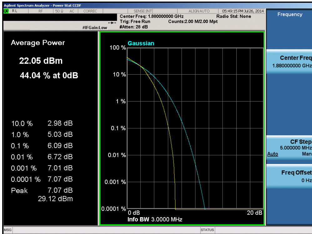
Plot 6-241. PAR Plot (Band 2 – 3.0MHz 16-QAM – RB Size 15)
