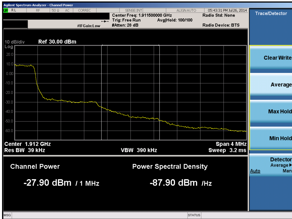
Plot 6-217. Upper Extended Band Edge Plot (Band 2 – 1.4MHz QPSK – RB Size 6)
