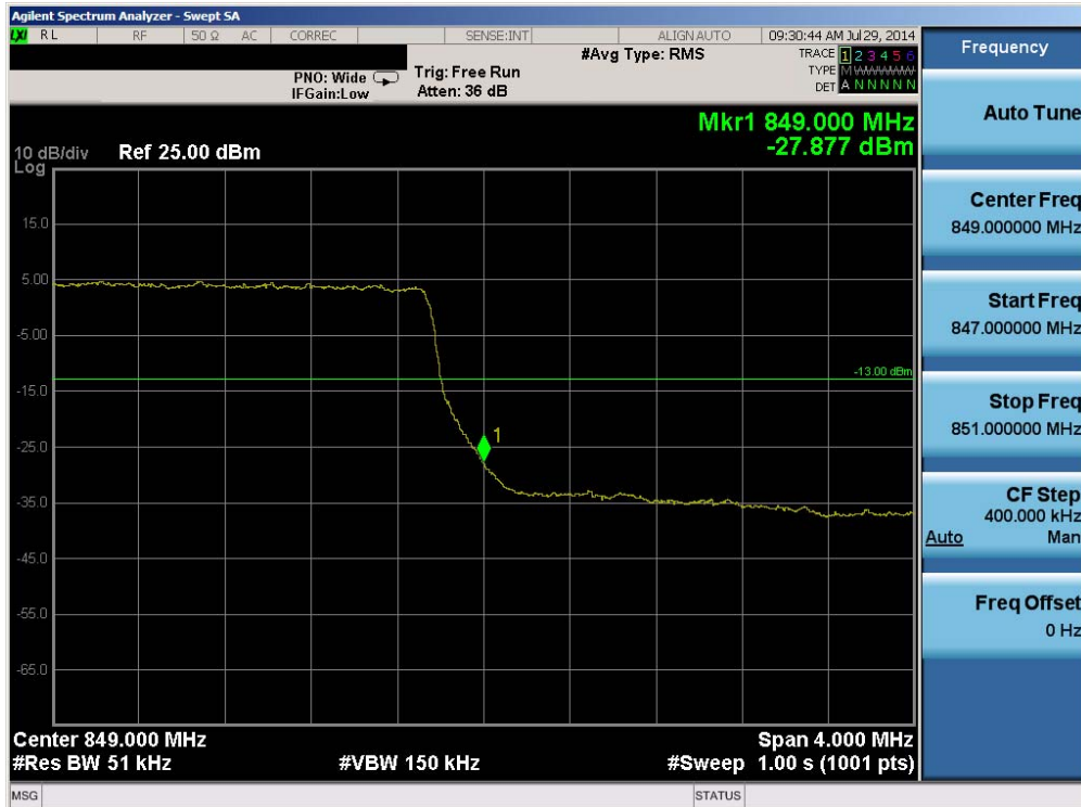
Plot 6-186. Upper Band Edge Plot (Band 5 – 5.0MHz QPSK – RB Size 25)
