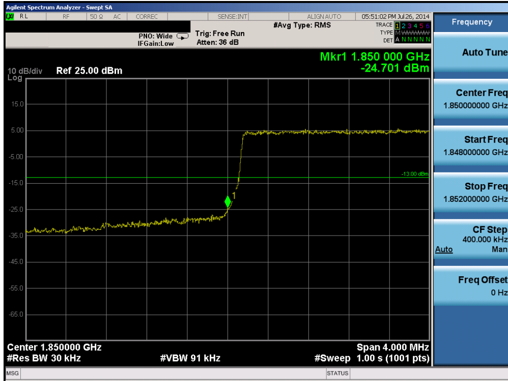
Plot 6-218. Lower Band Edge Plot (Band 2 – 3.0MHz QPSK – RB Size 15)
