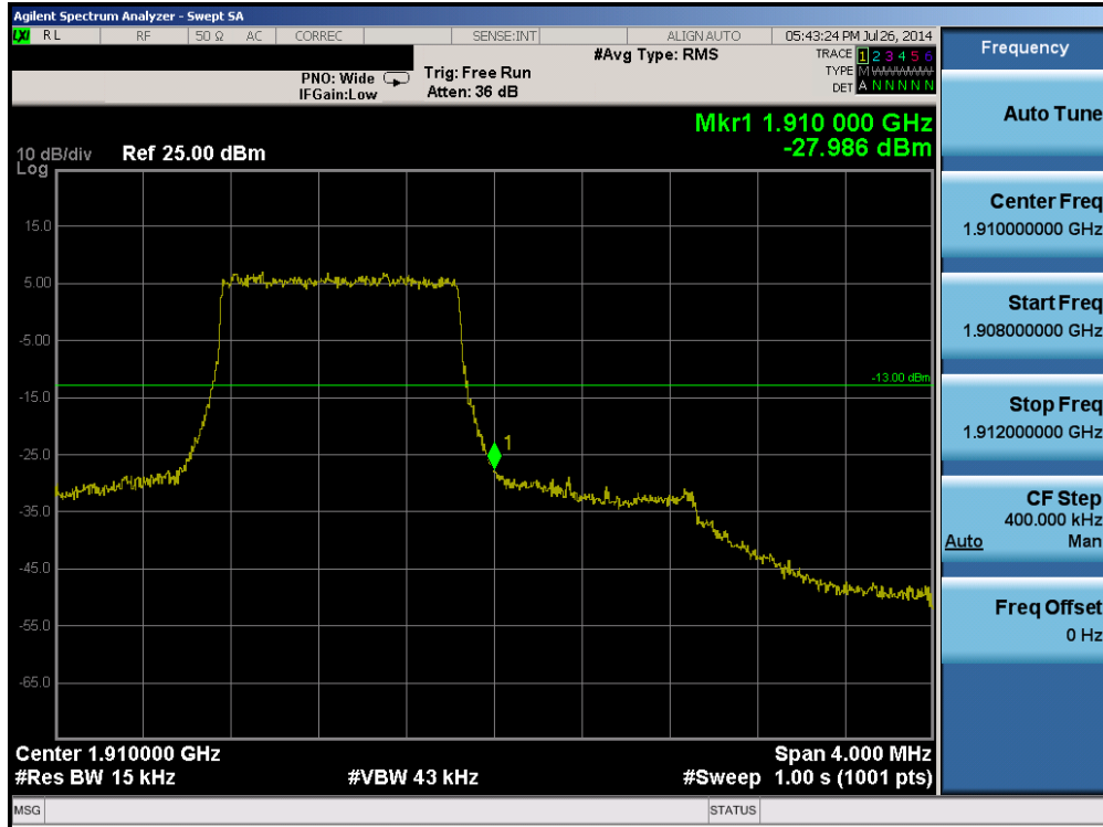
Plot 6-216. Upper Band Edge Plot (Band 2 – 1.4MHz QPSK – RB Size 6)
