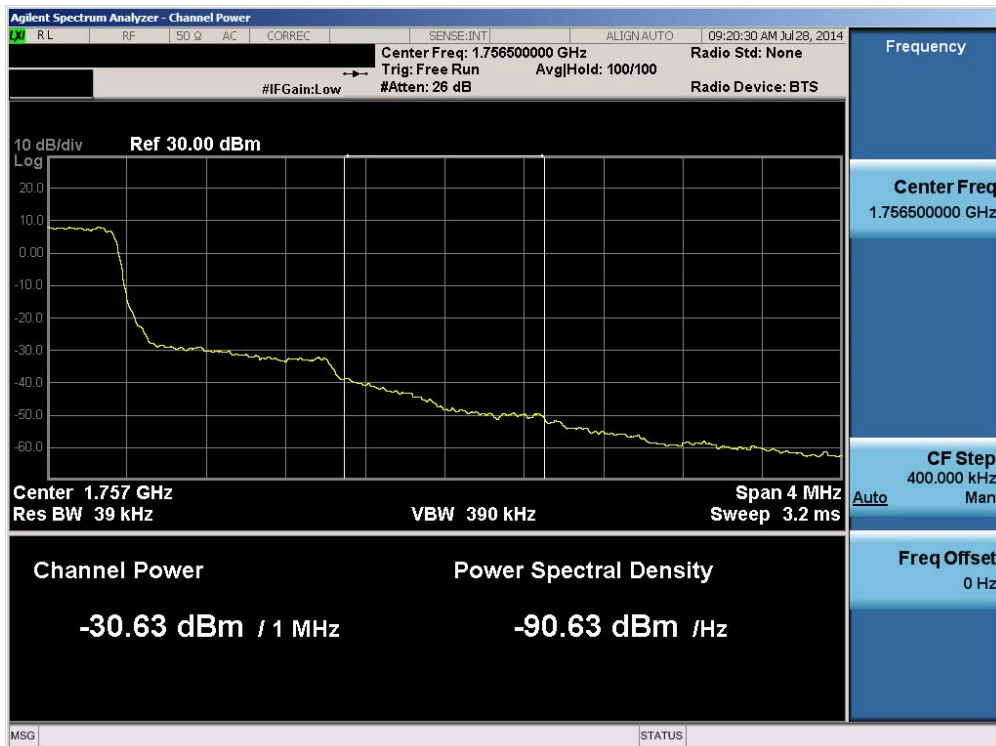
Plot 6-193. Upper Extended Band Edge Plot (Band 4 – 1.4MHz QPSK – RB Size 6)
