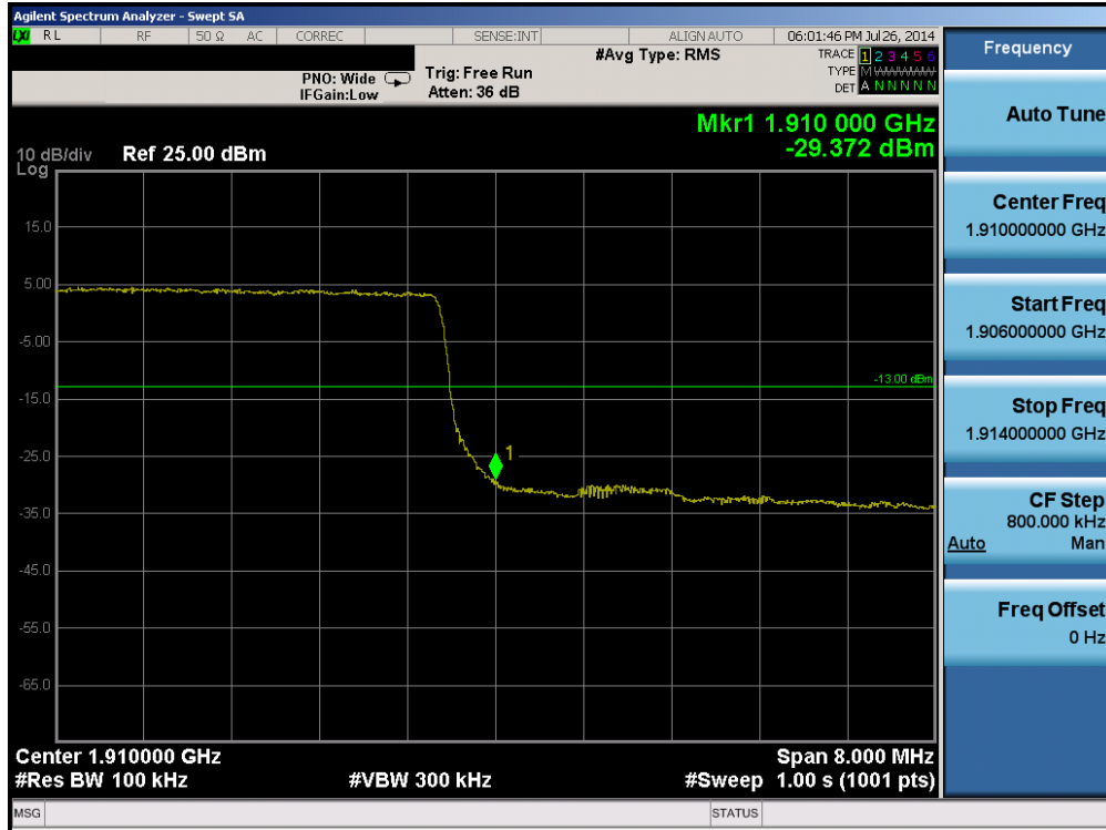
Plot 6-228. Upper Band Edge Plot (Band 2 – 10.0MHz QPSK – RB Size 50)
