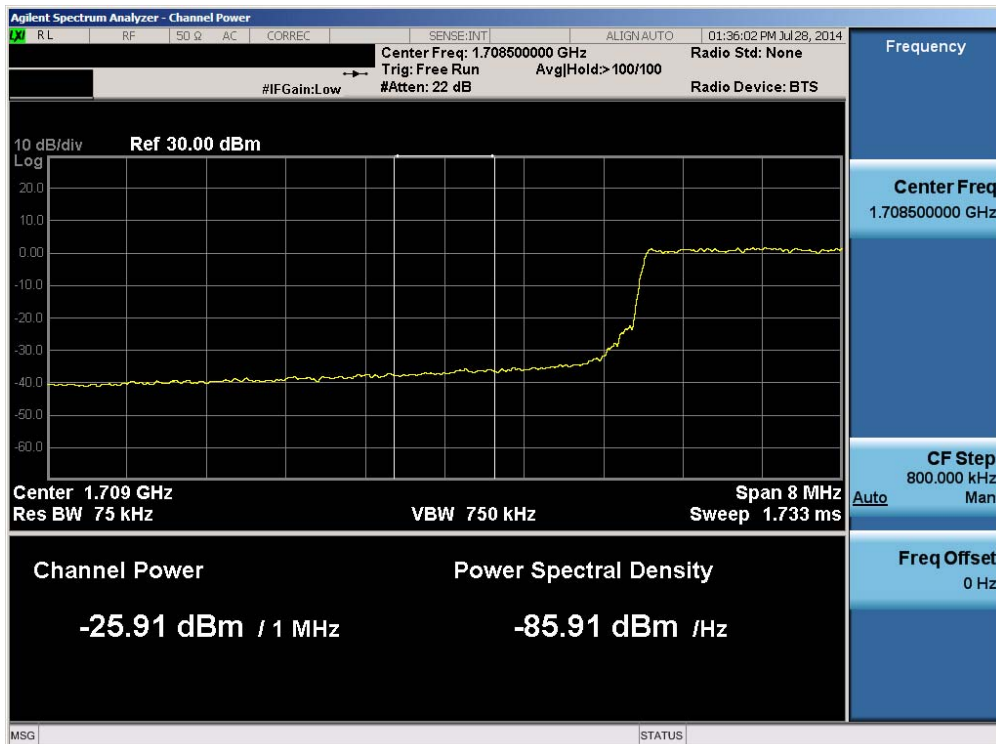
Plot 6-203. Lower Extended Band Edge Plot (Band 4 – 10.0MHz QPSK – RB Size 50)
