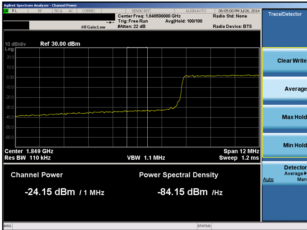
Plot 6-231. Lower Extended Band Edge Plot (Band 2 – 15.0MHz QPSK – RB Size 75)
