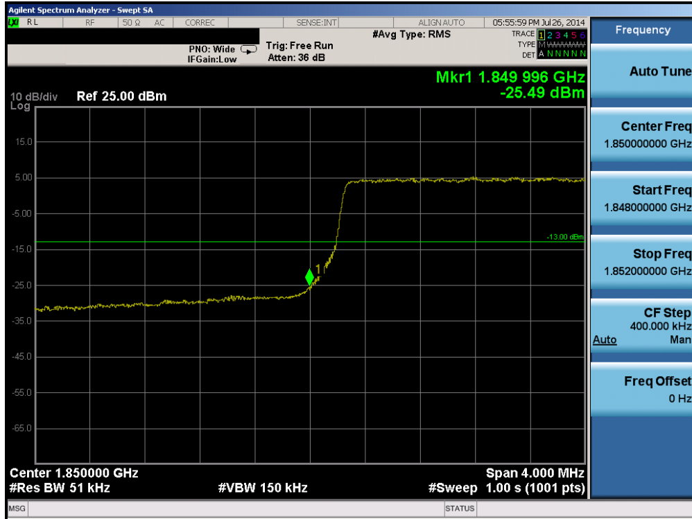
Plot 6-222. Lower Band Edge Plot (Band 2 – 5.0MHz QPSK – RB Size 25)
