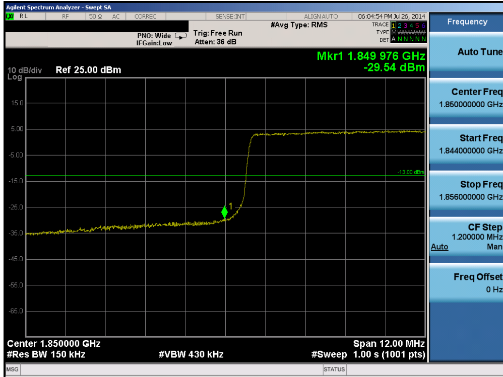
Plot 6-230. Lower Band Edge Plot (Band 2 – 15.0MHz QPSK – RB Size 75)
