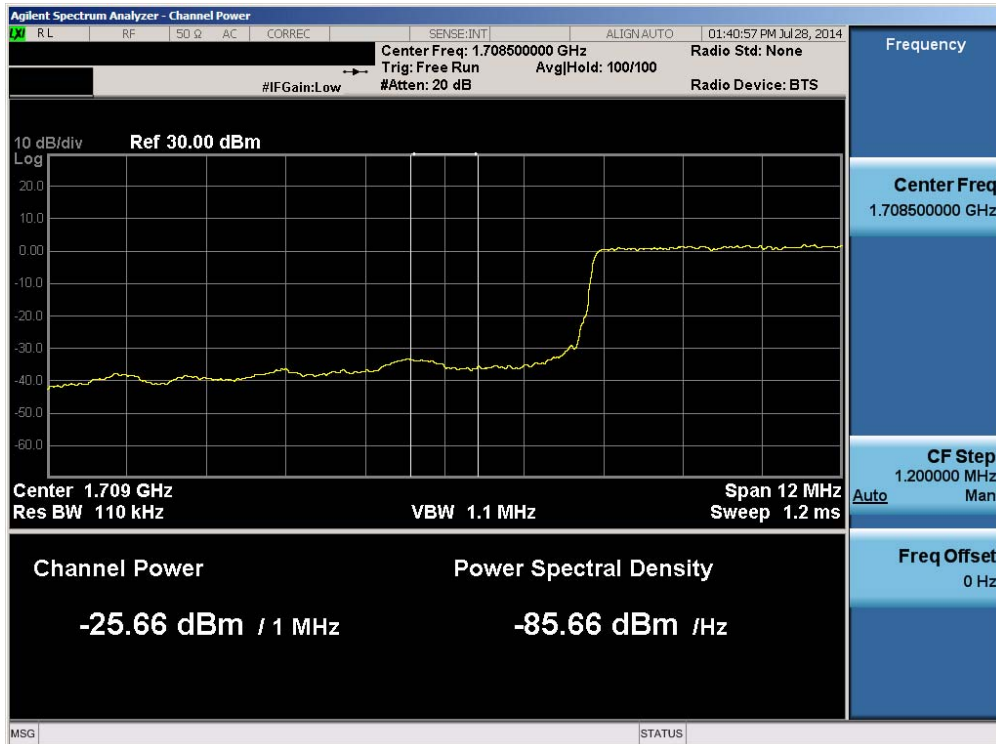
Plot 6-207. Lower Extended Band Edge Plot (Band 4 – 15.0MHz QPSK – RB Size 75)
