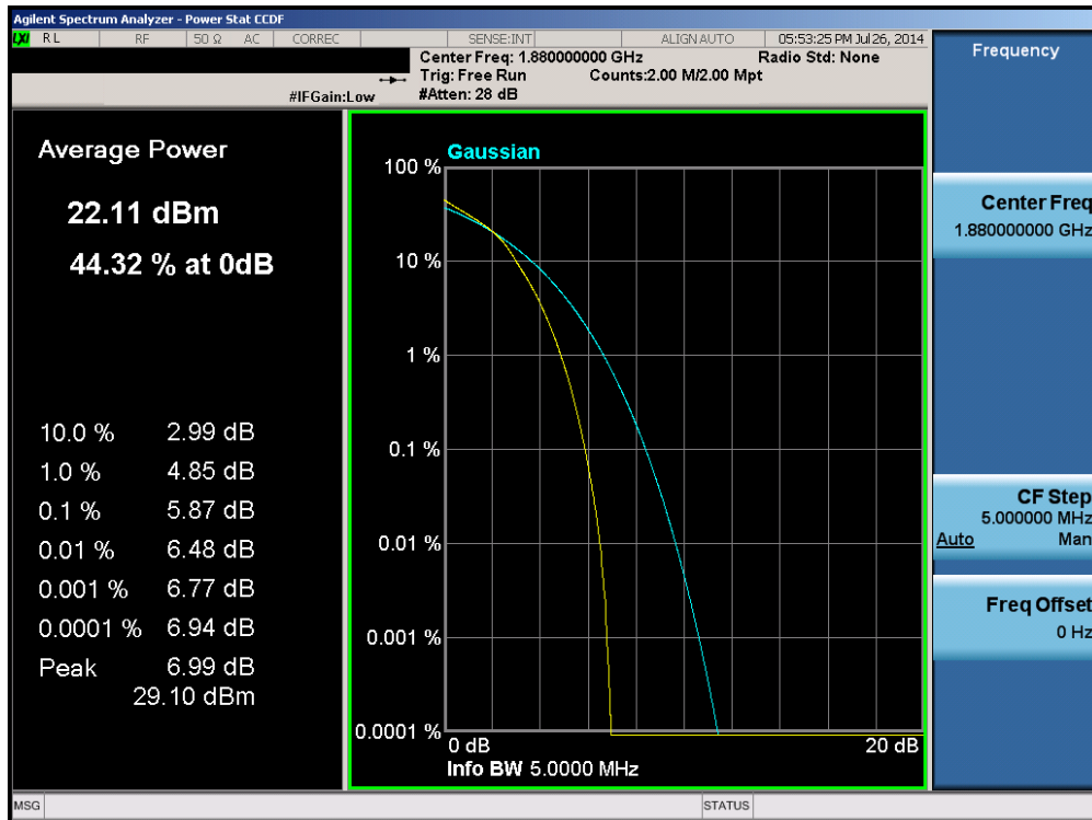
Plot 6-243. PAR Plot (Band 2 – 5.0MHz 16-QAM – RB Size 25)
