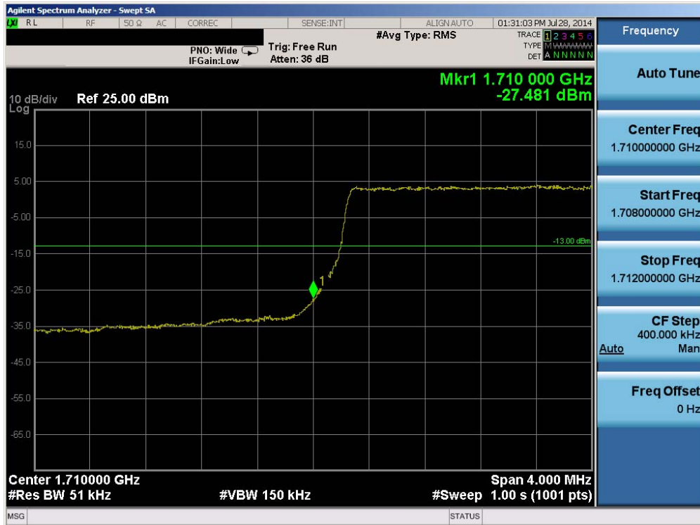
Plot 6-198. Lower Band Edge Plot (Band 4 – 5.0MHz QPSK – RB Size 25)
