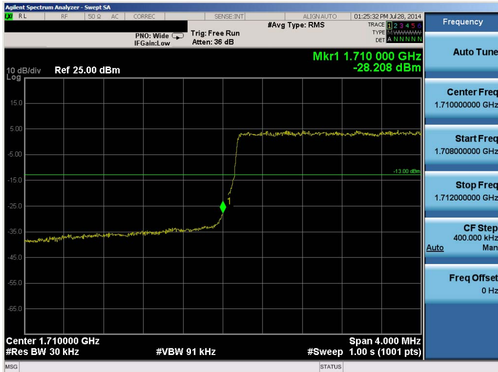
Plot 6-194. Lower Band Edge Plot (Band 4 – 3.0MHz QPSK – RB Size 15)
