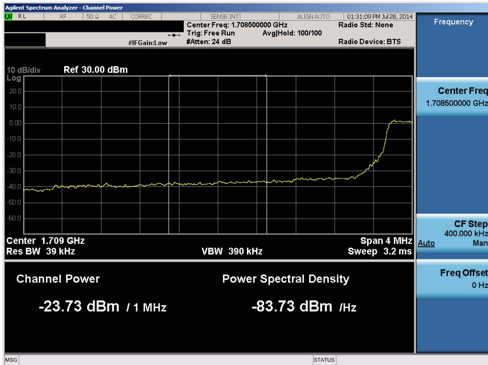
Plot 6-199. Lower Extended Band Edge Plot (Band 4 – 5.0MHz QPSK – RB Size 25)
