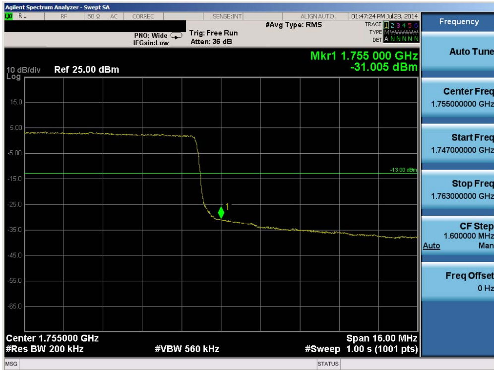
Plot 6-212. Upper Band Edge Plot (Band 4 – 20.0MHz QPSK – RB Size 100)
