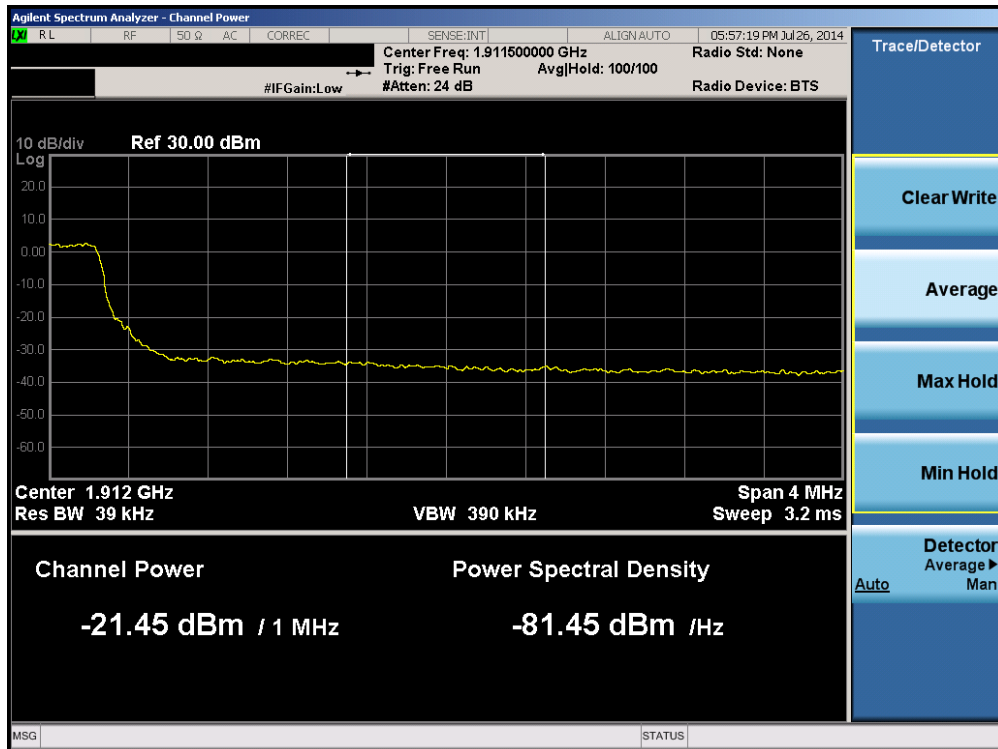
Plot 6-225. Upper Extended Band Edge Plot (Band 2 – 5.0MHz QPSK – RB Size 25)
