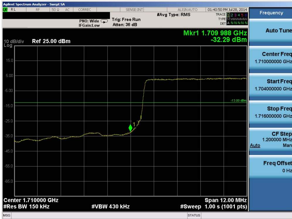
Plot 6-206. Lower Band Edge Plot (Band 4 – 15.0MHz QPSK – RB Size 75)
