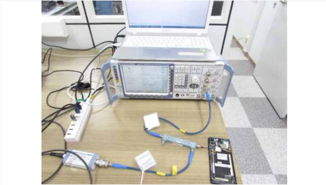
Test setup photo-1 (8-1(a) Legacy)
