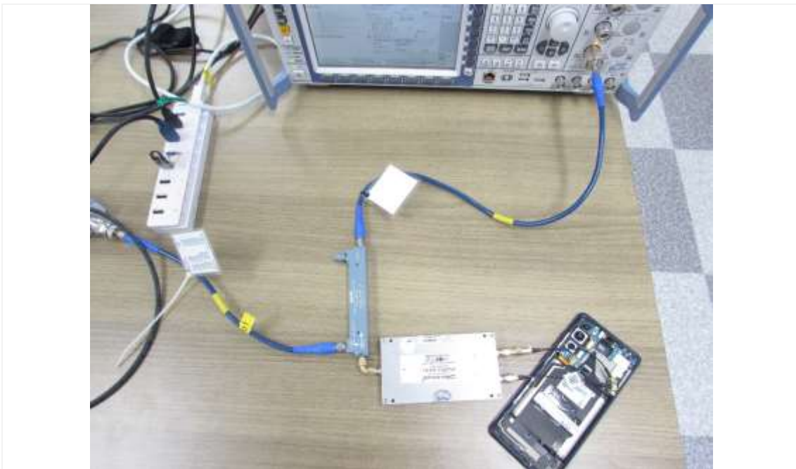
Test setup photo-2 (8-1(b) Legacy))
