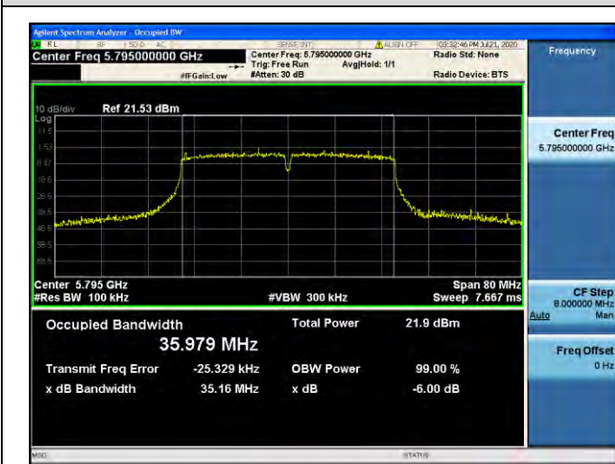
802.11ac(VHT40) (CH.159)
