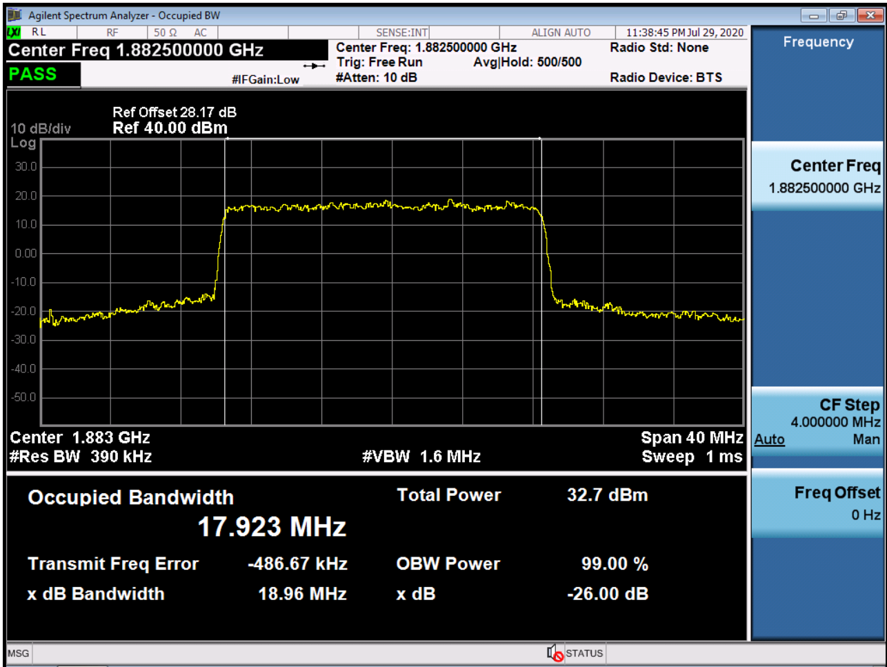
Sub6 n25(2). Occupied Bandwidth Plot (20M BW Ch.376500 QPSK RB 100_0)
