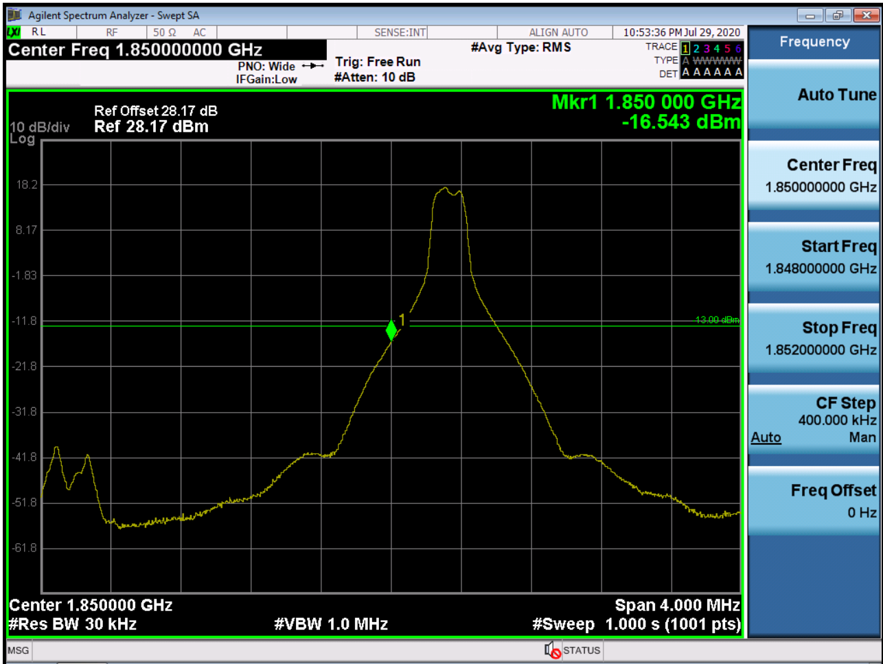
Sub6 n25(2). Lower Band Edge Plot (5M BW Ch.370500 BPSK_RB1_Offset 0)
