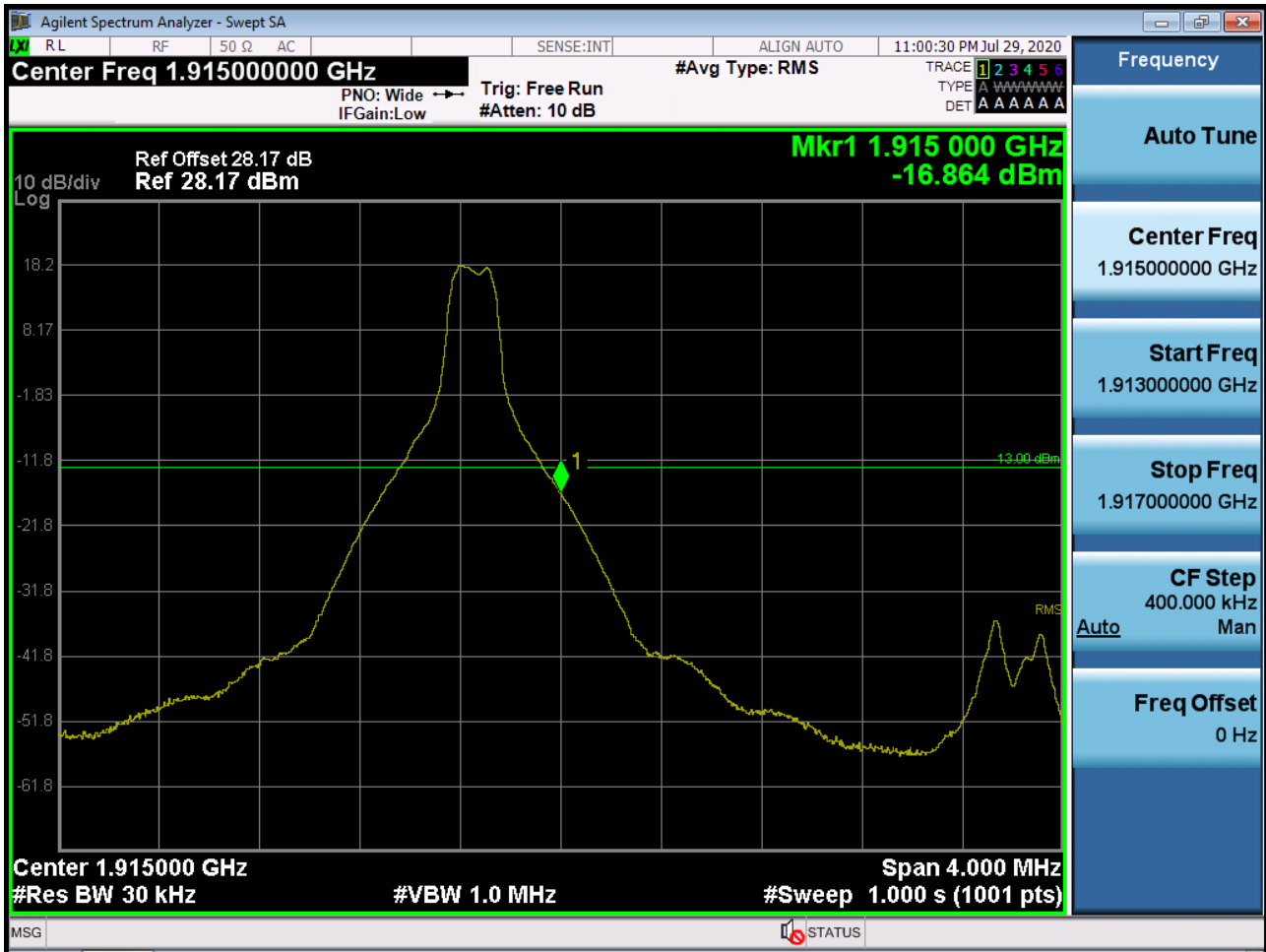
Sub6 n25(2). Upper Band Edge Plot (5M BW Ch.382500 BPSK_RB1_Offset 24)
