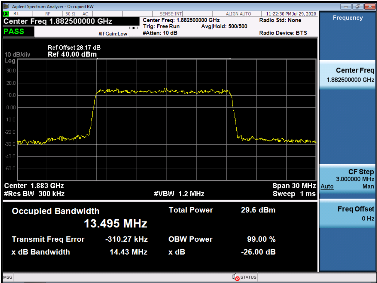
Sub6 n25(2). Occupied Bandwidth Plot (15M BW Ch.376500 256QAM RB 75_0)
