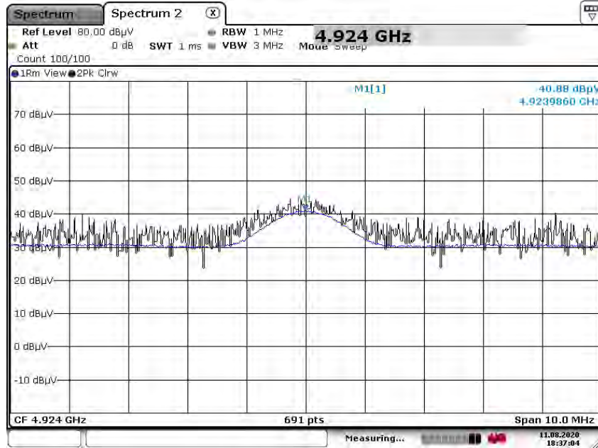
Radiated Spurious Emissions plot – Average Reading (Test case 1_ 2nd Harmonic)
