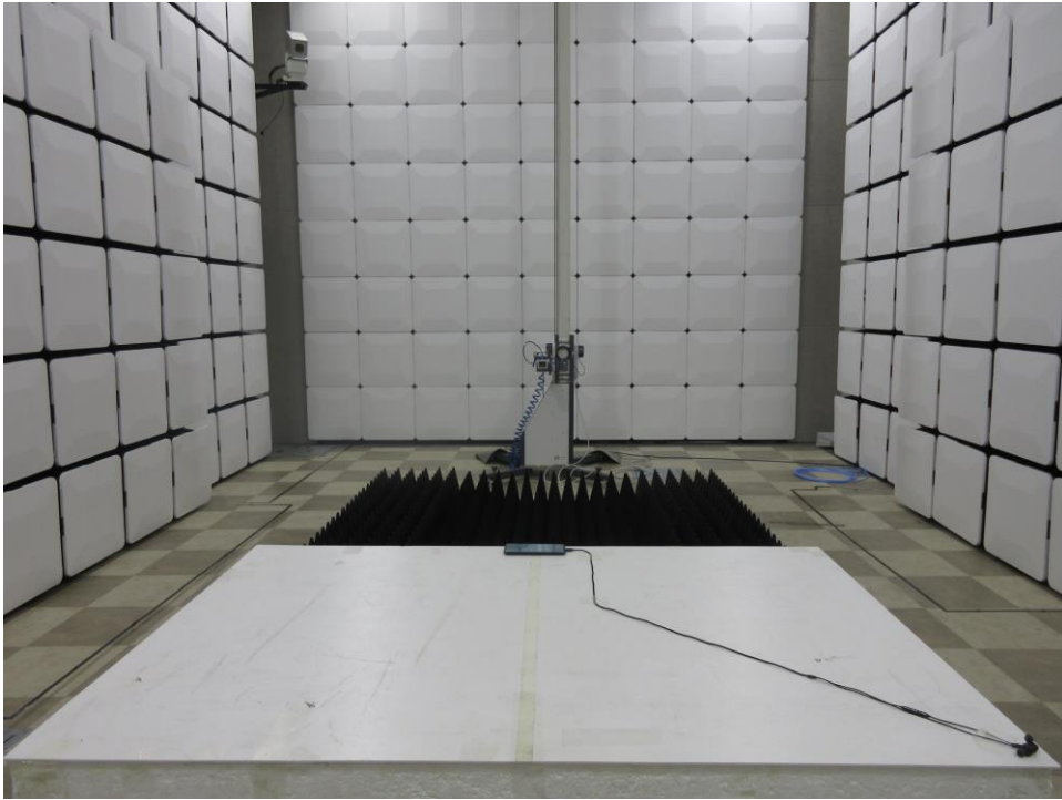
[EUT & Earphone]
