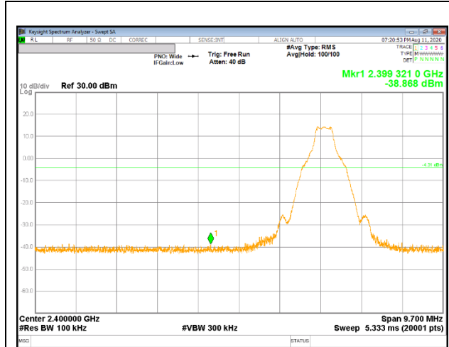
0 CHANNEL BANDEDGE
