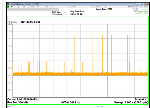
Antenna 1 / NUMBER OF PULSES IN 3.16 SECOND OBSERVATION PERIOD – DH5
