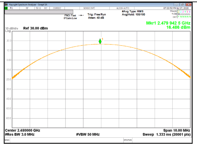
Antenna 2, 78 CHANNEL
