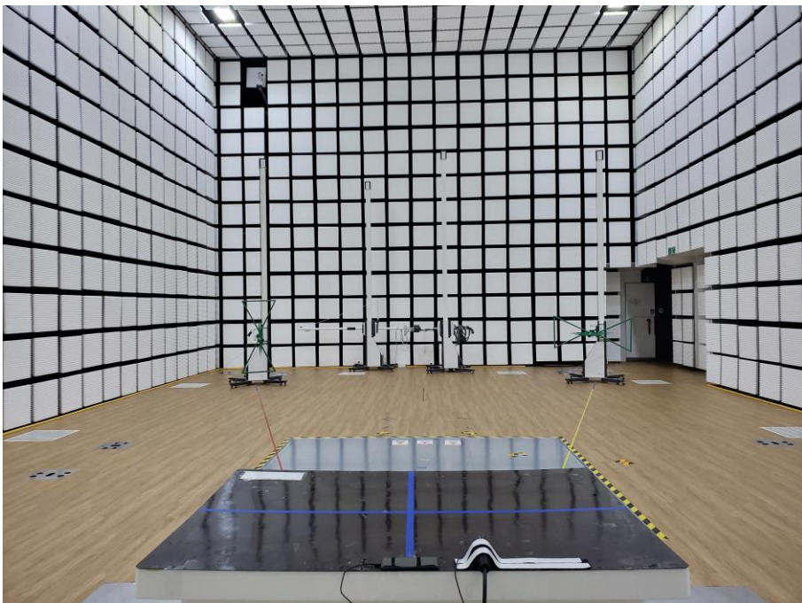
[ Mode 6 : Rear ]
