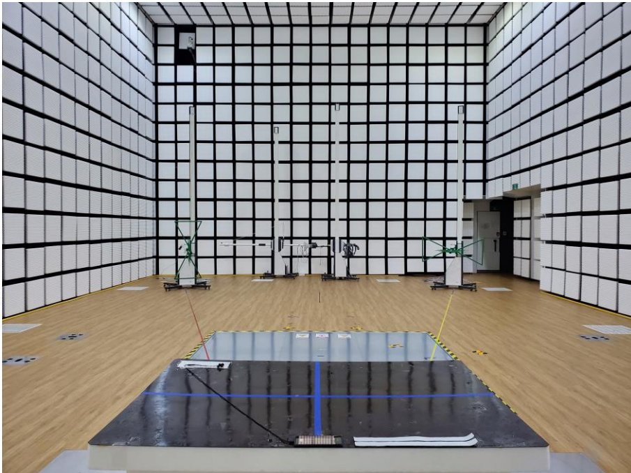
[ Mode 2 - 3 : Rear ]
