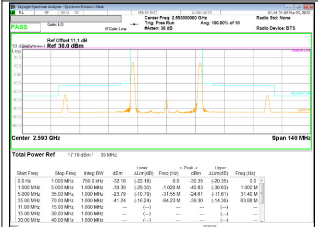
LTE B41 15MHz + 20MHz 16QAM Mid Ch RB1-0 + RB1-99
