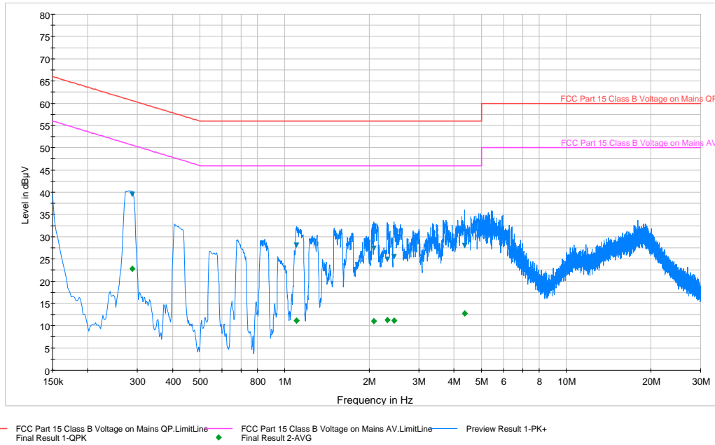
Plot 6-75. Line Conducted Plot with 802.11a UNII Band 2C (L1)
