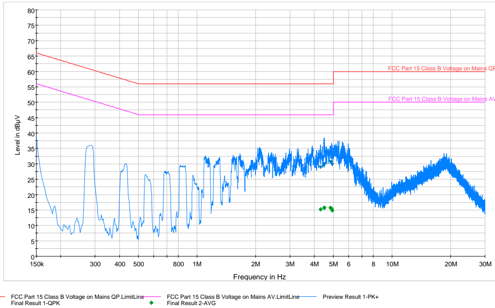
Plot 6-76. Line Conducted Plot with 802.11a UNII Band 2C (N)
