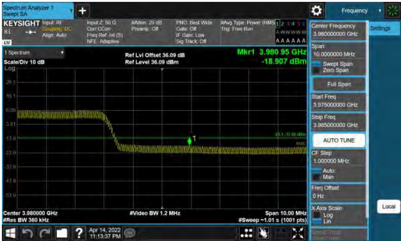
Sub6 n77. High Band Edge Plot (100 M BW Ch.662000 BPSK FullRB)(1)
