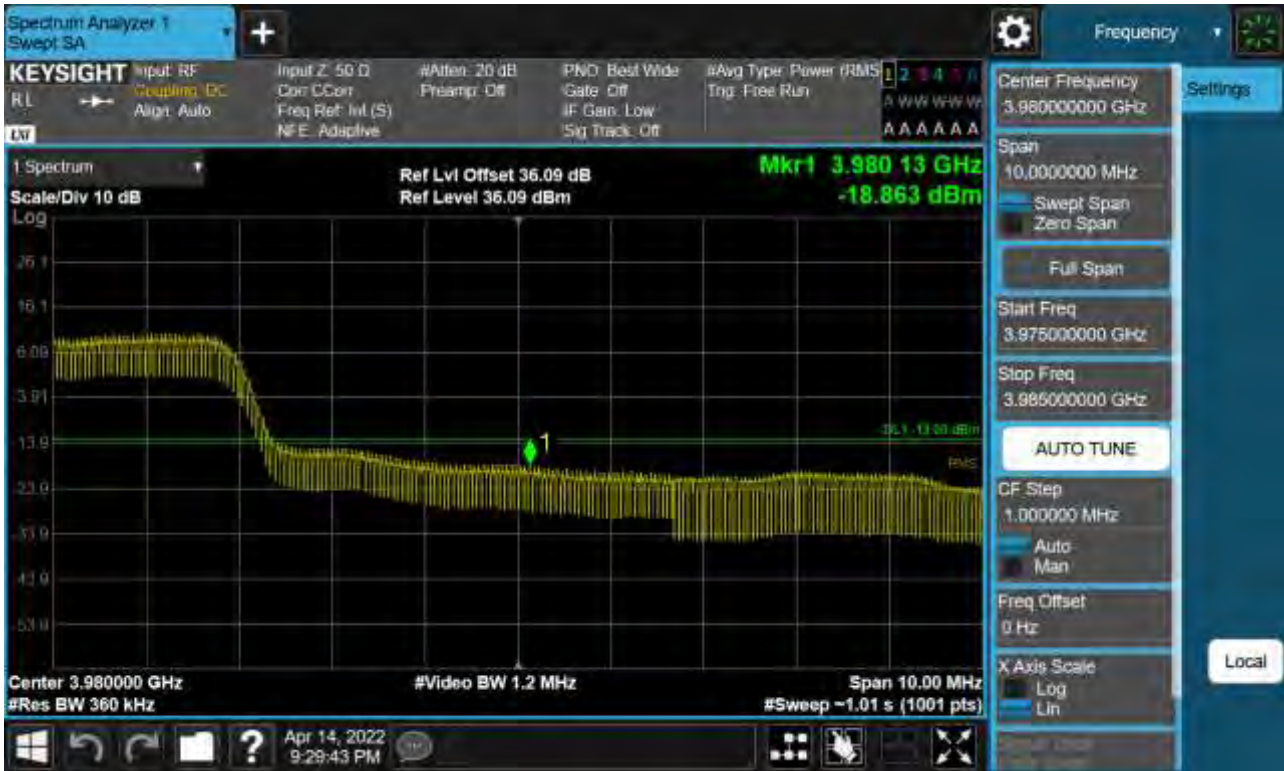
Sub6 n77. High Band Edge Plot (40 M BW Ch.664000 BPSK FullRB)(1)
