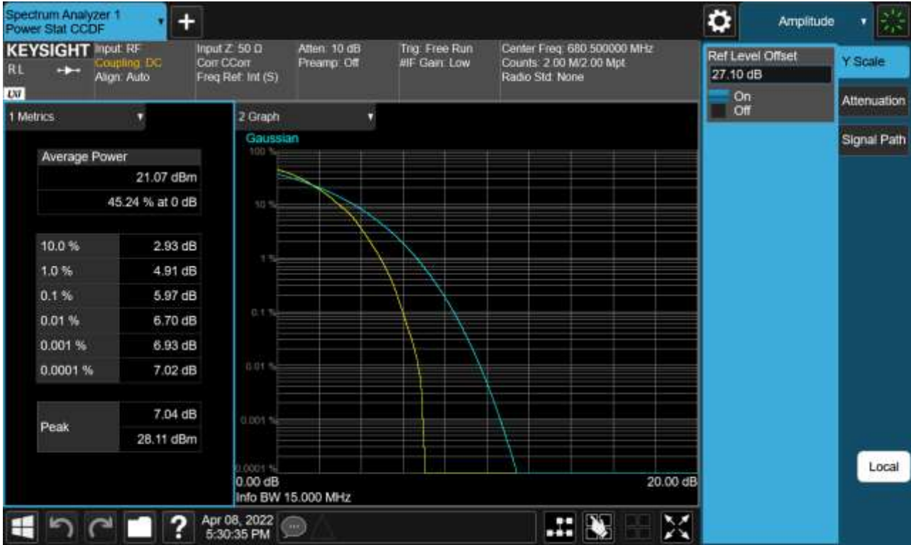
Sub6 n71. PAR Plot (15 M BW_Ch.349000_64QAM_Full RB)
