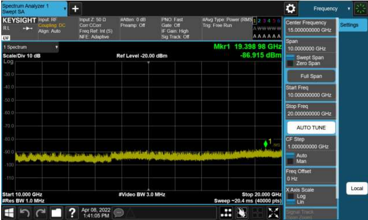
Sub6 n66. Conducted Spurious Plot_2 (345000ch_30 MHz_BPSK_RB 1_1)
