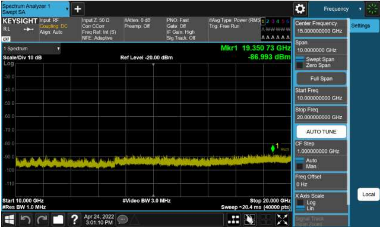
Sub6 n66. Conducted Spurious Plot_2 (349000ch_40 MHz_BPSK_RB 1_1)
