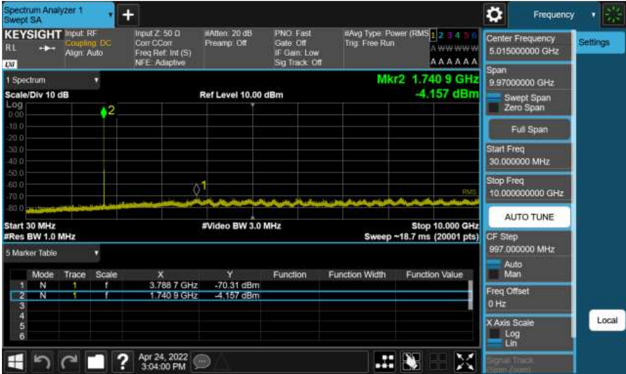
Sub6 n66. Conducted Spurious Plot_1 (352000ch_40 MHz_BPSK_RB 1_1)
