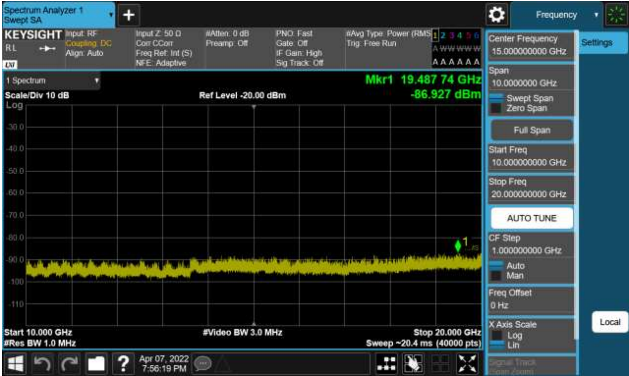
Sub6 n66. Conducted Spurious Plot_2 (343000ch_10 MHz_BPSK_RB 1_1)
