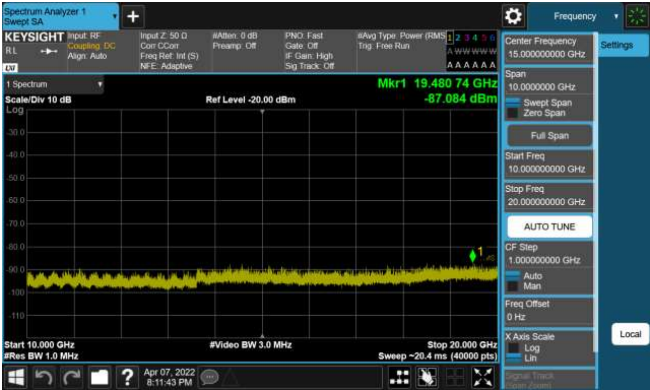
Sub6 n66. Conducted Spurious Plot_2 (349000ch_15 MHz_BPSK_RB 1_1)
