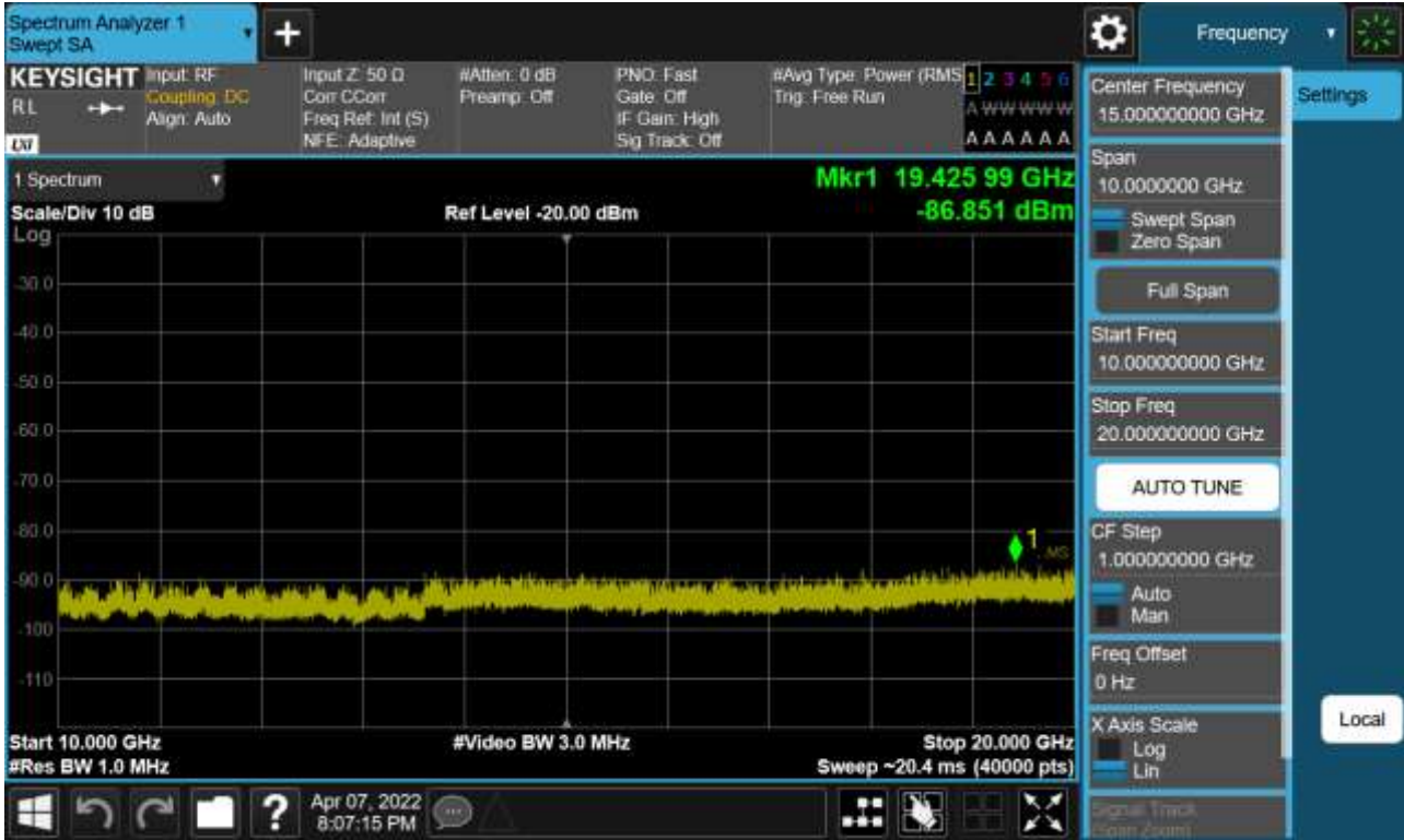
Sub6 n66. Conducted Spurious Plot_2 (343500ch_15 MHz_BPSK_RB 1_1)
