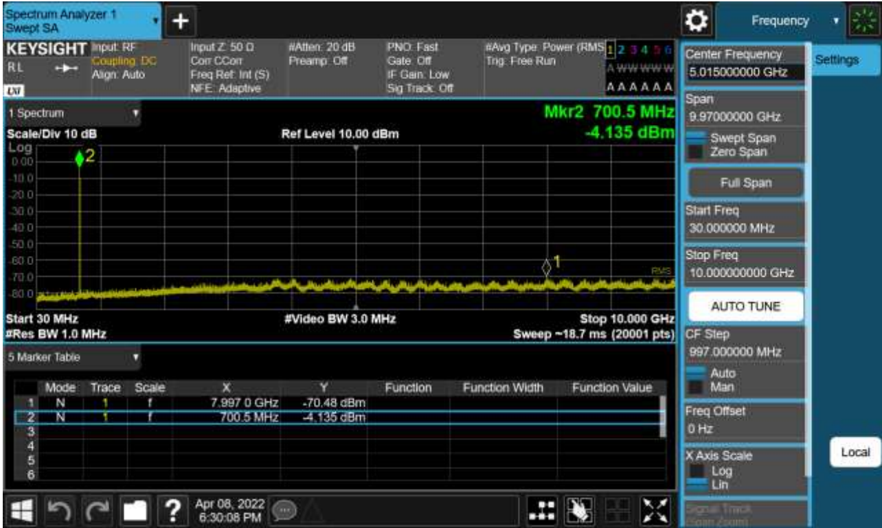
Sub6 n12. Conducted Spurious Plot _ (141500ch_15MHz_BPSK_RB 1_1)
