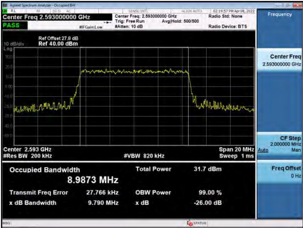
Occupied Bandwidth Plot (10 MHz Ch.40620 QPSK RB 50) (POWER CLASS 3)
