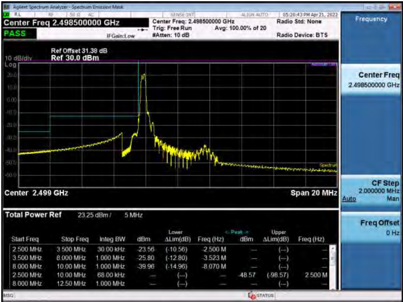
Low Channel Edge Plot (5 MHz Ch.39675 QPSK RB 1, Offset 0)-1 (POWER CLASS 2)
