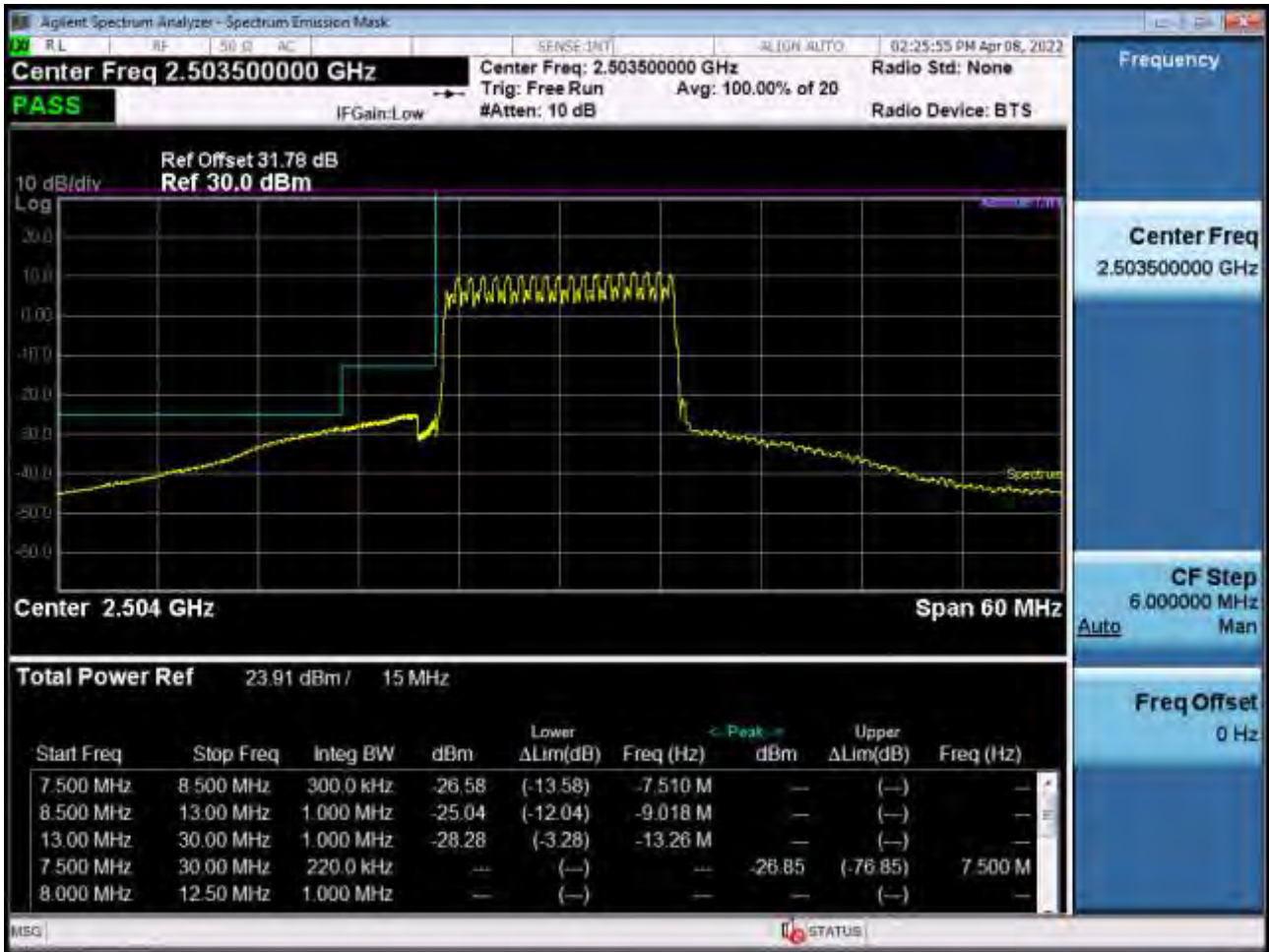
Low Channel Edge Plot (15 MHz Ch.39725 QPSK_RB75_Offset 0)-1 (POWER CLASS 3)
