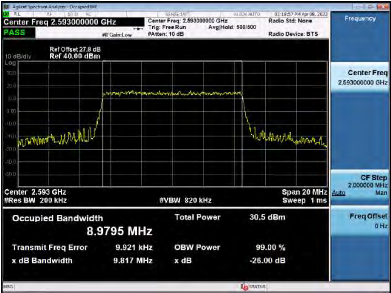
Occupied Bandwidth Plot (10 MHz Ch.40620 16-QAM RB 50) (POWER CLASS 3)
