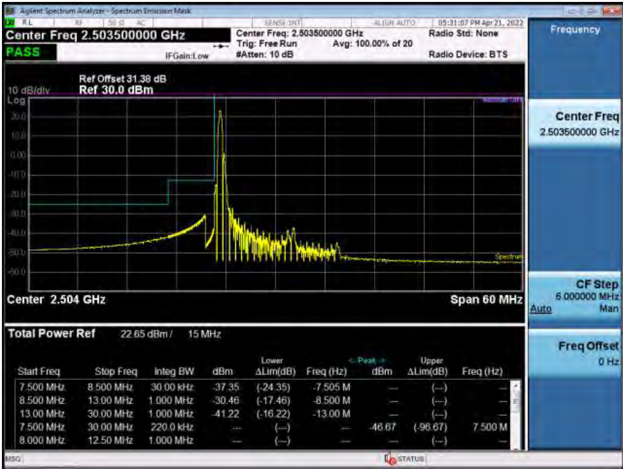
Low Channel Edge Plot (15 MHz Ch.39725 QPSK RB 1, Offset 0)-1 (POWER CLASS 2)
