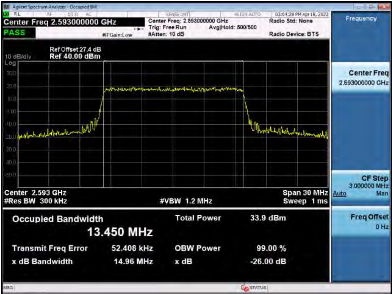
Occupied Bandwidth Plot (15 MHz Ch.40620 QPSK RB 75) (POWER CLASS 2)
