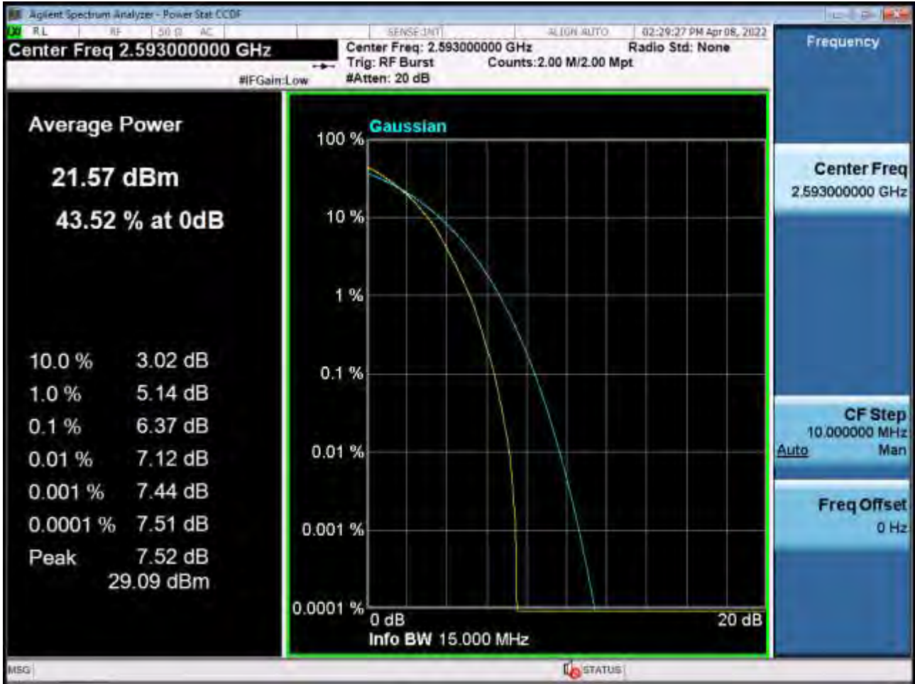
PAR Plot (15M BW_Ch.40620_64QAM_RB75_0) (POWER CLASS 3)
