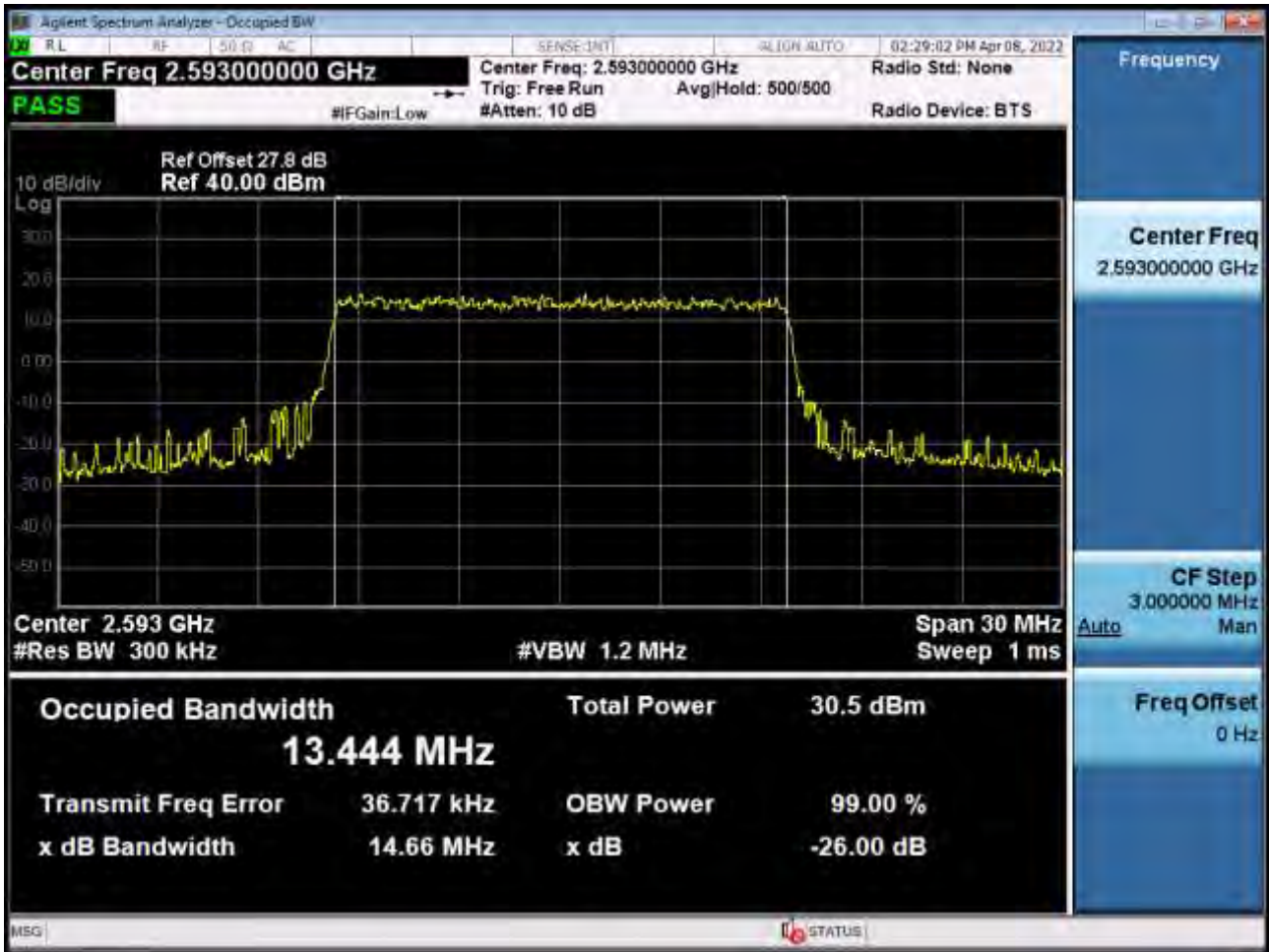
Occupied Bandwidth Plot (15 MHz Ch.40620 16-QAM RB 75) (POWER CLASS 3)
