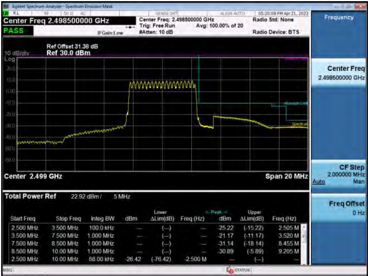
Low Channel Edge Plot (5 MHz Ch.39675 QPSK_RB25_Offset 0)-2 (POWER CLASS 2)
