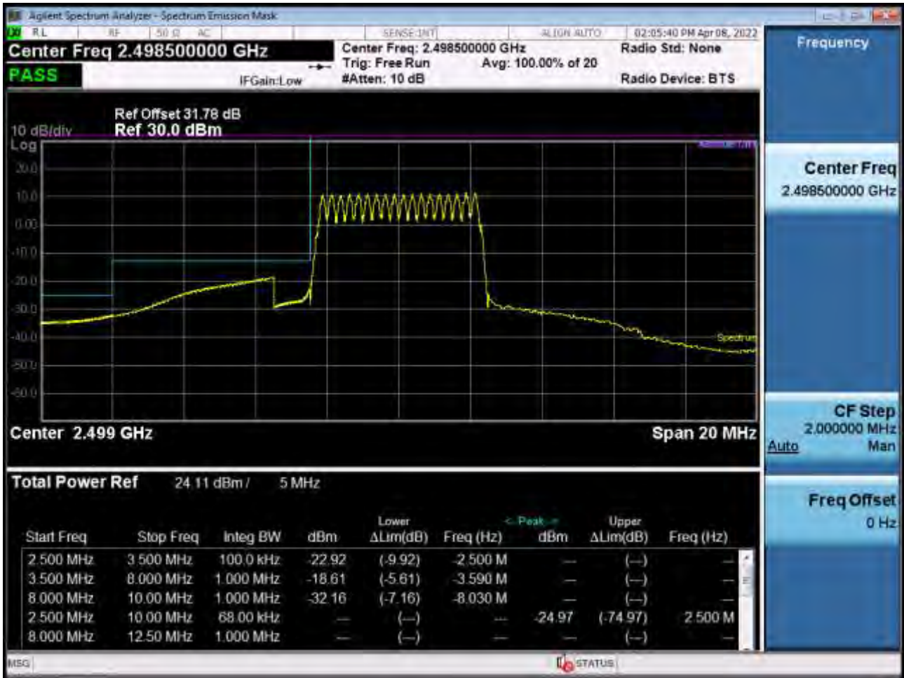
Low Channel Edge Plot (5 MHz Ch.39675 QPSK_RB25_Offset 0)-1 (POWER CLASS 3)
