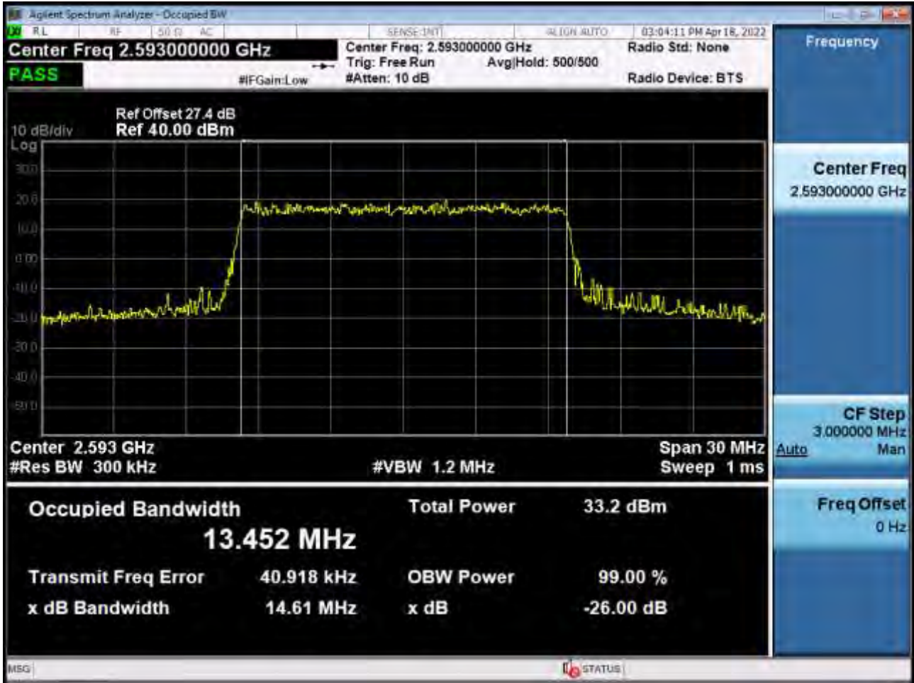
Occupied Bandwidth Plot (15 MHz Ch.40620 64-QAM RB 75) (POWER CLASS 2)
