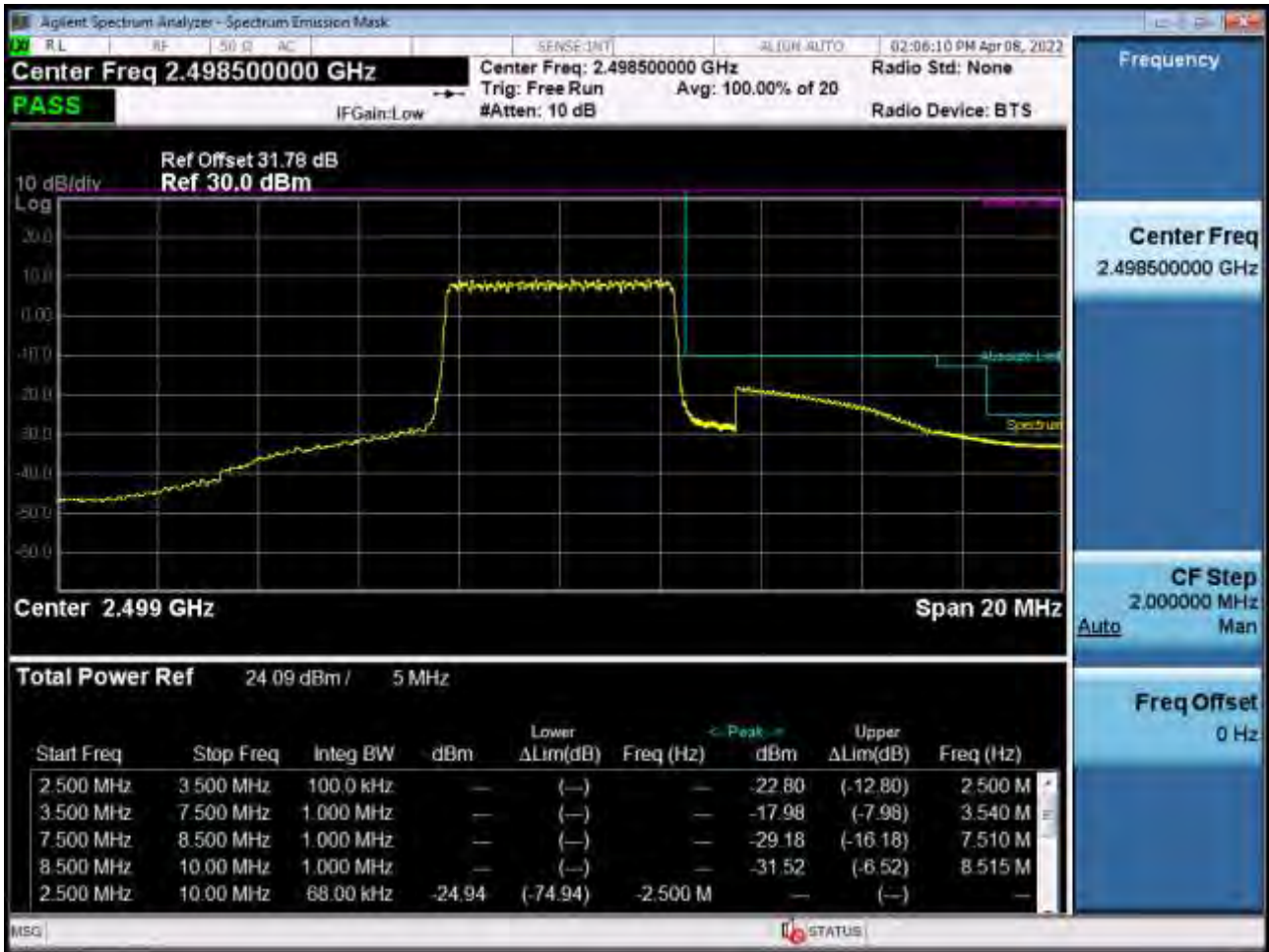
Low Channel Edge Plot (5 MHz Ch.39675 QPSK_RB25_Offset 0)-2 (POWER CLASS 3)
