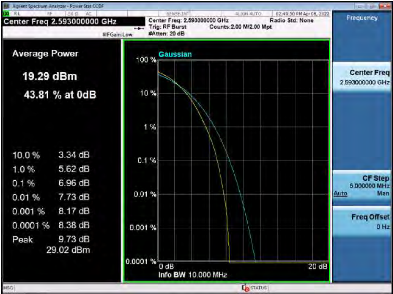
PAR Plot (10M BW_Ch.40620_256QAM_RB50_0) (POWER CLASS 3)
