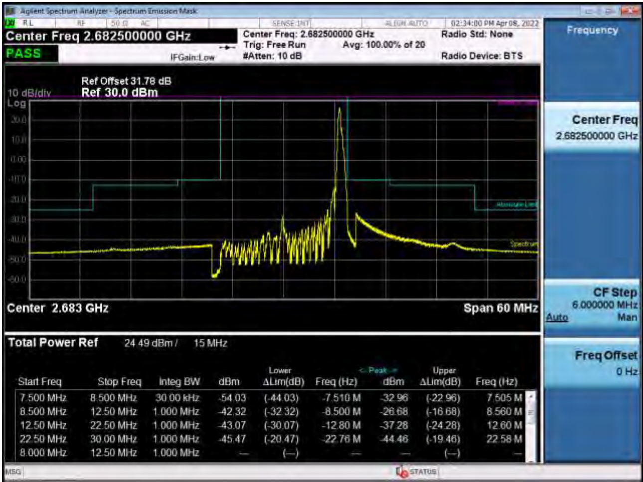
High Channel Edge Plot (15 MHz Ch.41515 QPSK RB 1, Offset 74) (POWER CLASS 3)
