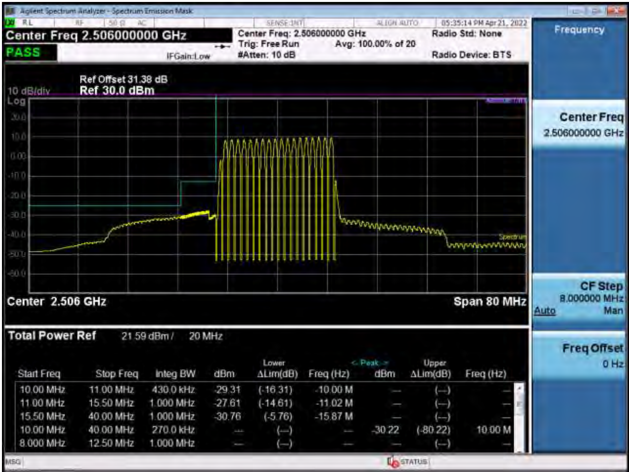
Low Channel Edge Plot (20 MHz Ch.39750 QPSK_RB100_Offset 0)-1 (POWER CLASS 2)
