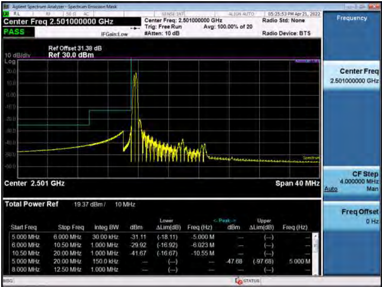
Low Channel Edge Plot (10 MHz Ch.39700 QPSK RB 1, Offset 0)-1 (POWER CLASS 2)
