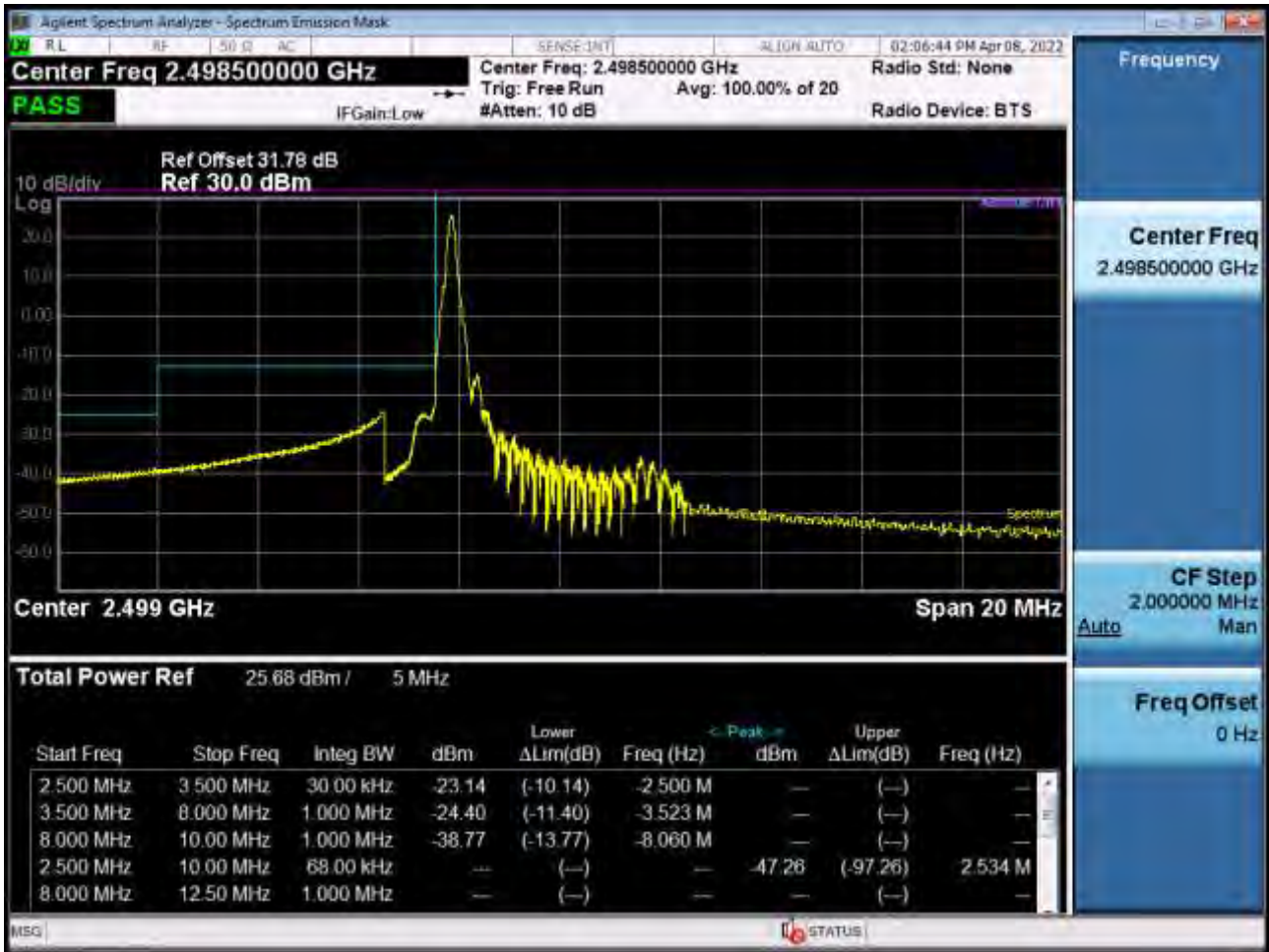
Low Channel Edge Plot (5 MHz Ch.39675 QPSK RB 1, Offset 0)-1 (POWER CLASS 3)
