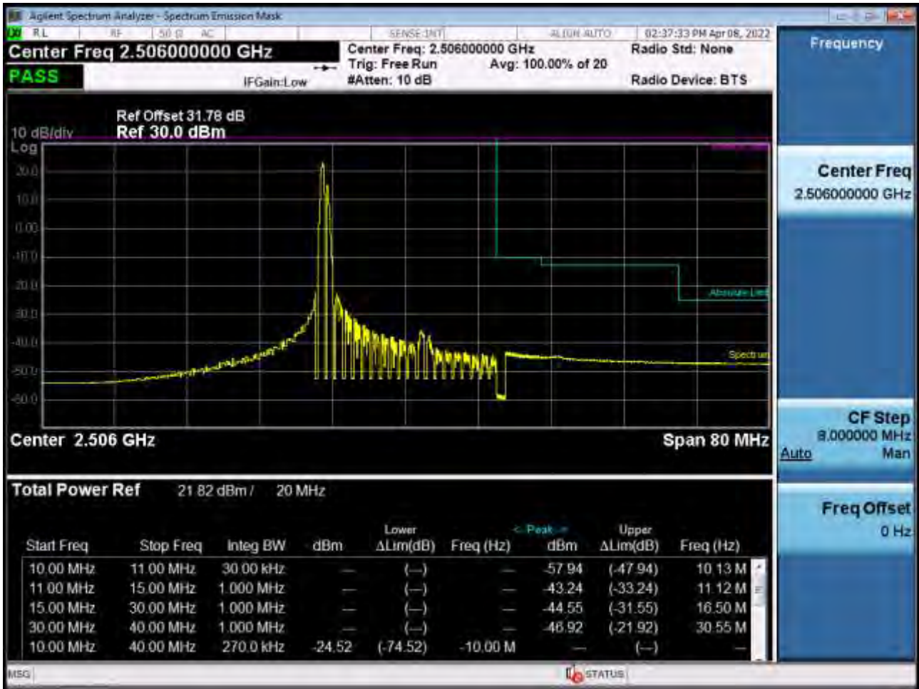
Low Channel Edge Plot (20 MHz Ch.39750 QPSK RB 1, Offset 0)-2 (POWER CLASS 3)
