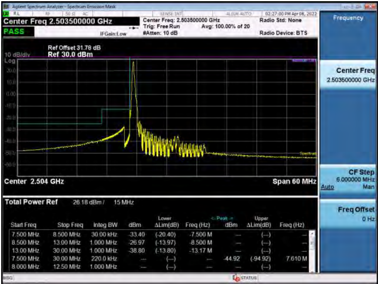
Low Channel Edge Plot (15 MHz Ch.39725 QPSK RB 1, Offset 0)-1 (POWER CLASS 3)
