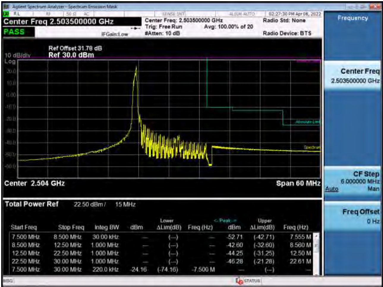
Low Channel Edge Plot (15 MHz Ch.39725 QPSK RB 1, Offset 0)-2 (POWER CLASS 3)
