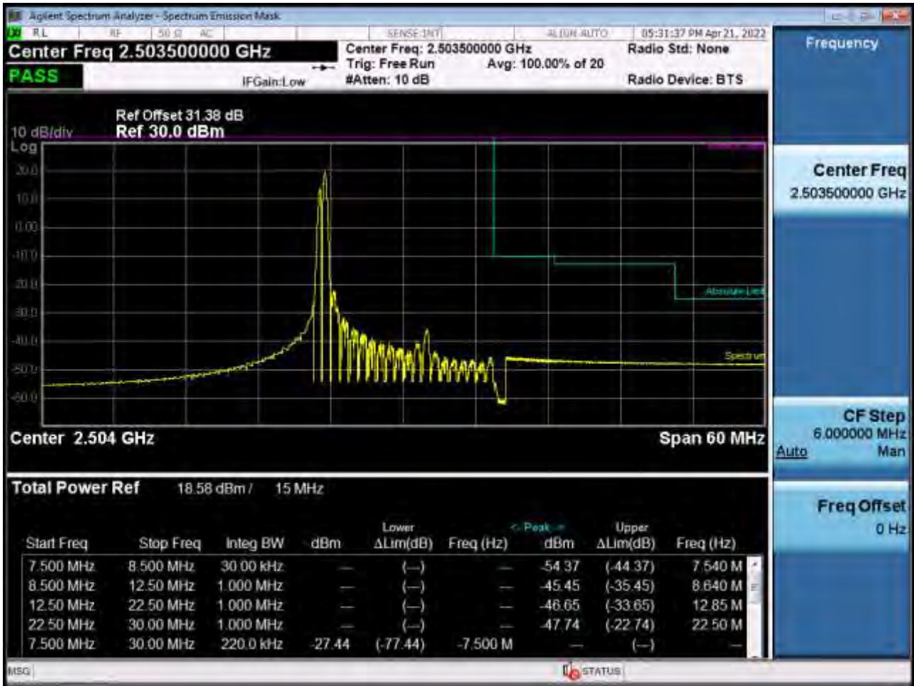
Low Channel Edge Plot (15 MHz Ch.39725 QPSK RB 1, Offset 0)-2 (POWER CLASS 2)
