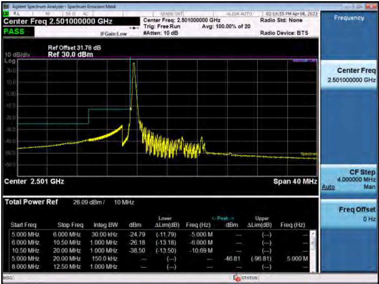
Low Channel Edge Plot (10 MHz Ch.39700 QPSK RB 1, Offset 0)-1 (POWER CLASS 3)
