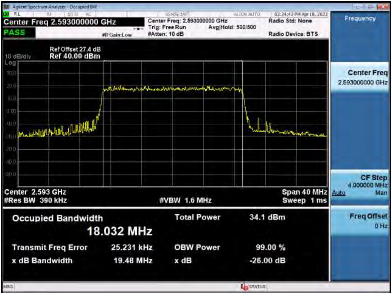
Occupied Bandwidth Plot (20 MHz Ch.40620 QPSK RB 100) (POWER CLASS 2)
