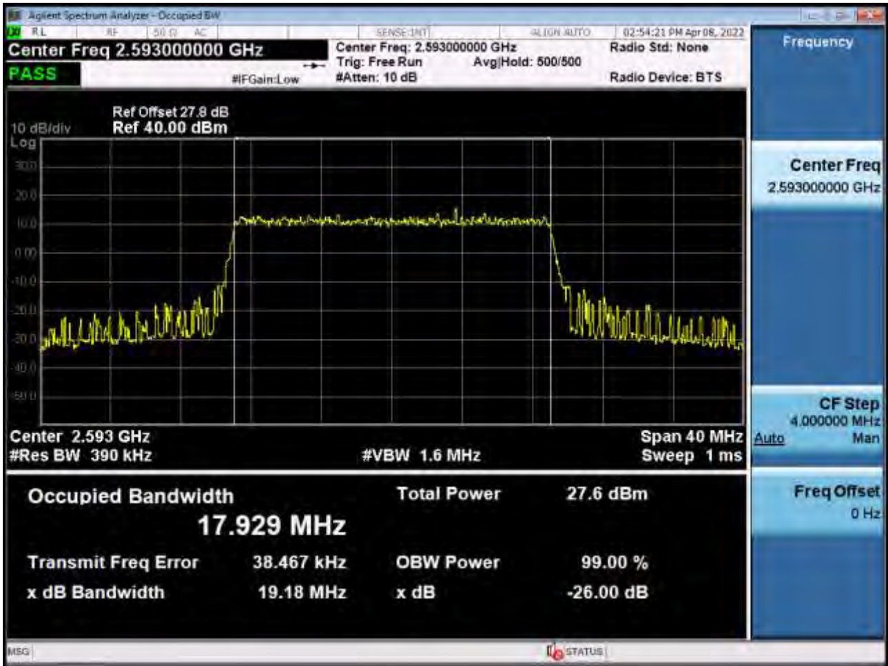
Occupied Bandwidth Plot (20 MHz Ch.40620 256-QAM RB 100) (POWER CLASS 3)
