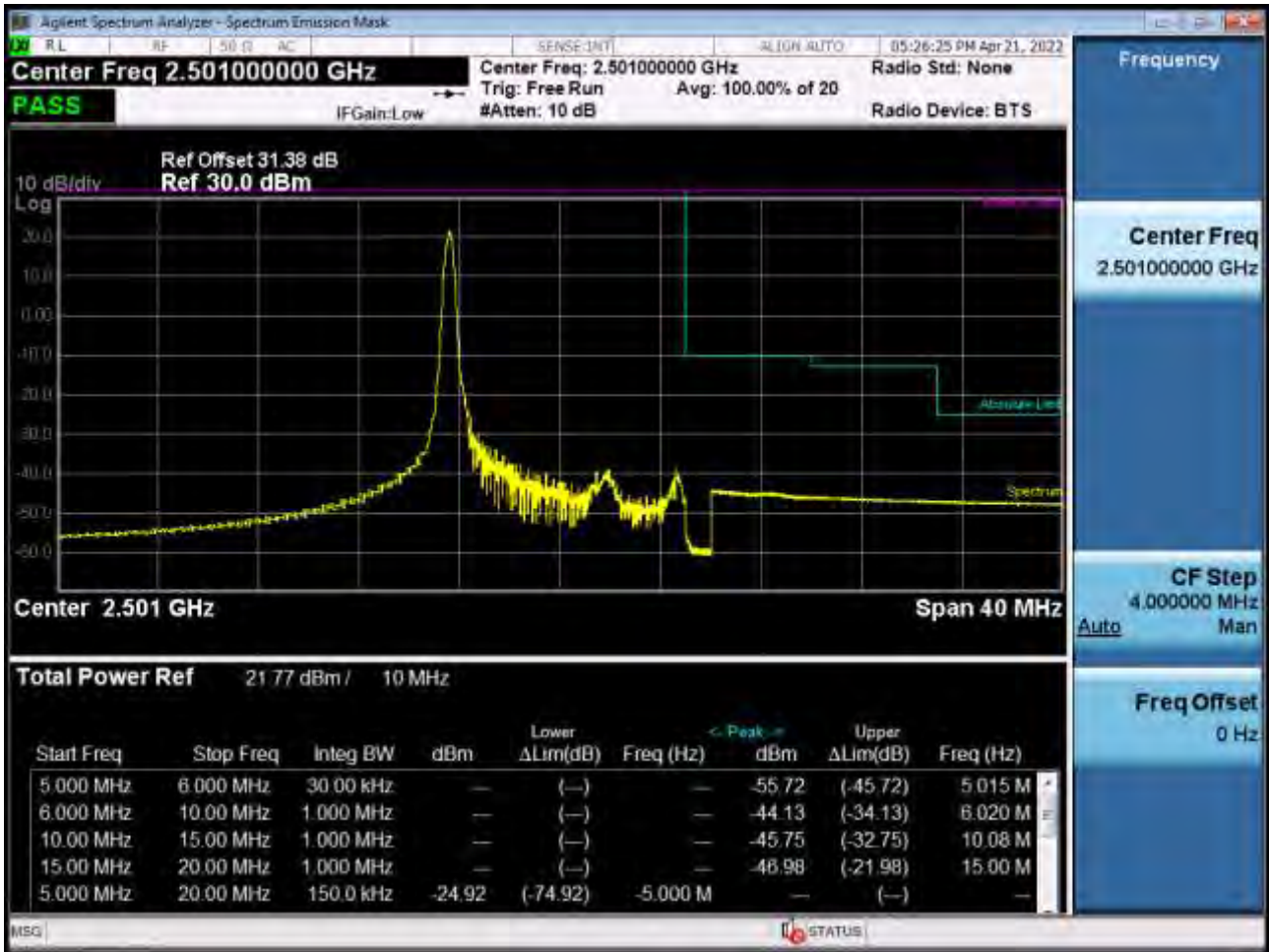
Low Channel Edge Plot (10 MHz Ch.39700 QPSK RB 1, Offset 0)-2 (POWER CLASS 2)
