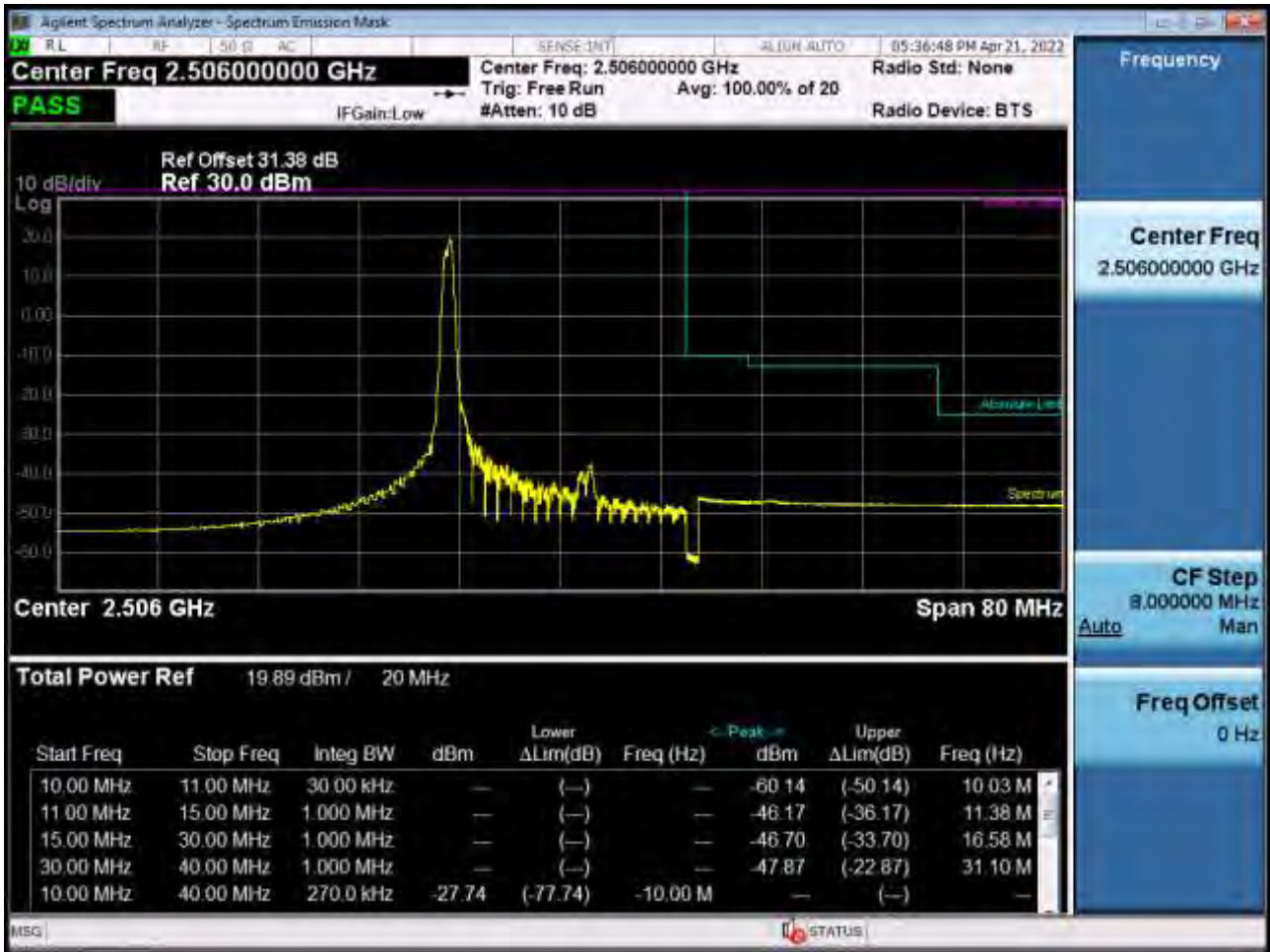
Low Channel Edge Plot (20 MHz Ch.39750 QPSK RB 1, Offset 0)-2 (POWER CLASS 2)
