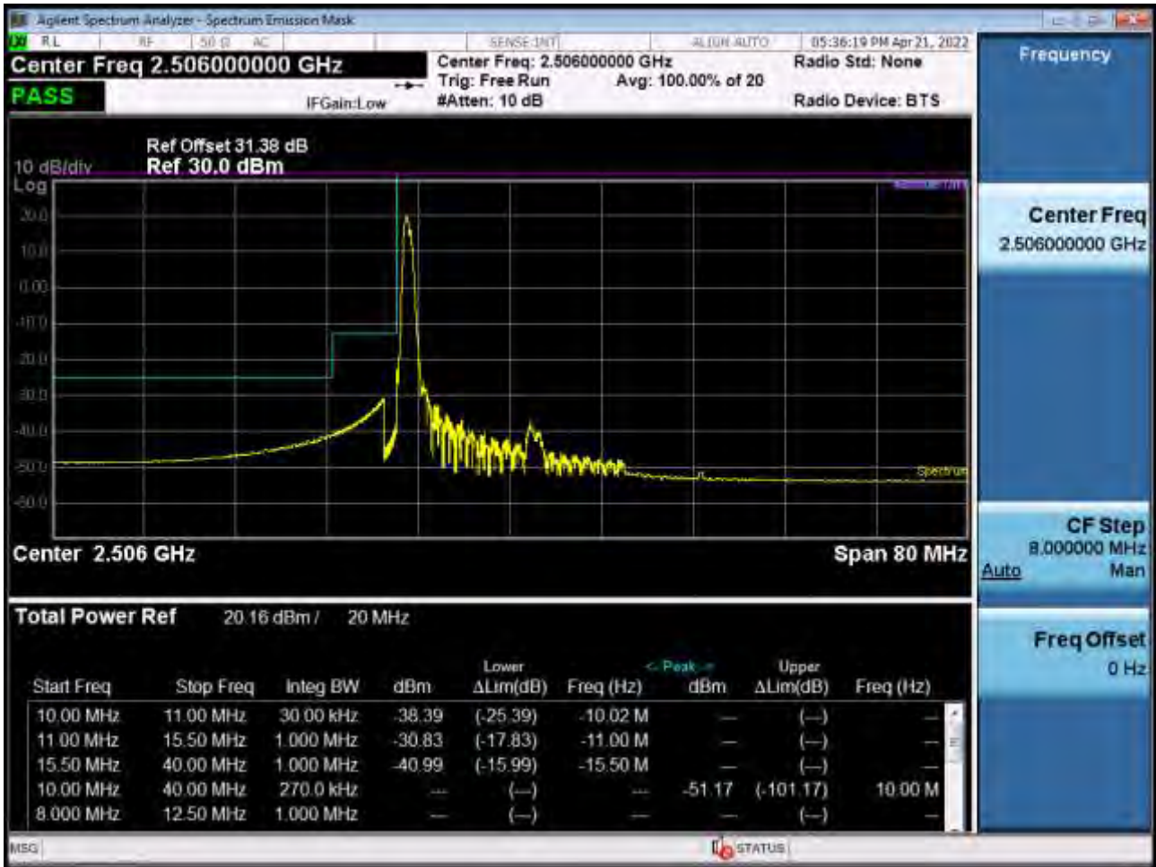
Low Channel Edge Plot (20 MHz Ch.39750 QPSK RB 1, Offset 0)-1 (POWER CLASS 2)
