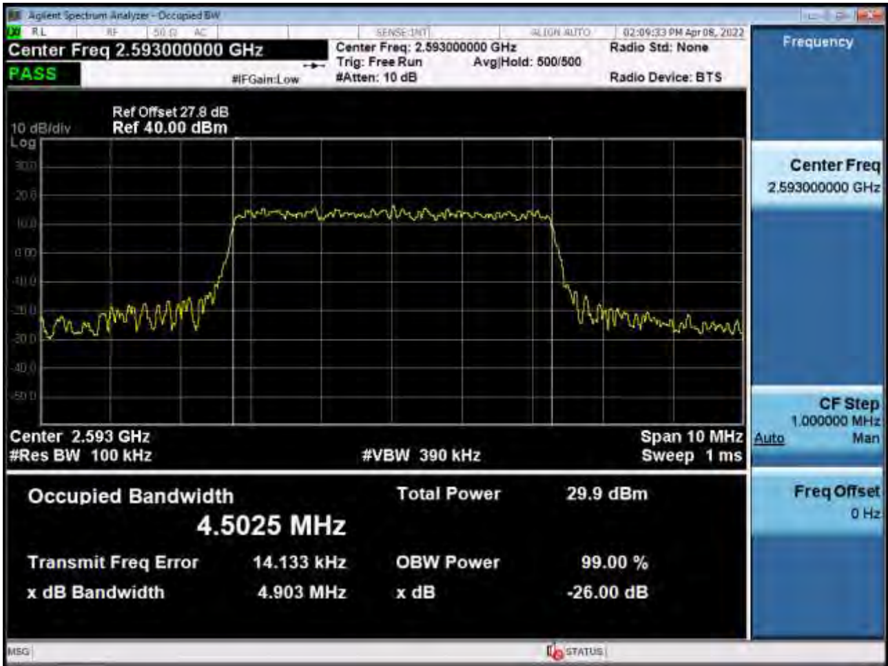
Occupied Bandwidth Plot (5 MHz Ch.40620 64-QAM RB 25) (POWER CLASS 3)
