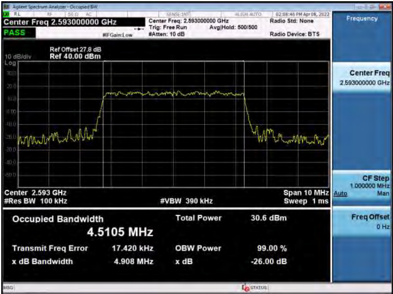
Occupied Bandwidth Plot (5 MHz Ch.40620 16-QAM RB 25) (POWER CLASS 3)
