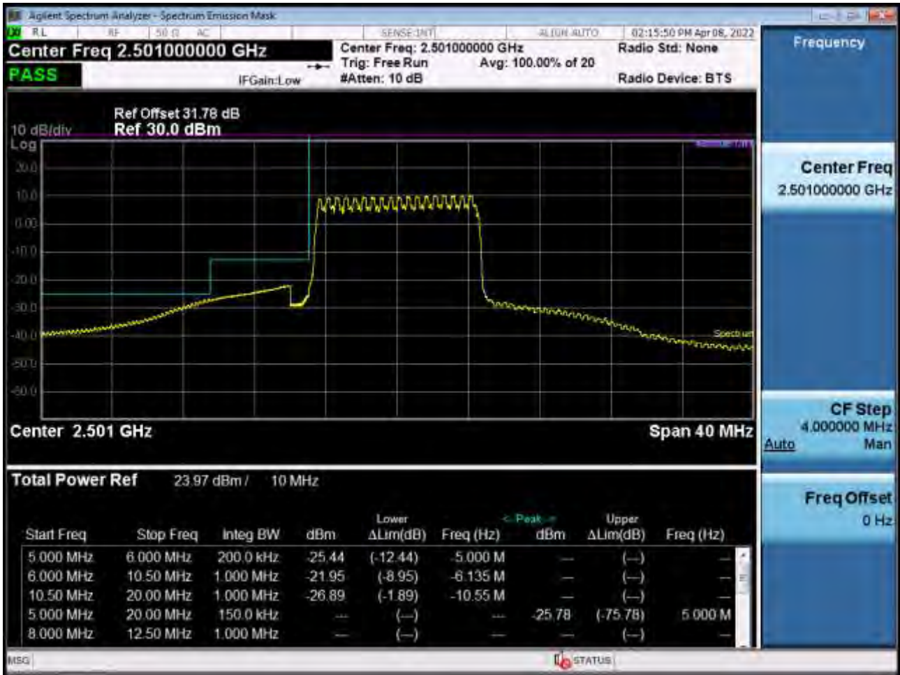
Low Channel Edge Plot (10 MHz Ch.39700 QPSK_RB50_Offset 0)-1 (POWER CLASS 3)
