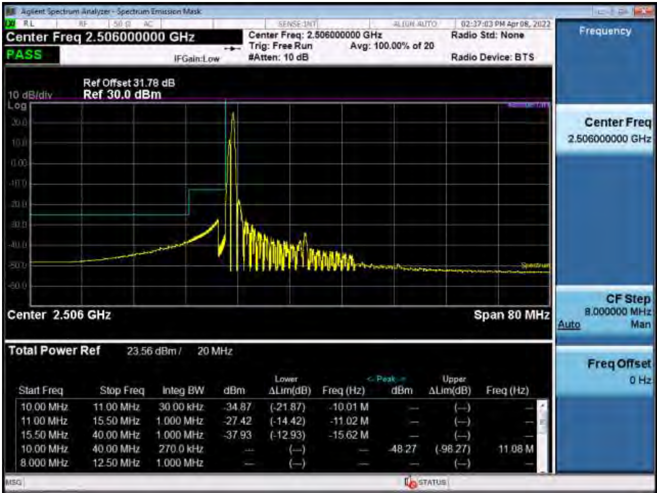
Low Channel Edge Plot (20 MHz Ch.39750 QPSK RB 1, Offset 0)-1 (POWER CLASS 3)
