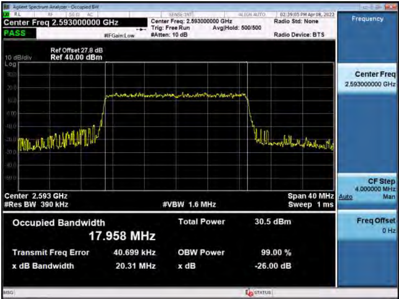
Occupied Bandwidth Plot (20 MHz Ch.40620 16-QAM RB 100) (POWER CLASS 3)
