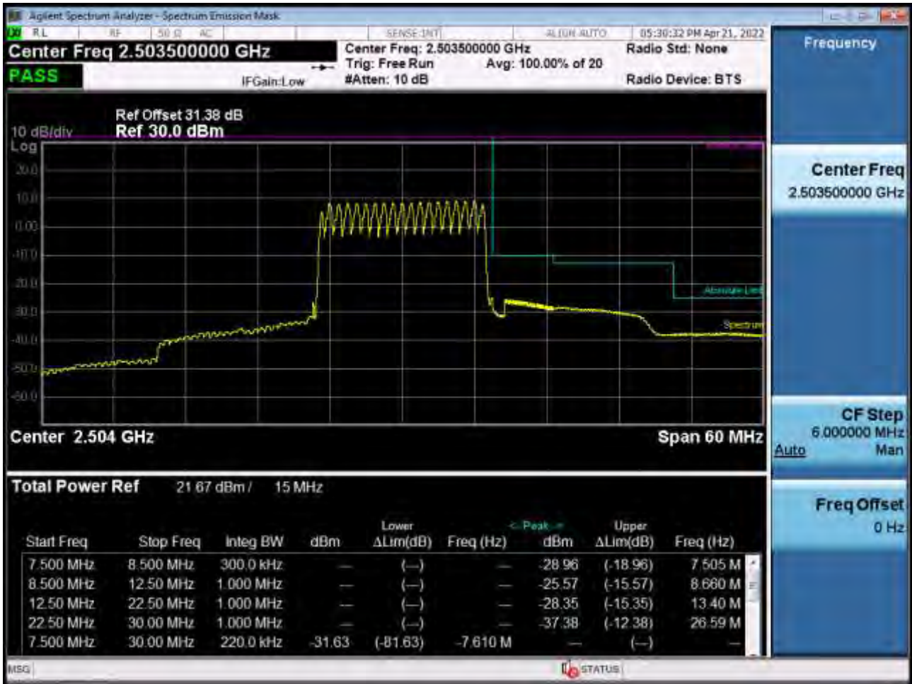
Low Channel Edge Plot (15 MHz Ch.39725 QPSK_RB75_Offset 0)-2 (POWER CLASS 2)
