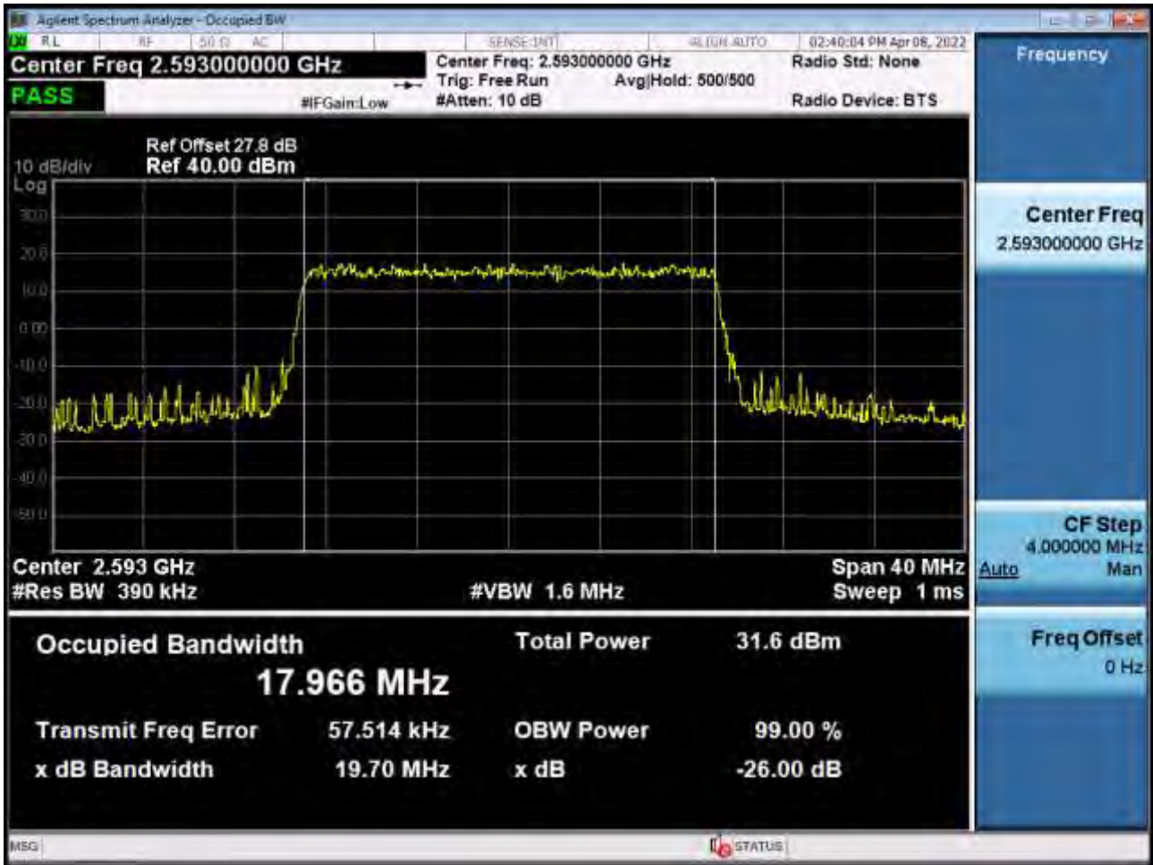
Occupied Bandwidth Plot (20 MHz Ch.40620 QPSK RB 100) (POWER CLASS 3)
