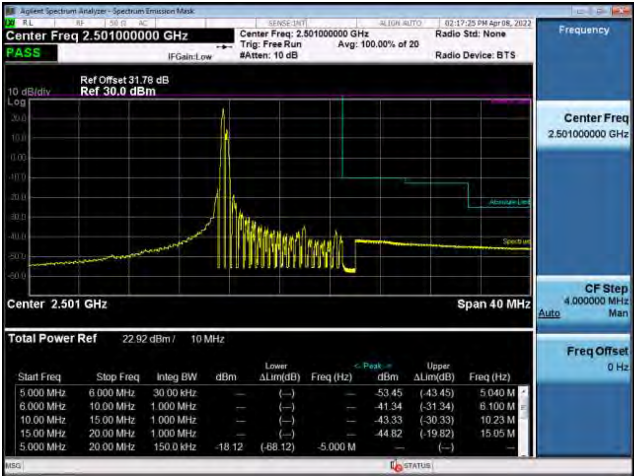
Low Channel Edge Plot (10 MHz Ch.39700 QPSK RB 1, Offset 0)-2 (POWER CLASS 3)
