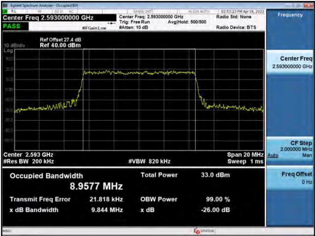
Occupied Bandwidth Plot (10 MHz Ch.40620 16-QAM RB 50) (POWER CLASS 2)
