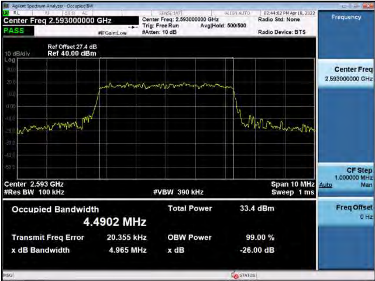
Occupied Bandwidth Plot (5 MHz Ch.40620 64-QAM RB 25) (POWER CLASS 2)
