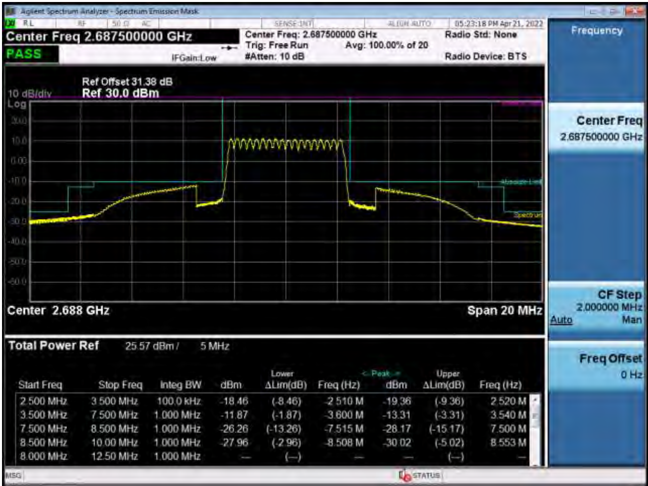
High Channel Edge Plot (5 MHz Ch.41565 QPSK_RB25_Offset 0) (POWER CLASS 2)
