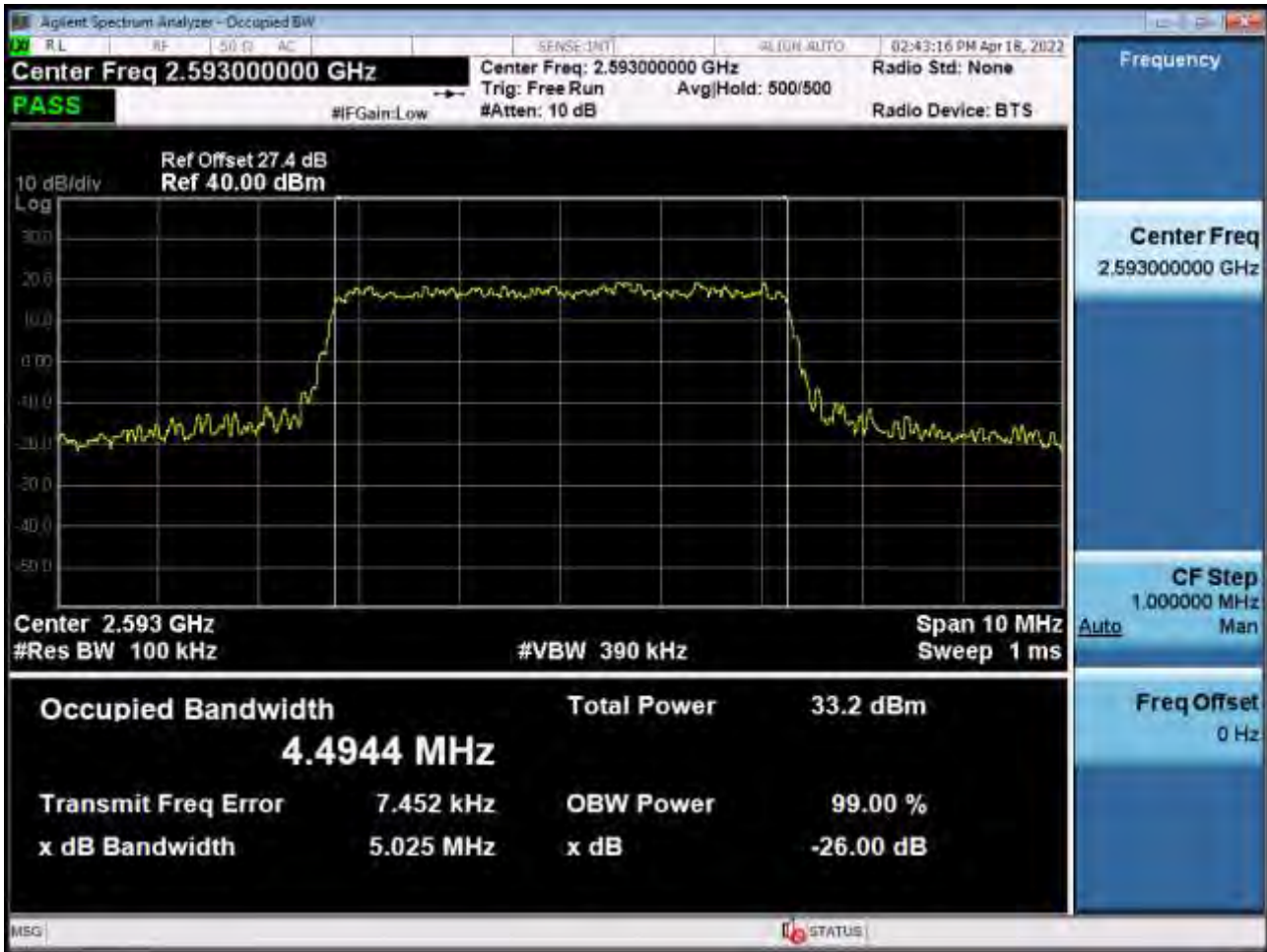
Occupied Bandwidth Plot (5 MHz Ch.40620 16-QAM RB 25) (POWER CLASS 2)
