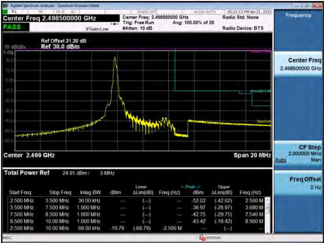
Low Channel Edge Plot (5 MHz Ch.39675 QPSK RB 1, Offset 0)-2 (POWER CLASS 2)
