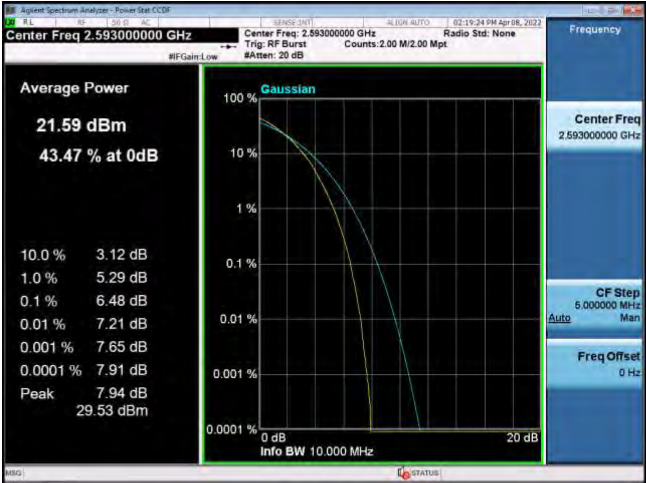
PAR Plot (10M BW_Ch.40620_64QAM_RB50_0) (POWER CLASS 3)
