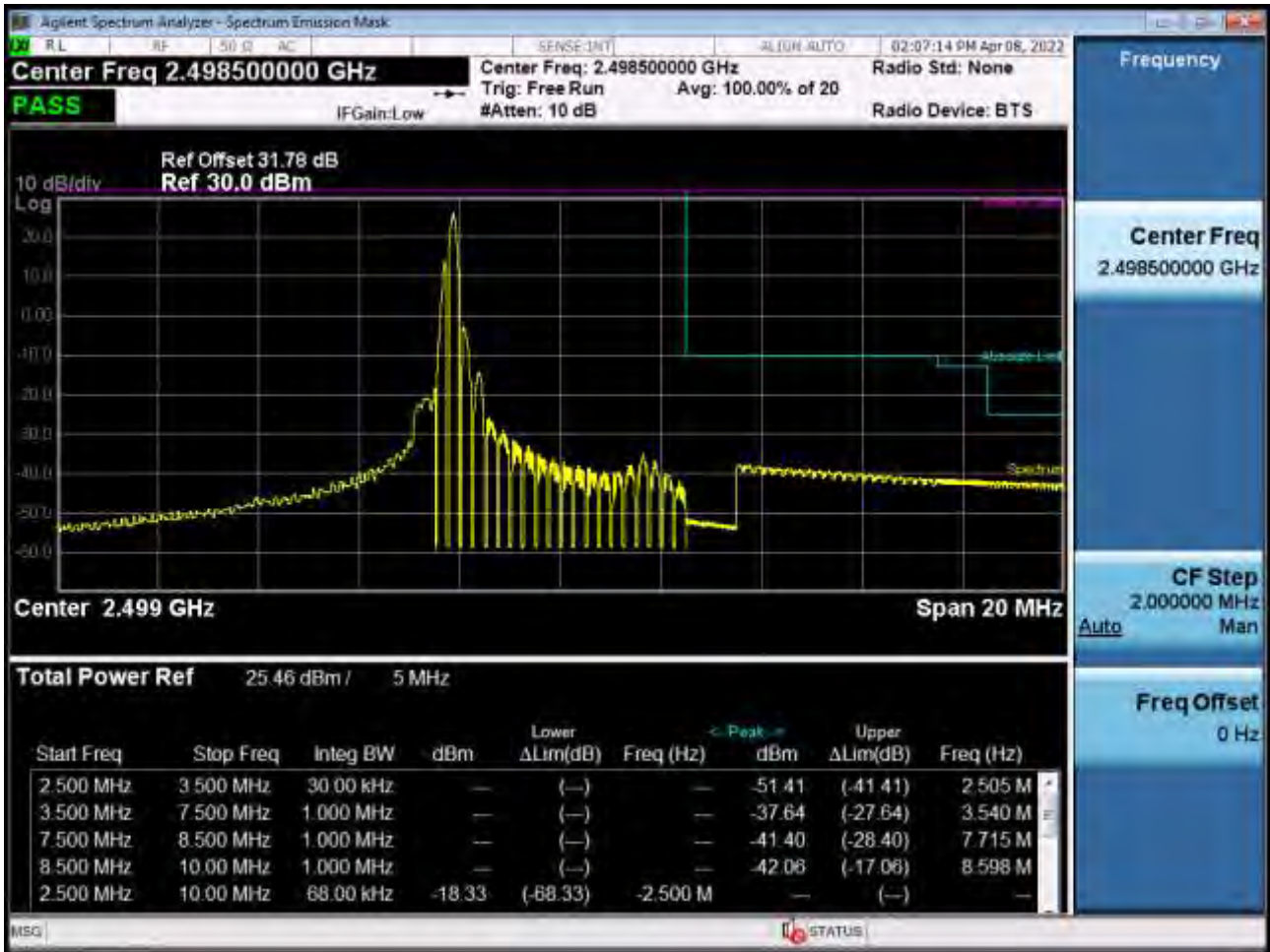
Low Channel Edge Plot (5 MHz Ch.39675 QPSK RB 1, Offset 0)-2 (POWER CLASS 3)
