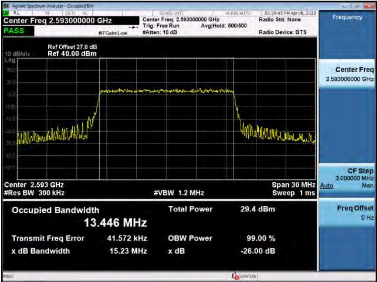
Occupied Bandwidth Plot (15 MHz Ch.40620 64-QAM RB 75) (POWER CLASS 3)
