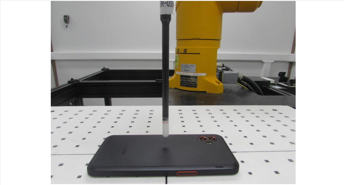
Distance of 9.95 mm from the EUT
