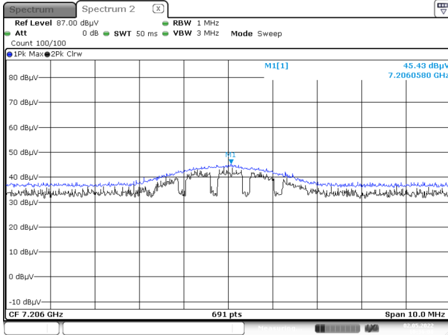
Radiated Spurious Emissions plot – Average & Peak Result (3rd Harmonic, X-V)
