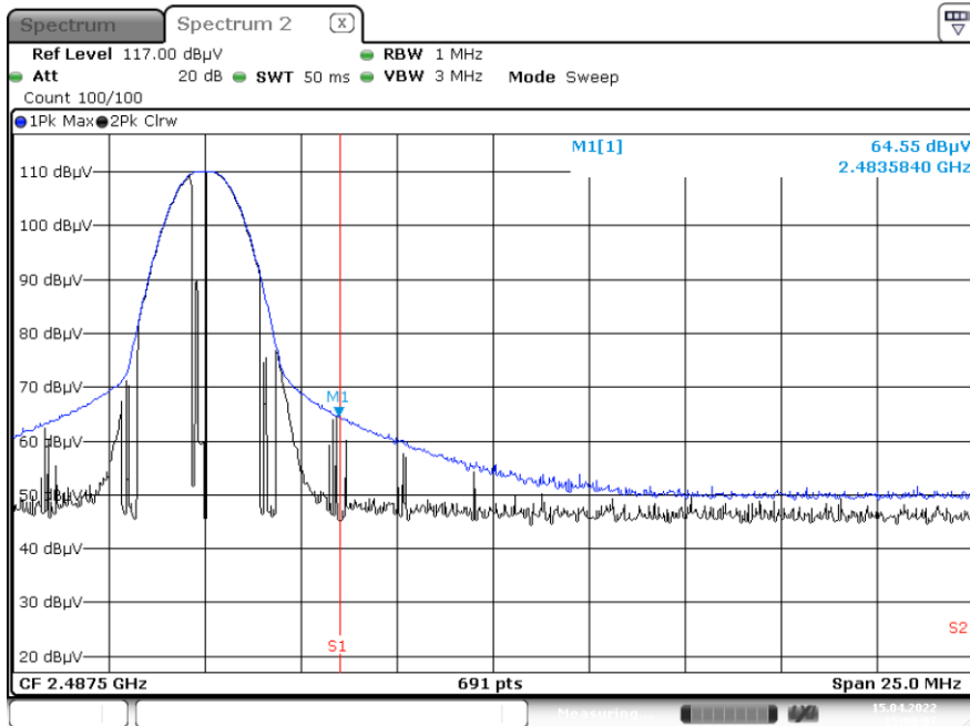
Radiated Restricted Band Edges plot –Peak&AverageResult(GFSK, Ch.78, Z-V)
