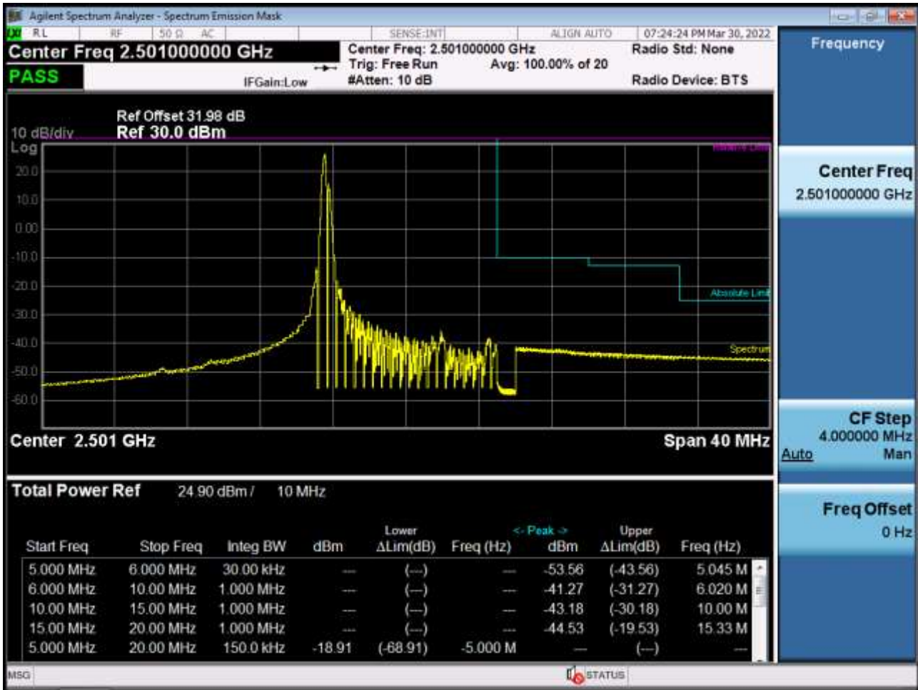
Low Channel Edge Plot (10 MHz Ch.39700 QPSK RB 1, Offset 0)-2
