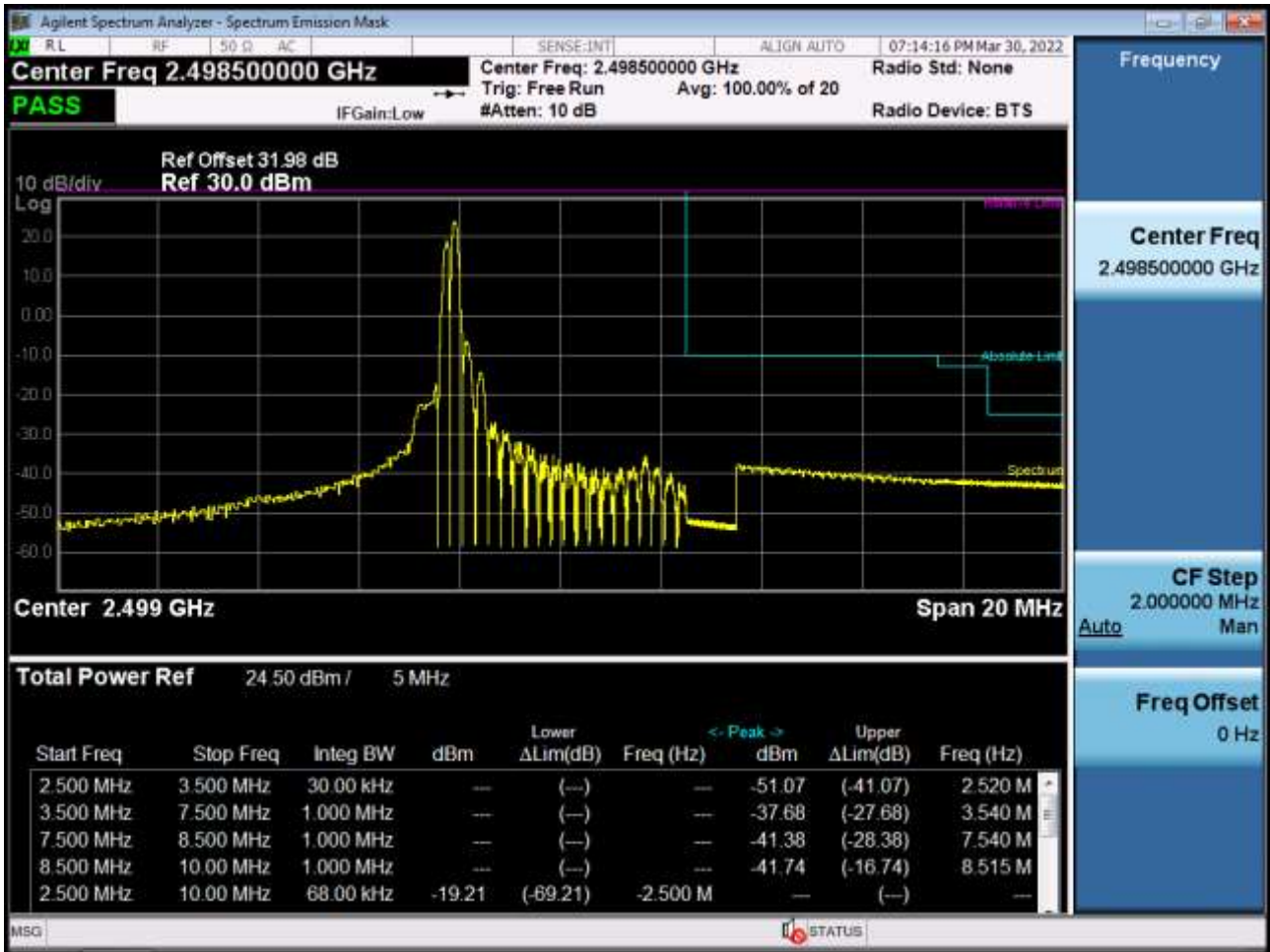
Low Channel Edge Plot (5 MHz Ch.39675 QPSK RB 1, Offset 0)-2
