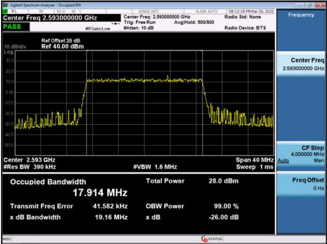
Occupied Bandwidth Plot (20 MHz Ch.40620 256-QAM RB 100)
