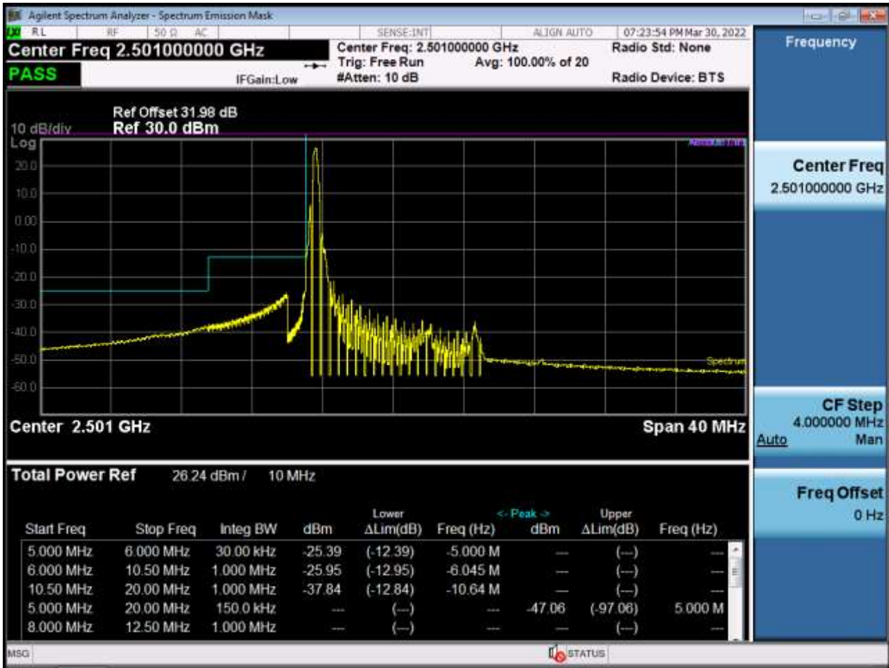
Low Channel Edge Plot (10 MHz Ch.39700 QPSK RB 1, Offset 0)-1
