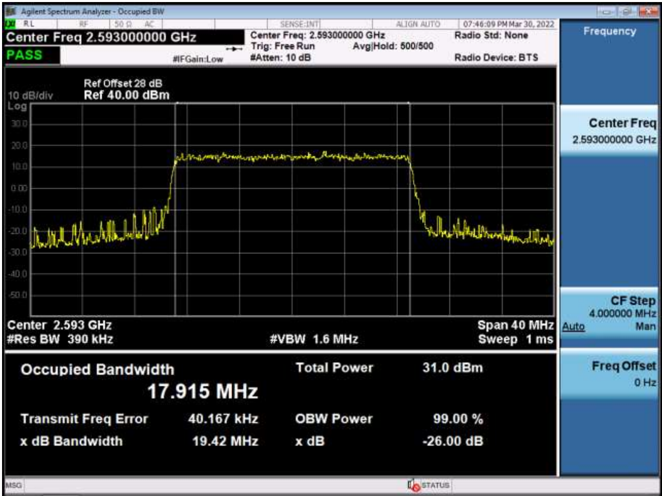
Occupied Bandwidth Plot (20 MHz Ch.40620 16-QAM RB 100)
