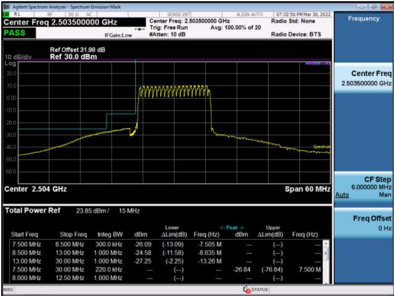
Low Channel Edge Plot (15 MHz Ch.39725 QPSK_RB75_Offset 0)-1
