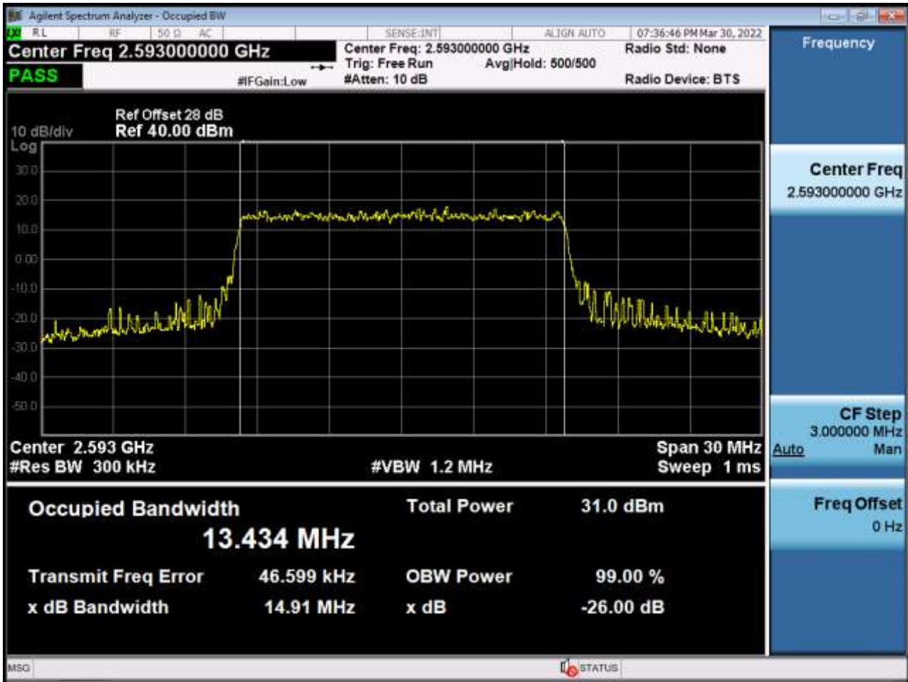
Occupied Bandwidth Plot (15 MHz Ch.40620 64-QAM RB 75)
