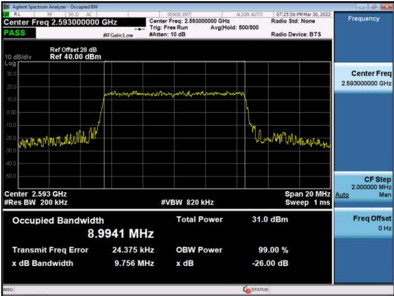
Occupied Bandwidth Plot (10 MHz Ch.40620 16-QAM RB 50)
