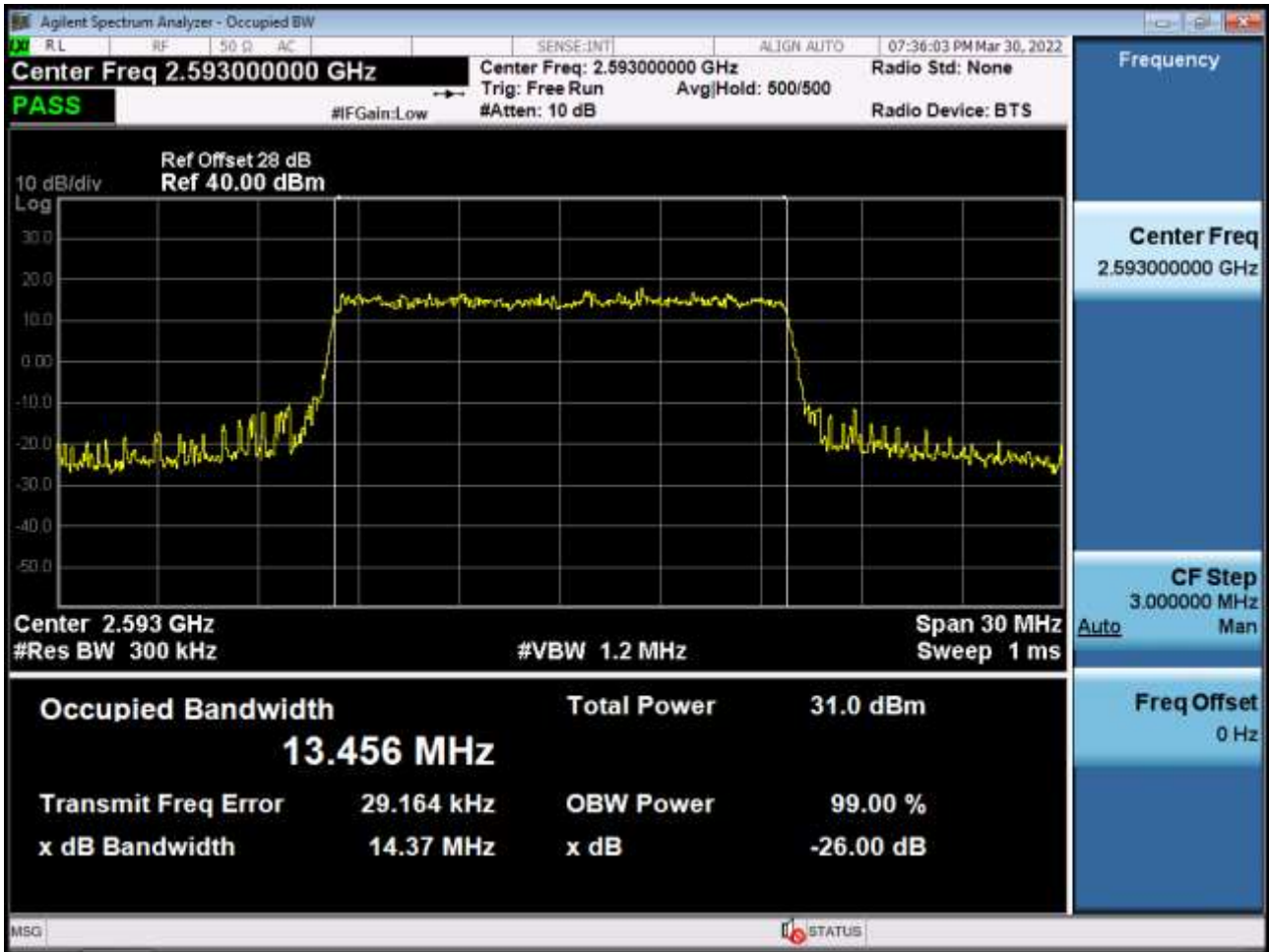
Occupied Bandwidth Plot (15 MHz Ch.40620 16-QAM RB 75)
