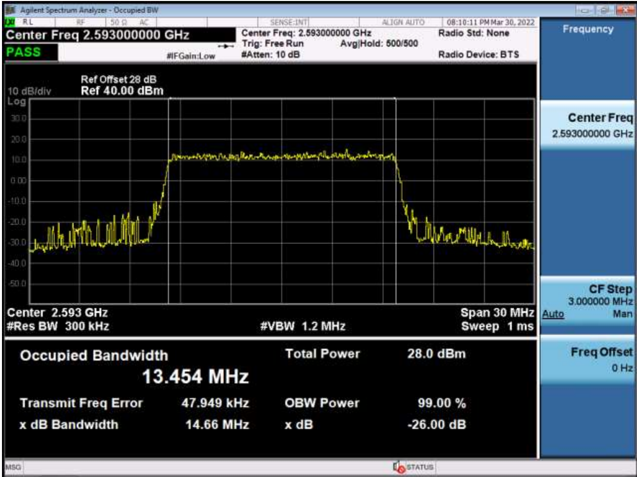
Occupied Bandwidth Plot (15 MHz Ch.40620 256-QAM RB 75)
