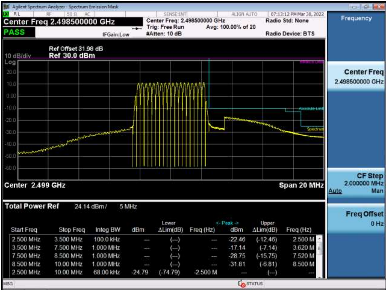
Low Channel Edge Plot (5 MHz Ch.39675 QPSK_RB25_Offset 0)-2
