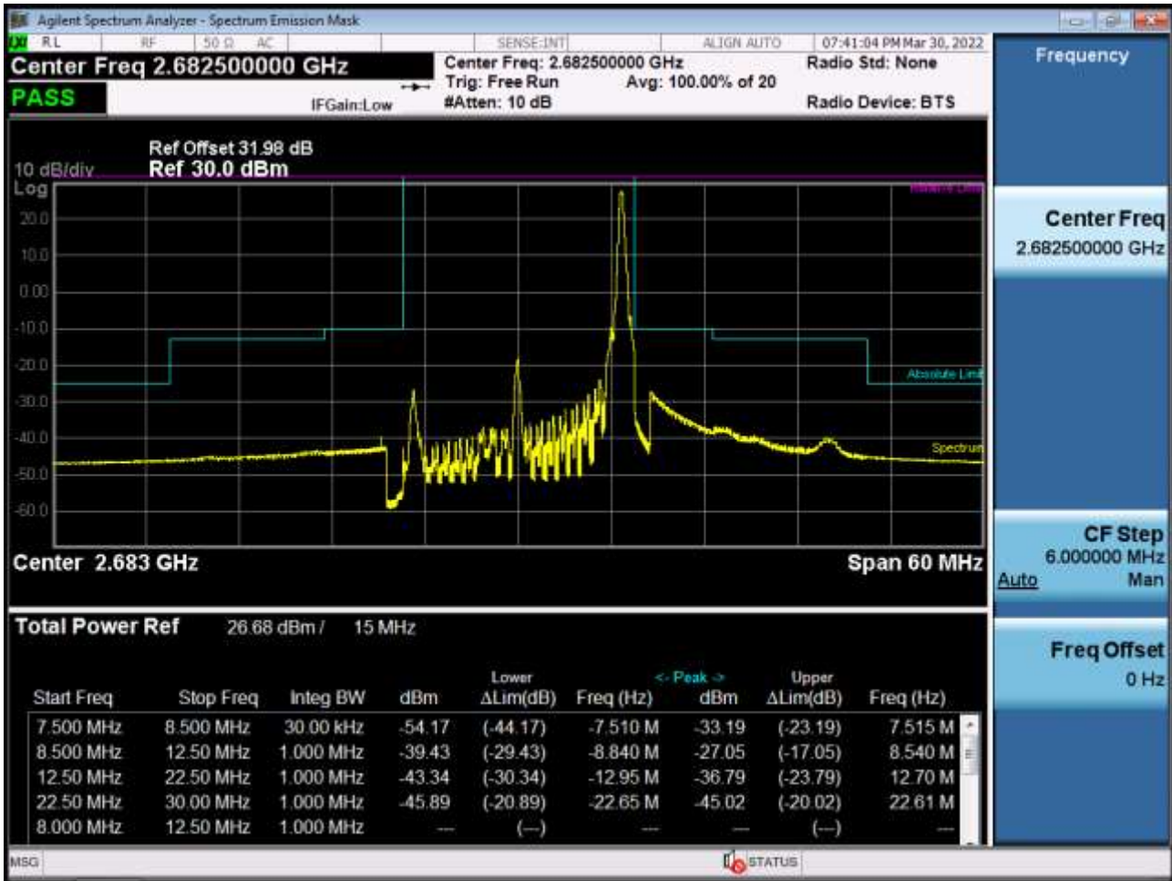
High Channel Edge Plot (15 MHz Ch.41515 QPSK RB 1, Offset 74)
