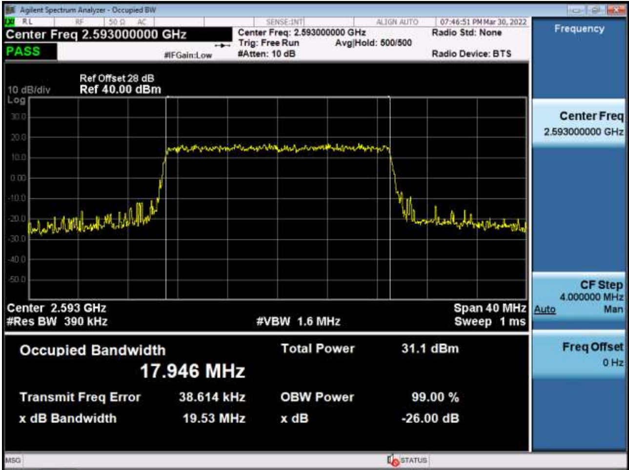
Occupied Bandwidth Plot (20 MHz Ch.40620 64-QAM RB 100)
