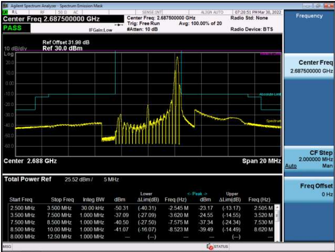
High Channel Edge Plot (5 MHz Ch.41565 QPSK RB 1, Offset 24)
