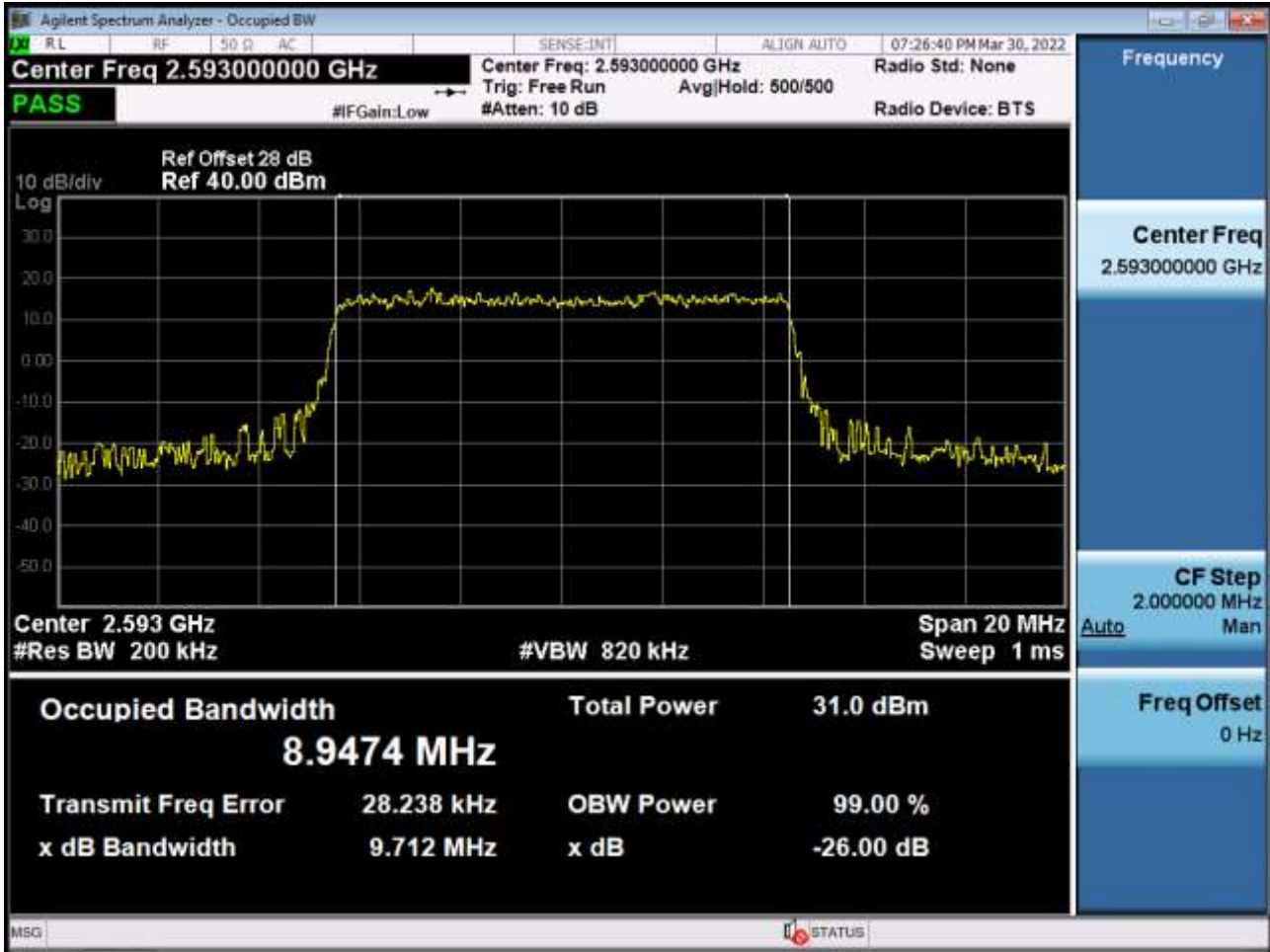
Occupied Bandwidth Plot (10 MHz Ch.40620 64-QAM RB 50)
