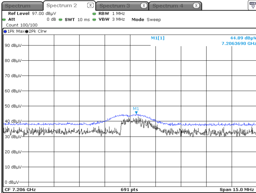
Radiated Spurious Emissions plot – Average & Peak Result ( \pi/4 DQPSK, Ch. 0 3rd Harmonic, Y-V)
