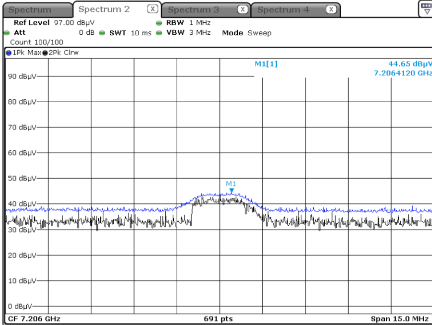
Radiated Spurious Emissions plot – Average & Peak Result (GFSK, Ch. 0 3rd Harmonic, Y-V)
