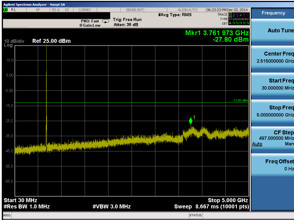
Plot 6-33. Conducted Spurious Plot (Band 17 – 10.0MHz QPSK – RB Size 1, RB Offset 0 – High Channel)
