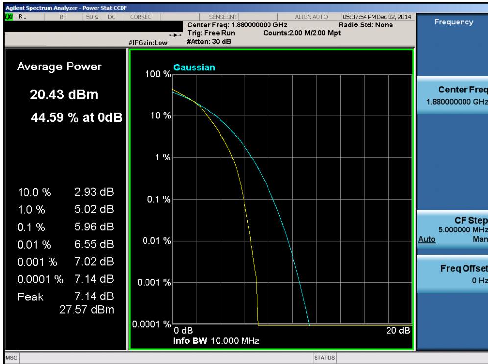
Plot 6-110. PAR Plot (Band 2 – 10.0MHz 16-QAM – RB Size 50)
