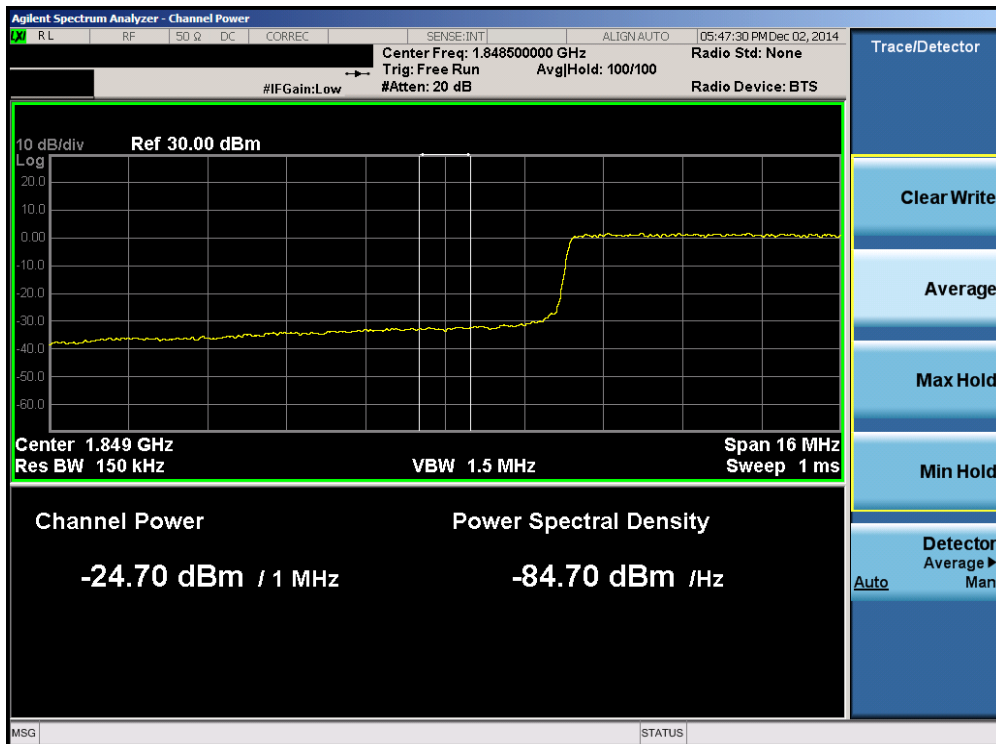
Plot 6-100. Lower Extended Band Edge Plot (Band 2 – 20.0MHz QPSK – RB Size 100)
