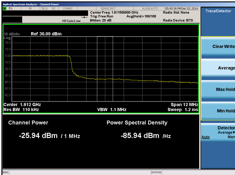
Plot 6-98. Upper Extended Band Edge Plot (Band 2 – 15.0MHz QPSK – RB Size 75)
