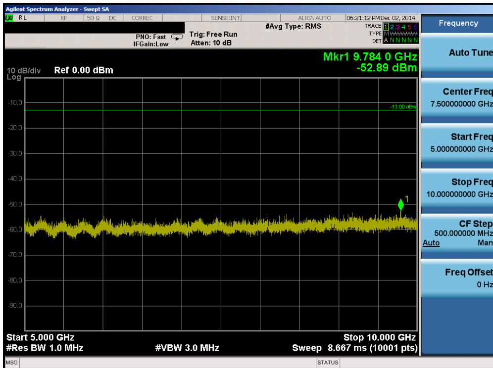
Plot 6-32. Conducted Spurious Plot (Band 17 – 10.0MHz QPSK – RB Size 1, RB Offset 0 – Mid Channel)
