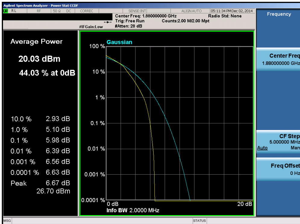
Plot 6-104. PAR Plot (Band 2 – 1.4MHz 16-QAM – RB Size 6)
