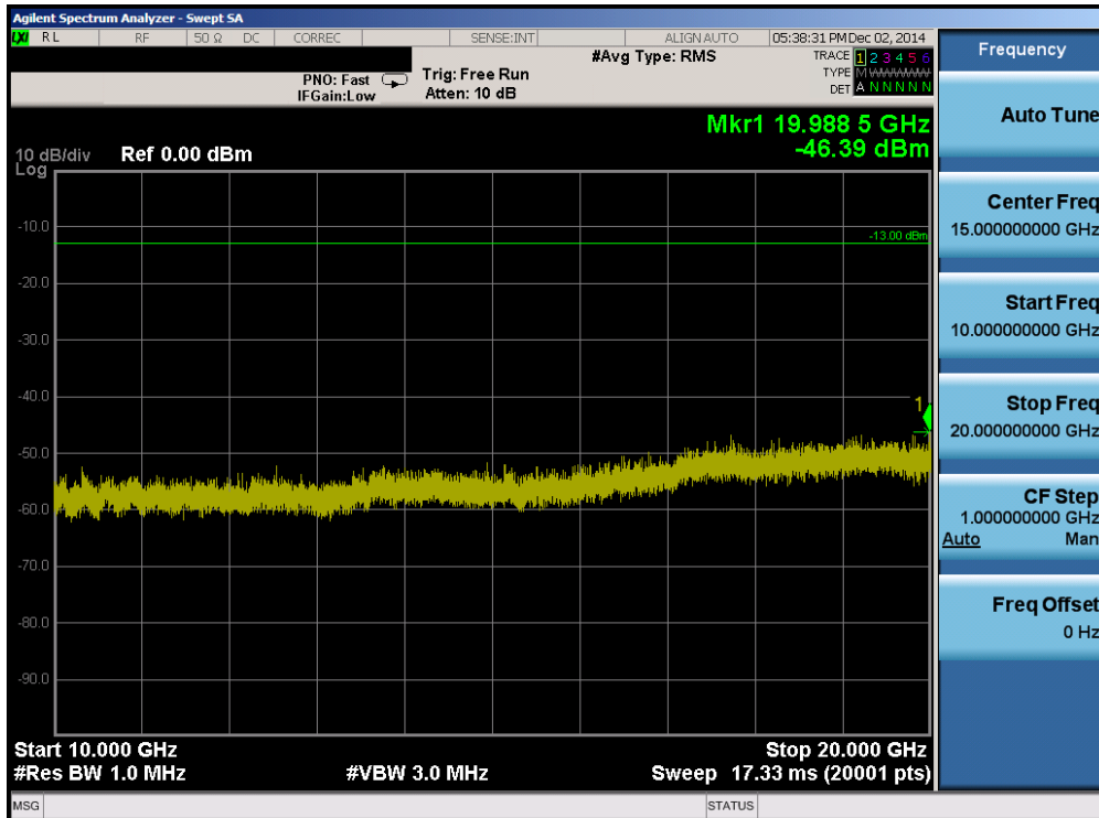
Plot 6-44. Conducted Spurious Plot (Band 2 – 10.0MHz QPSK – RB Size 1, RB Offset 0 – Mid Channel)
