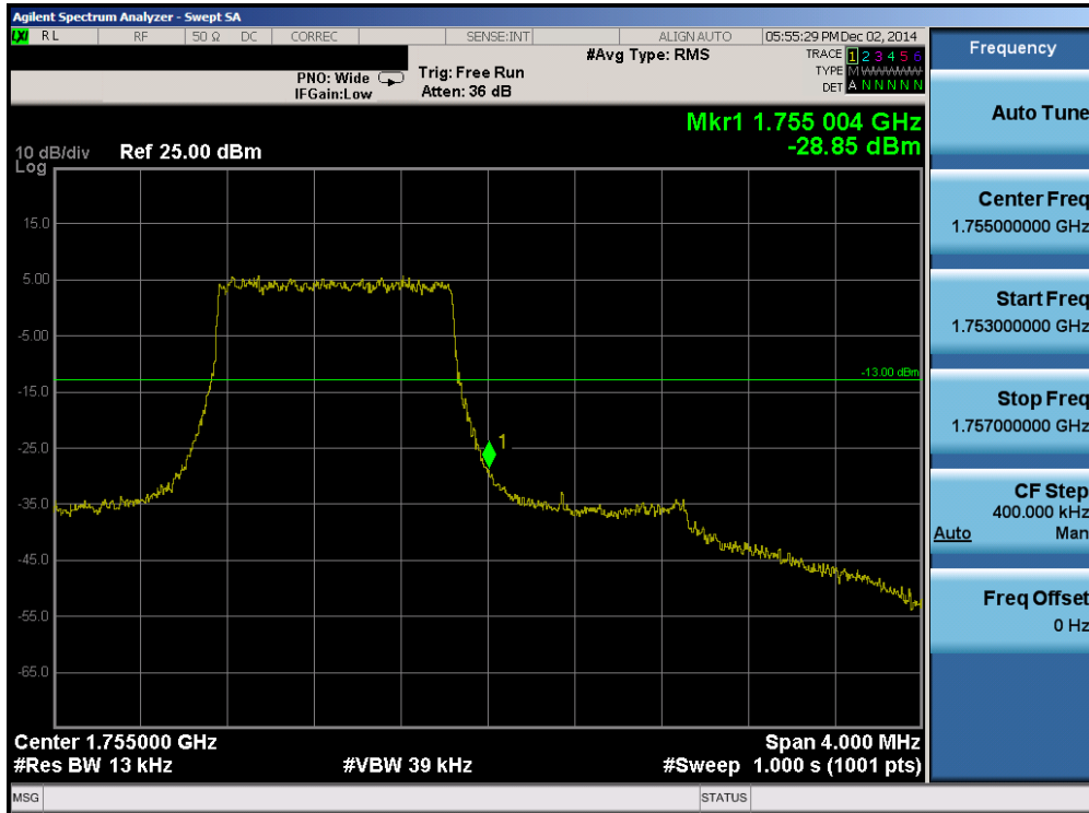
Plot 6-57. Upper Band Edge Plot (Band 4 – 1.4MHz QPSK – RB Size 6)
