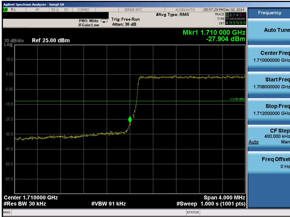
Plot 6-59. Lower Band Edge Plot (Band 4 – 3.0MHz QPSK – RB Size 15)
