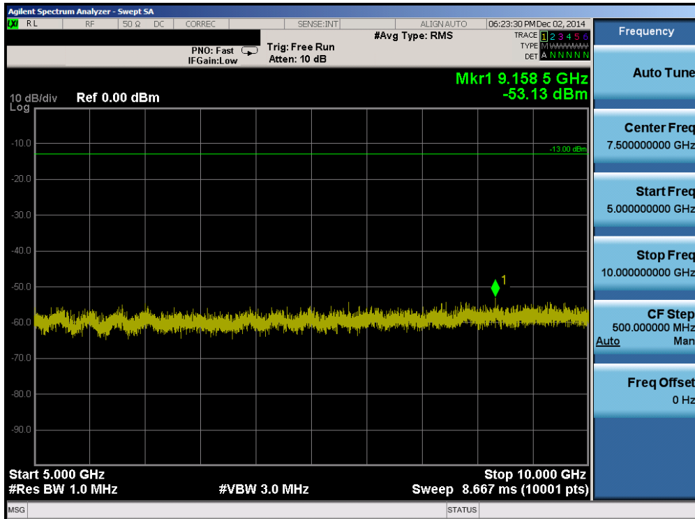
Plot 6-34. Conducted Spurious Plot (Band 4 – 5.0MHz QPSK – RB Size 1, RB Offset 0 – High Channel)
