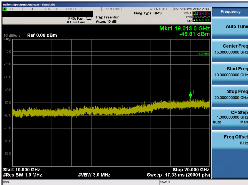
Plot 6-42. Conducted Spurious Plot (Band 2 – 10.0MHz QPSK – RB Size 1, RB Offset 0 – Low Channel)
