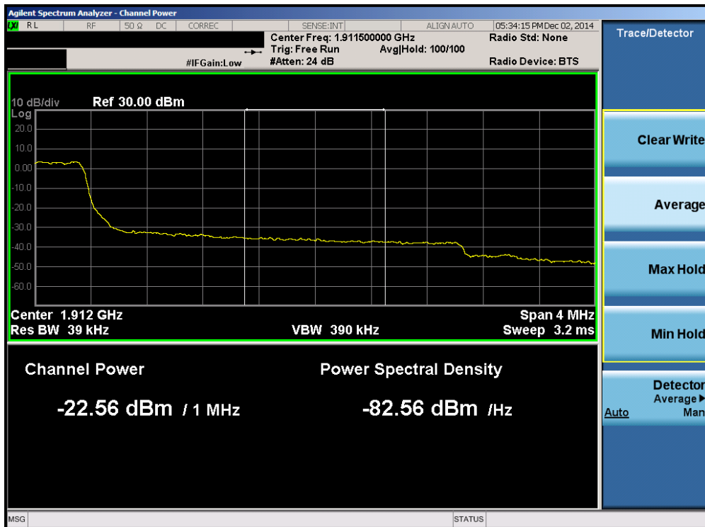
Plot 6-86. Upper Extended Band Edge Plot (Band 2 – 3.0MHz QPSK – RB Size 15)
