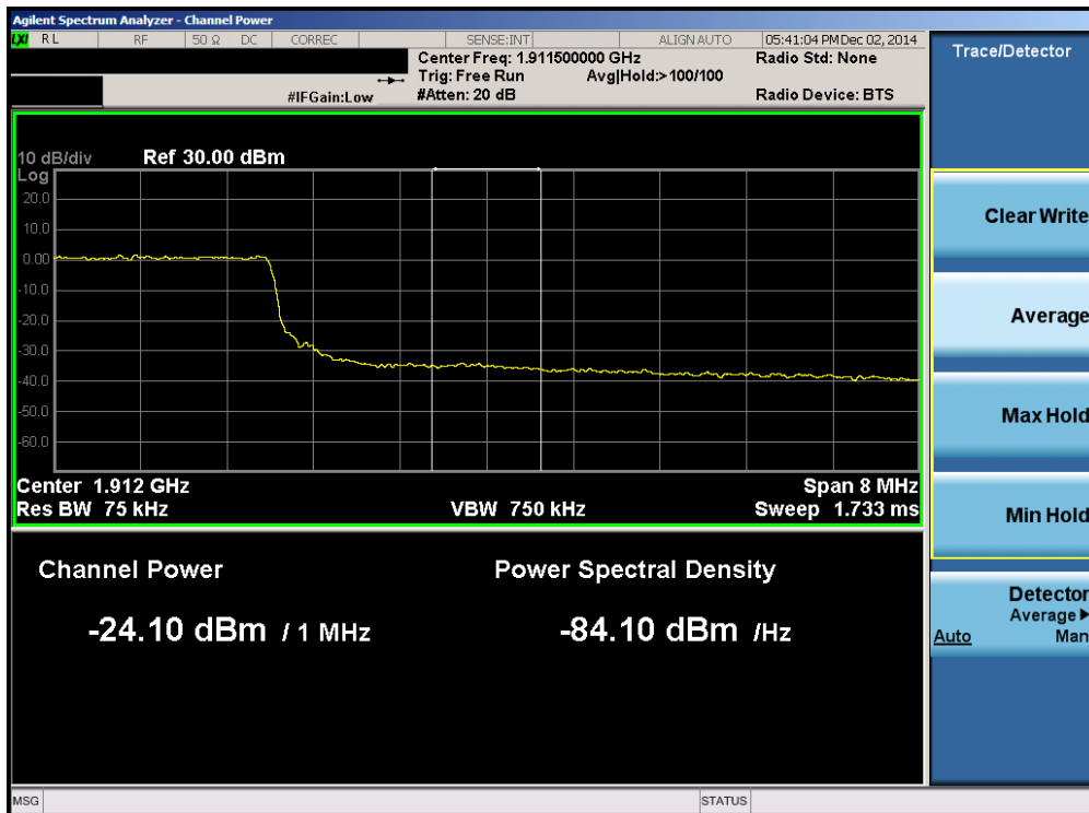
Plot 6-94. Upper Extended Band Edge Plot (Band 2 – 10.0MHz QPSK – RB Size 50)
