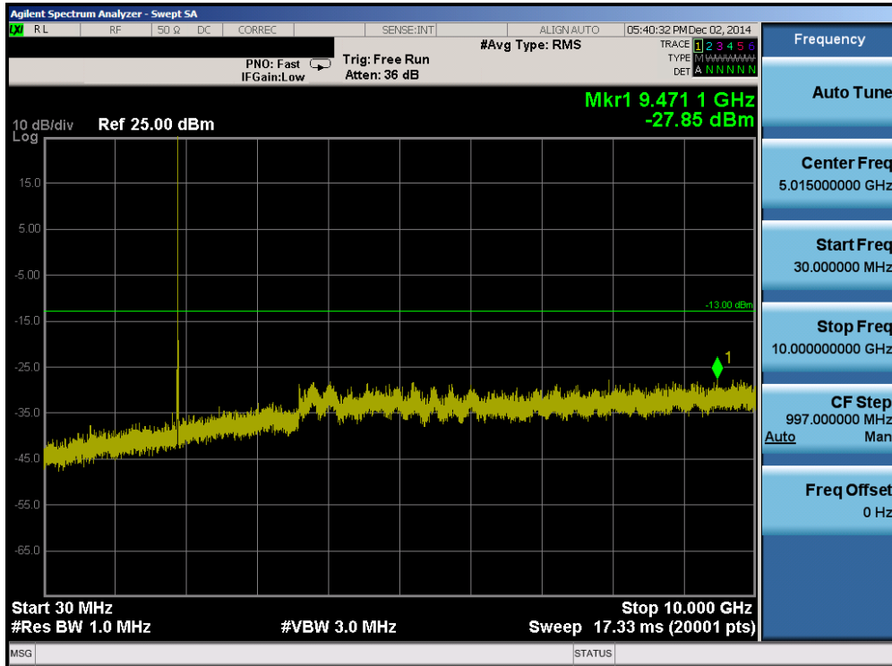
Plot 6-45. Conducted Spurious Plot (Band 2 – 10.0MHz QPSK – RB Size 1, RB Offset 0 – High Channel)
