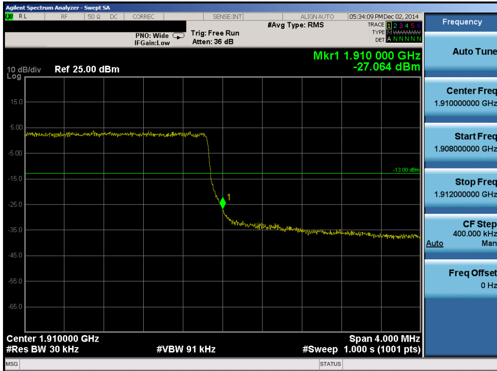
Plot 6-85. Upper Band Edge Plot (Band 2 – 3.0MHz QPSK – RB Size 15)
