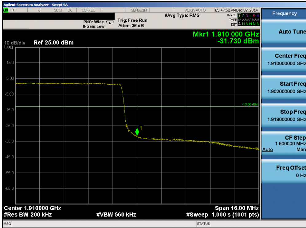
Plot 6-101. Upper Band Edge Plot (Band 2 – 20.0MHz QPSK – RB Size 100)
