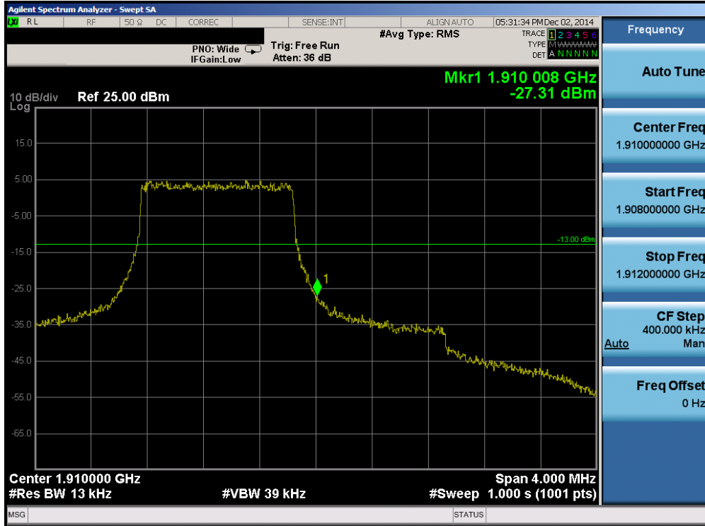
Plot 6-81. Upper Band Edge Plot (Band 2 – 1.4MHz QPSK – RB Size 6)
