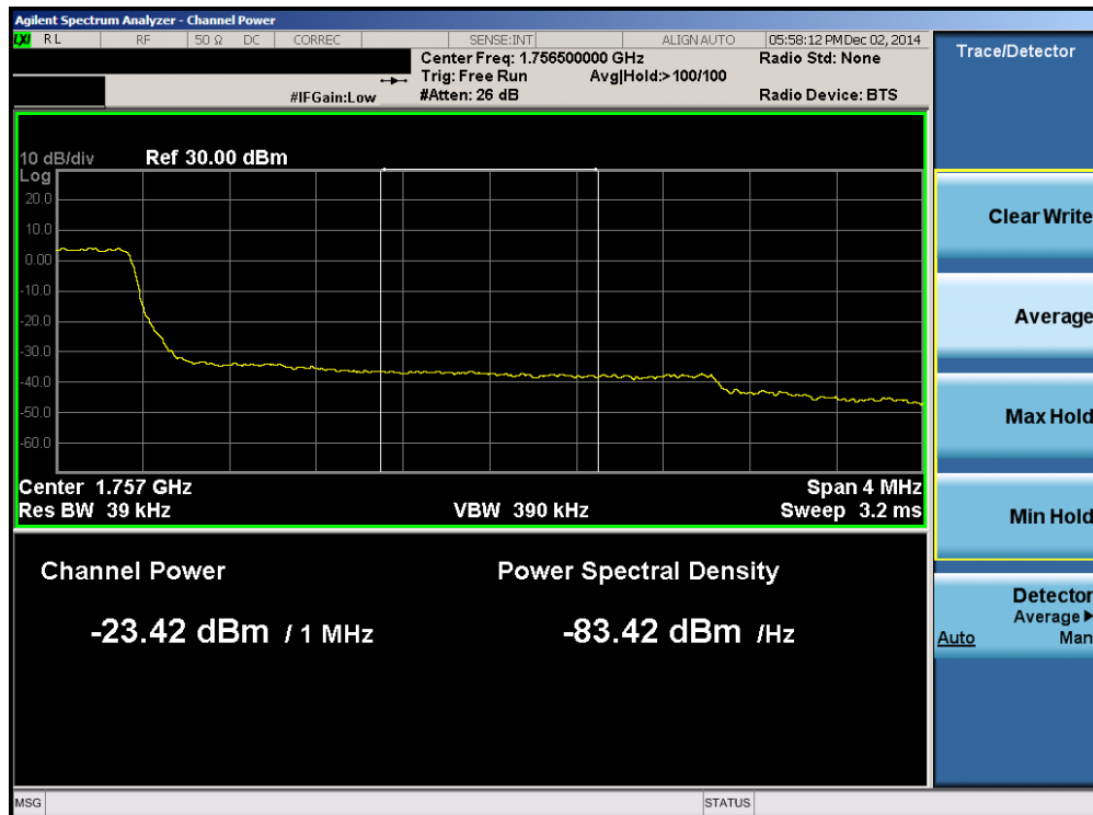
Plot 6-62. Upper Extended Band Edge Plot (Band 4 – 3.0MHz QPSK – RB Size 15)
