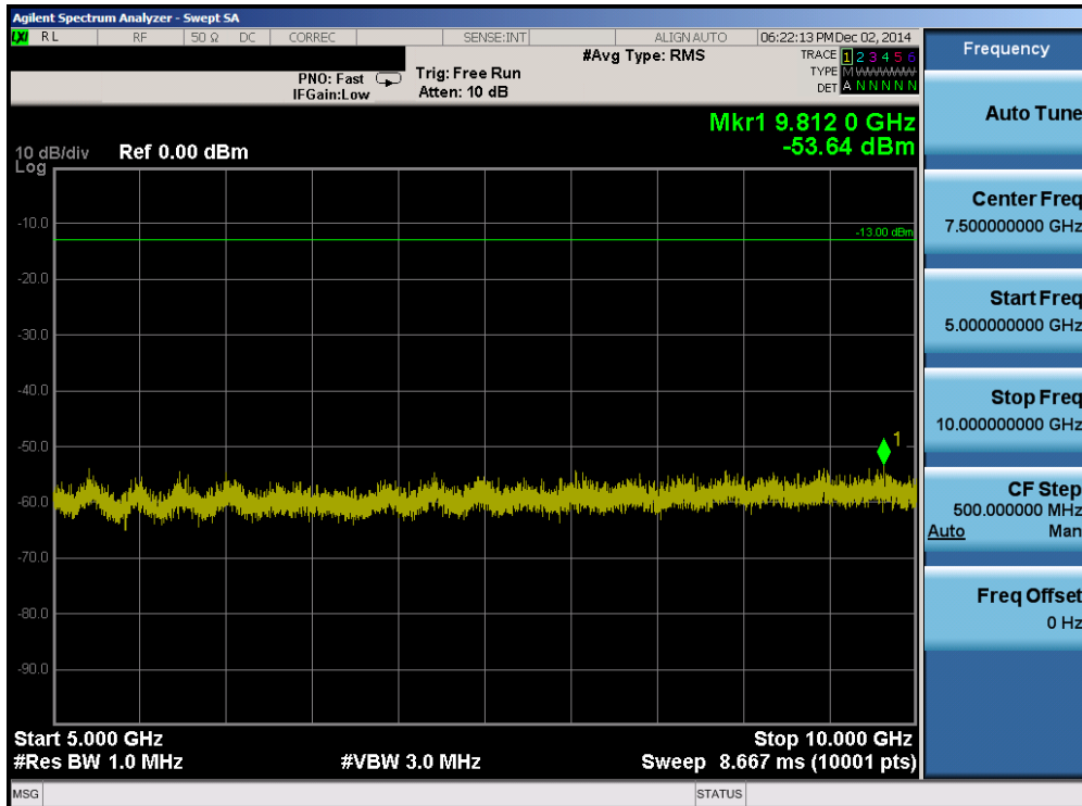
Plot 6-30. Conducted Spurious Plot (Band 17 – 10.0MHz QPSK – RB Size 1, RB Offset 0 – Low Channel)
