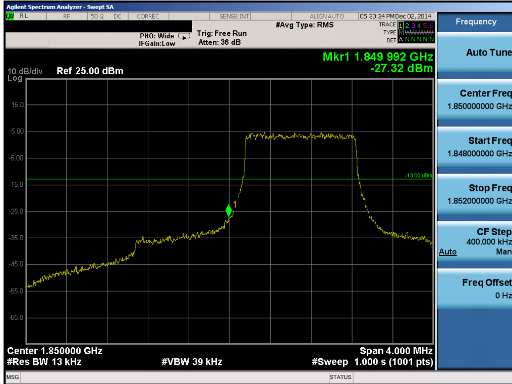
Plot 6-79. Lower Band Edge Plot (Band 2 – 1.4MHz QPSK – RB Size 6)
