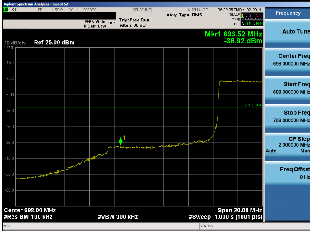
Plot 6-51. Lower Band Edge Plot (Band 17 – 10.0MHz QPSK – RB Size 50)
