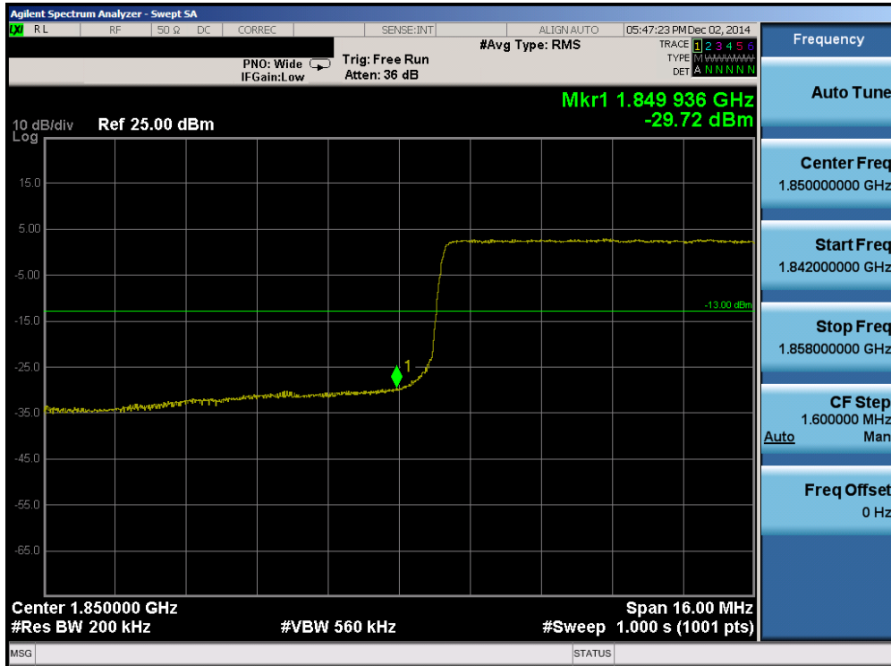
Plot 6-99. Lower Band Edge Plot (Band 2 – 20.0MHz QPSK – RB Size 100)
