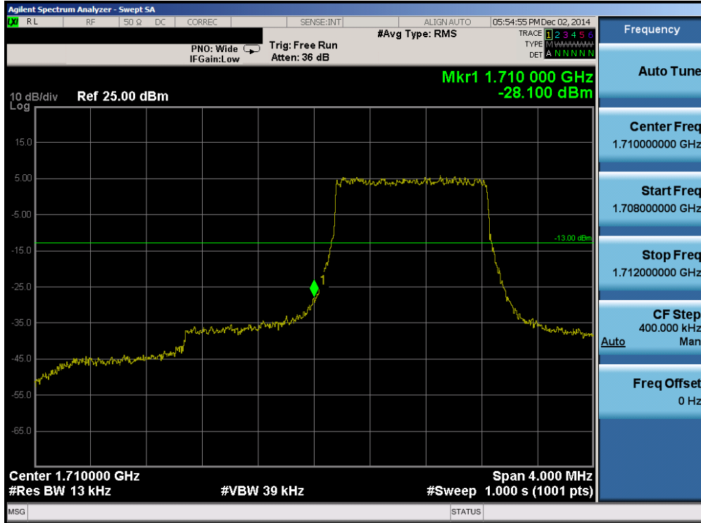
Plot 6-55. Lower Band Edge Plot (Band 4 – 1.4MHz QPSK – RB Size 6)
