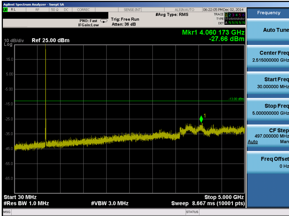
Plot 6-29. Conducted Spurious Plot (Band 17 – 10.0MHz QPSK – RB Size 1, RB Offset 0– Low Channel)
