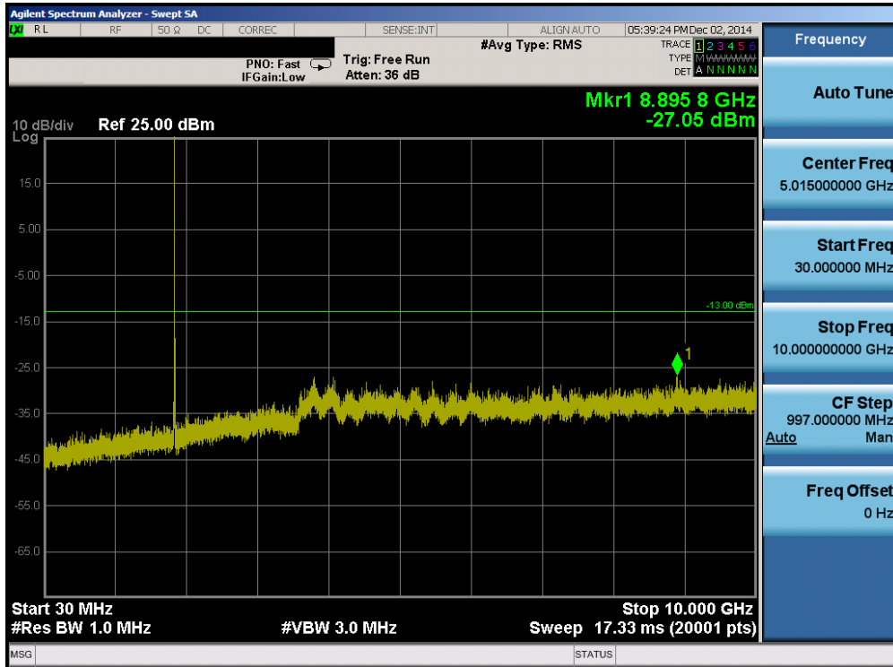
Plot 6-41. Conducted Spurious Plot (Band 2 – 10.0MHz QPSK – RB Size 1, RB Offset 0– Low Channel)
