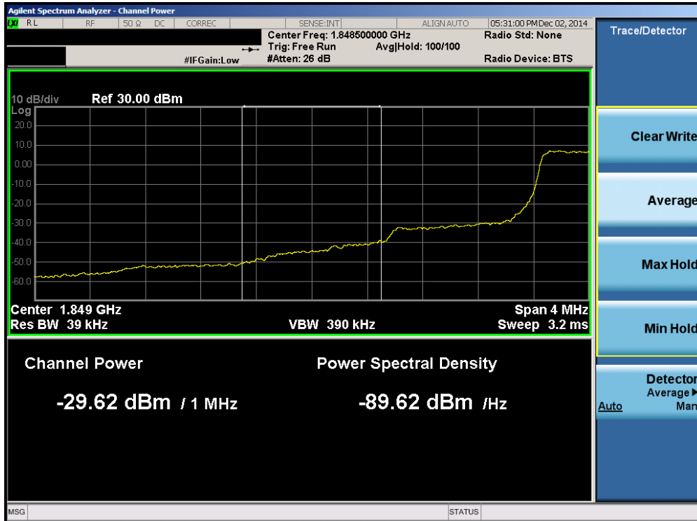
Plot 6-80. Lower Extended Band Edge Plot (Band 2 – 1.4MHz QPSK – RB Size 6)
