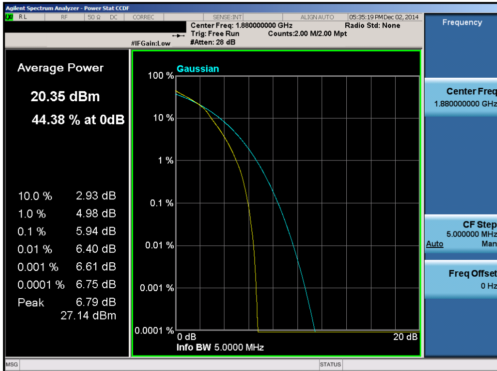
Plot 6-108. PAR Plot (Band 2 – 5.0MHz 16-QAM – RB Size 25)
