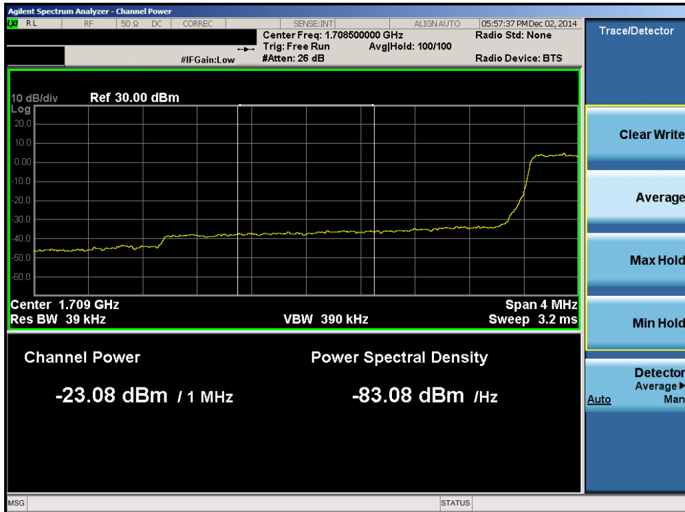
Plot 6-60. Lower Extended Band Edge Plot (Band 4 – 3.0MHz QPSK – RB Size 15)
