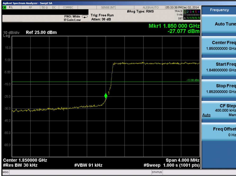
Plot 6-83. Lower Band Edge Plot (Band 2 – 3.0MHz QPSK – RB Size 15)
