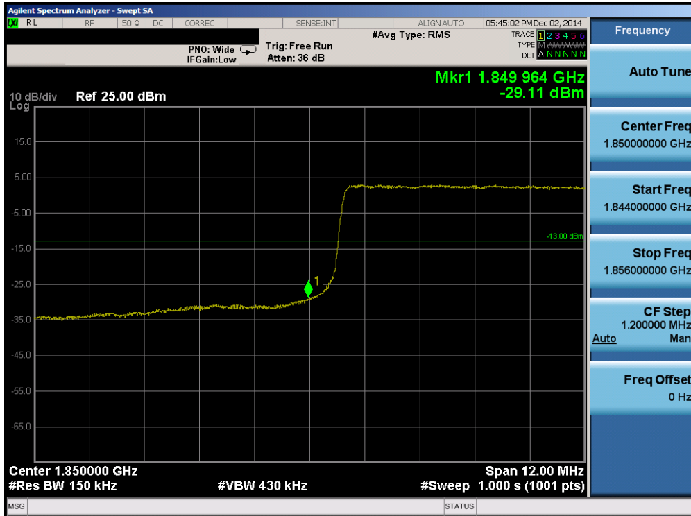
Plot 6-95. Lower Band Edge Plot (Band 2 – 15.0MHz QPSK – RB Size 75)
