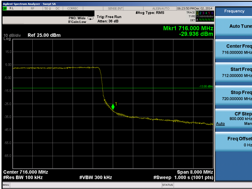
Plot 6-53. Upper Band Edge Plot (Band 17 – 10.0MHz QPSK – RB Size 50)
