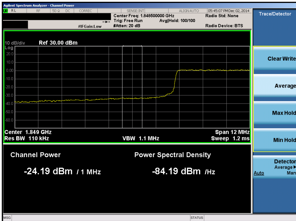
Plot 6-96. Lower Extended Band Edge Plot (Band 2 – 15.0MHz QPSK – RB Size 75)
