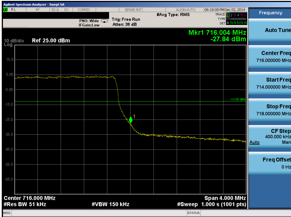
Plot 6-49. Upper Band Edge Plot (Band 17 – 5.0MHz QPSK – RB Size 25)
