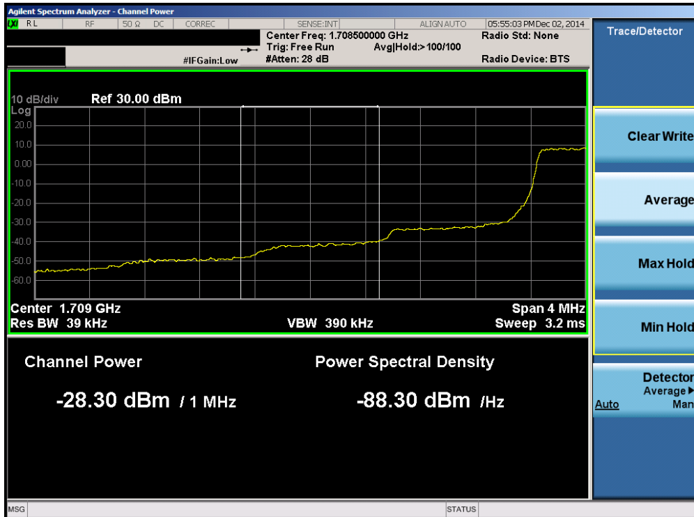
Plot 6-56. Lower Extended Band Edge Plot (Band 4 – 1.4MHz QPSK – RB Size 6)
