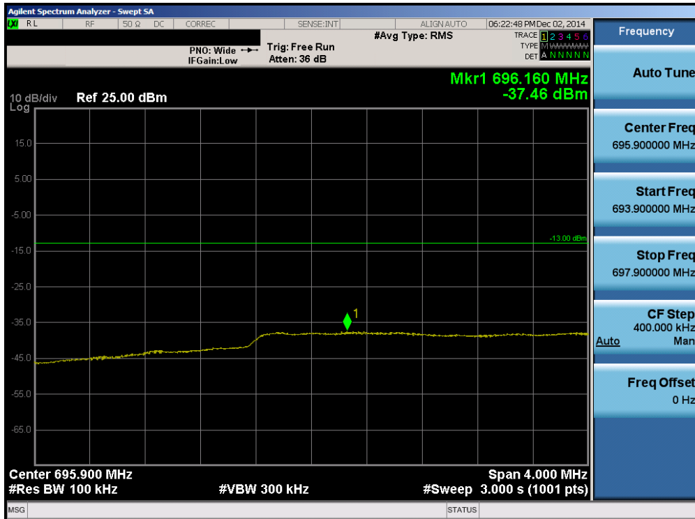
Plot 6-52. Lower Extended Band Edge Plot (Band 17 – 10.0MHz QPSK – RB Size 50)
