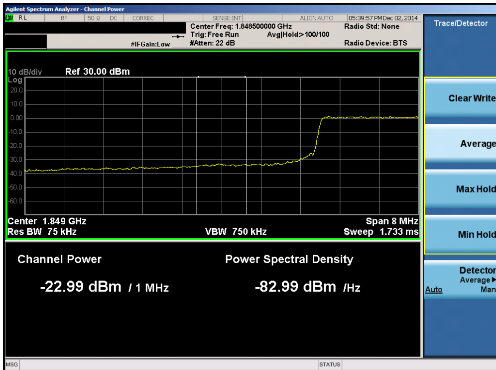
Plot 6-92. Lower Extended Band Edge Plot (Band 2 – 10.0MHz QPSK – RB Size 50)
