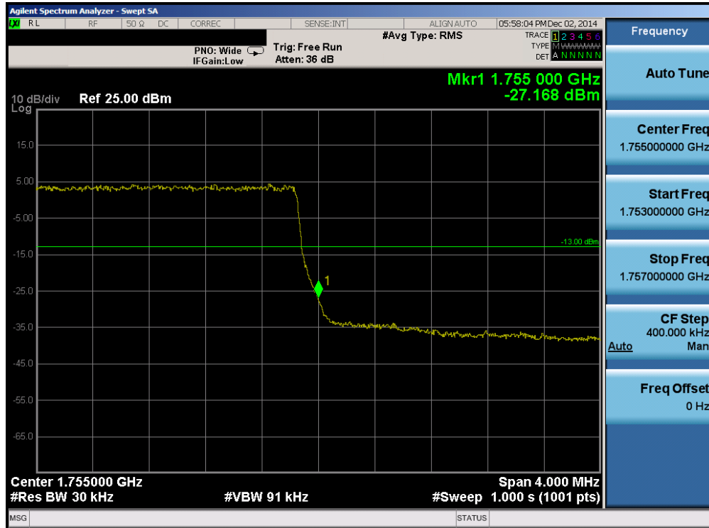
Plot 6-61. Upper Band Edge Plot (Band 4 – 3.0MHz QPSK – RB Size 15)
