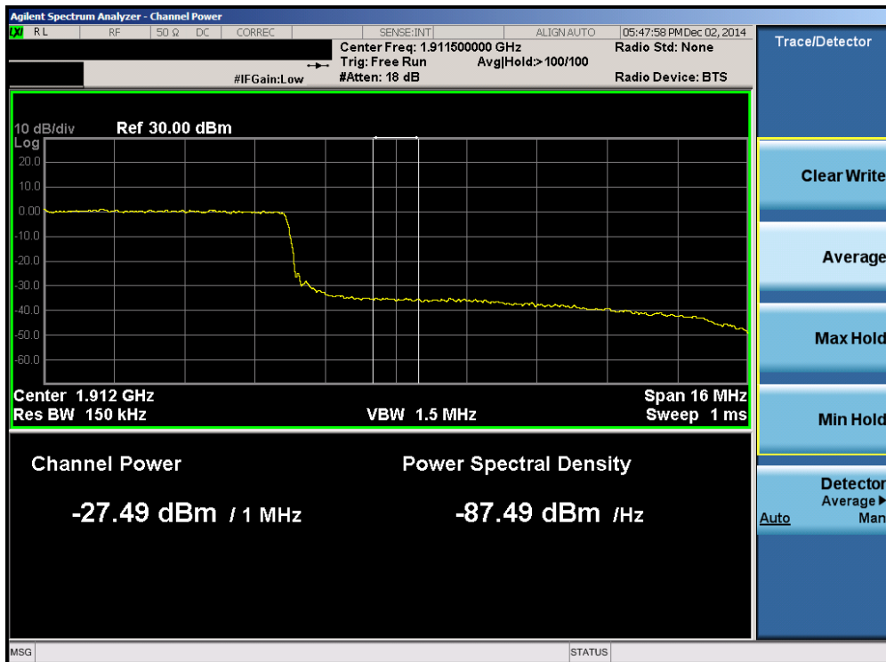
Plot 6-102. Upper Extended Band Edge Plot (Band 2 – 20.0MHz QPSK – RB Size 100)
