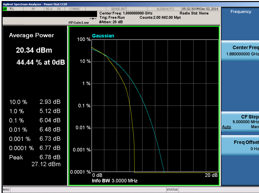
Plot 6-106. PAR Plot (Band 2 – 3.0MHz 16-QAM – RB Size 15)
