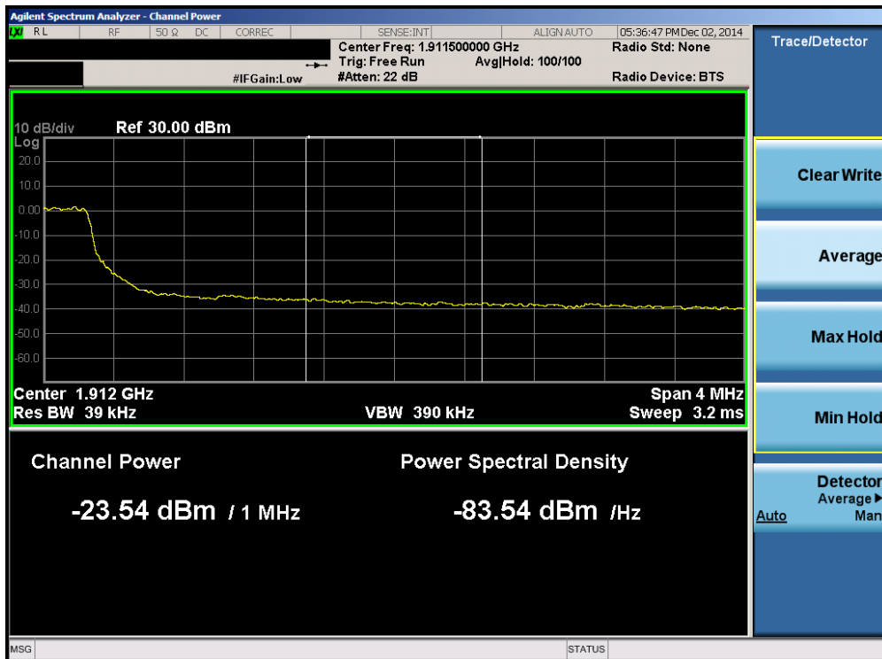
Plot 6-90. Upper Extended Band Edge Plot (Band 2 – 5.0MHz QPSK – RB Size 25)
