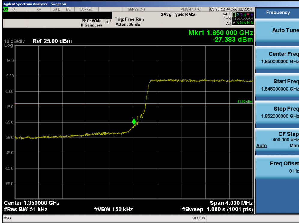
Plot 6-87. Lower Band Edge Plot (Band 2 – 5.0MHz QPSK – RB Size 25)
