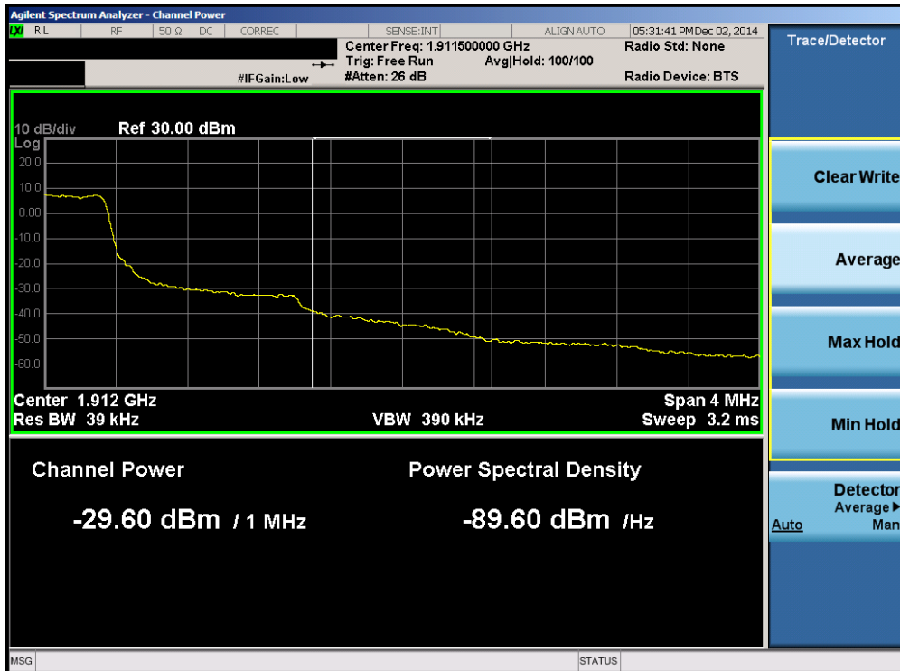
Plot 6-82. Upper Extended Band Edge Plot (Band 2 – 1.4MHz QPSK – RB Size 6)
