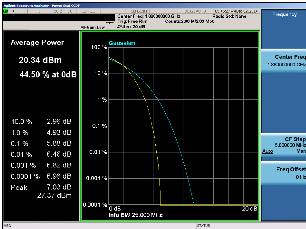
Plot 6-114. PAR Plot (Band 2 – 20.0MHz 16-QAM – RB Size 100)
