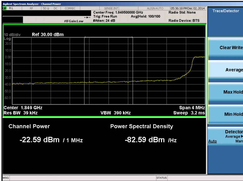
Plot 6-88. Lower Extended Band Edge Plot (Band 2 – 5.0MHz QPSK – RB Size 25)
