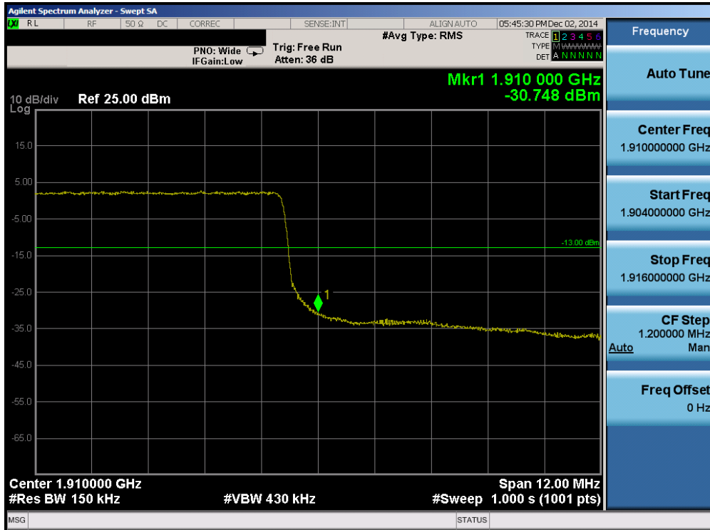
Plot 6-97. Upper Band Edge Plot (Band 2 – 15.0MHz QPSK – RB Size 75)
