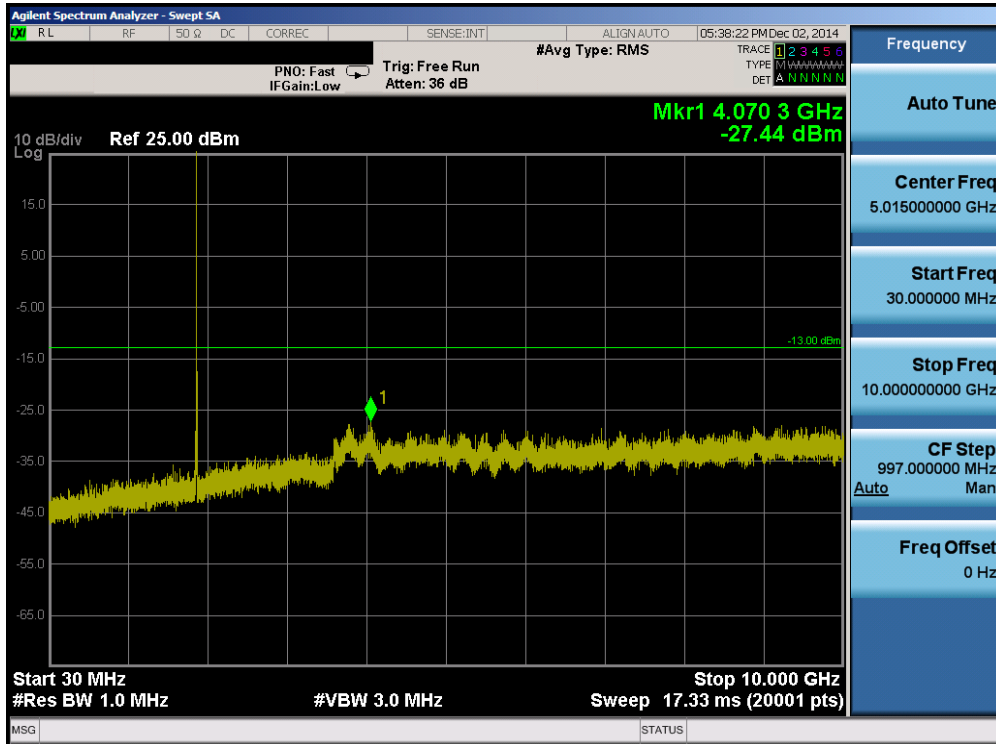
Plot 6-43. Conducted Spurious Plot (Band 2 – 10.0MHz QPSK – RB Size 1, RB Offset 0 – Mid Channel)
