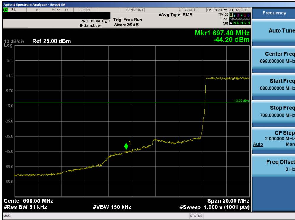
Plot 6-47. Lower Band Edge Plot (Band 17 – 5.0MHz QPSK – RB Size 25)
