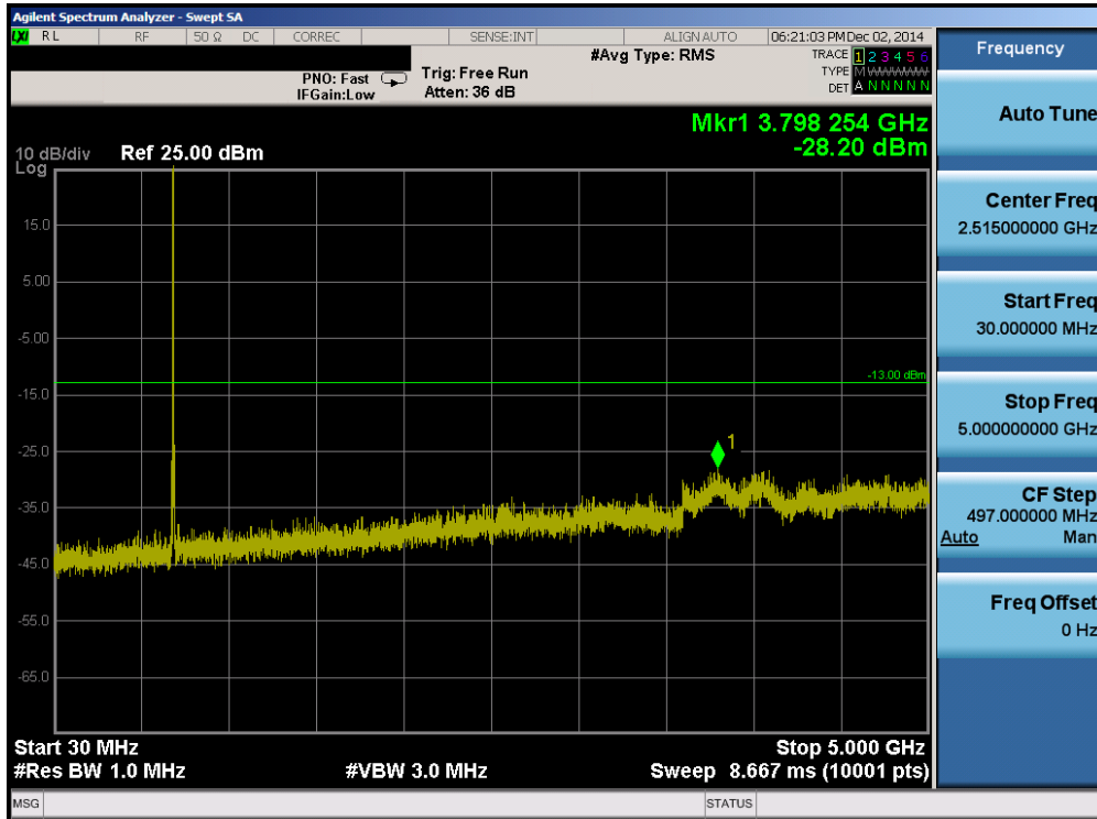
Plot 6-31. Conducted Spurious Plot (Band 17 – 10.0MHz QPSK – RB Size 1, RB Offset 0 – Mid Channel)
