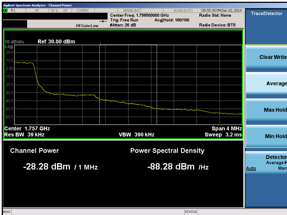
Plot 6-58. Upper Extended Band Edge Plot (Band 4 – 1.4MHz QPSK – RB Size 6)
