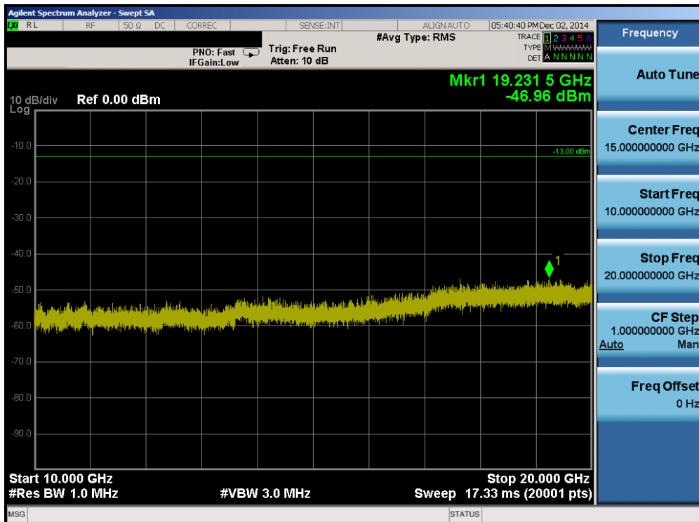
Plot 6-46. Conducted Spurious Plot (Band 2 – 10.0MHz QPSK – RB Size 1, RB Offset 0 – High Channel)
