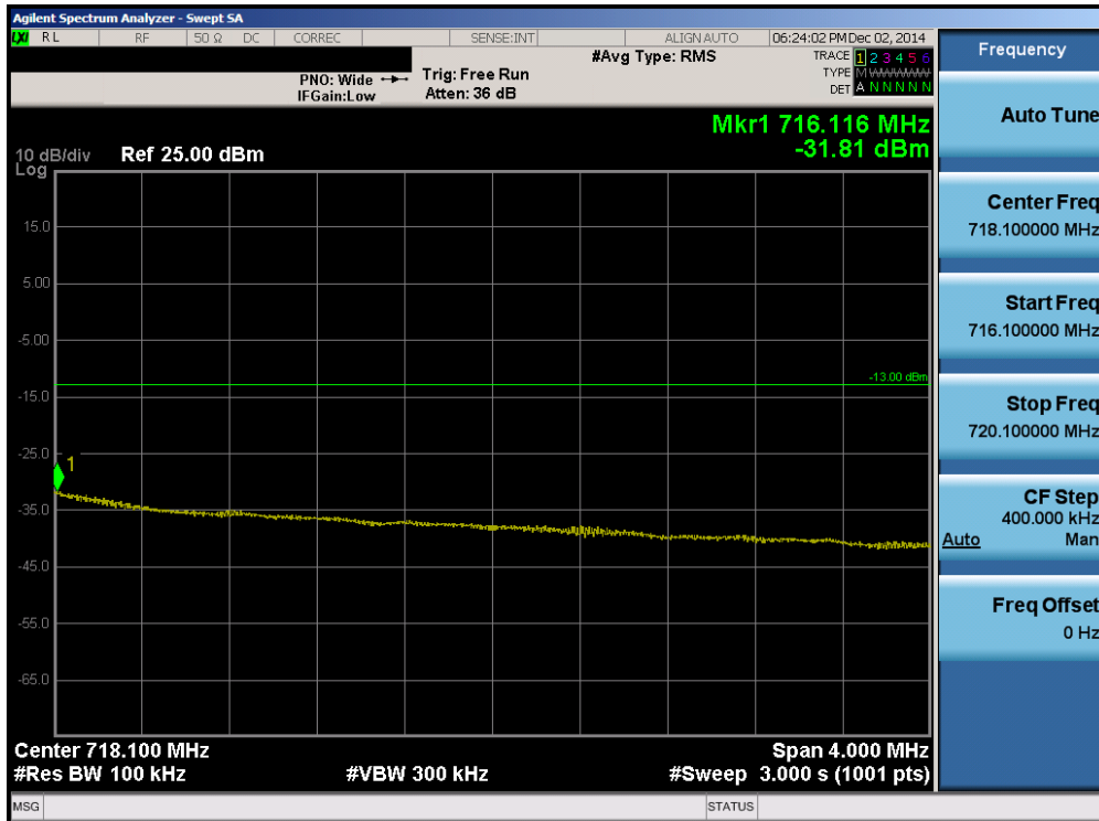
Plot 6-54. Upper Extended Band Edge Plot (Band 17 – 10.0MHz QPSK – RB Size 50)
