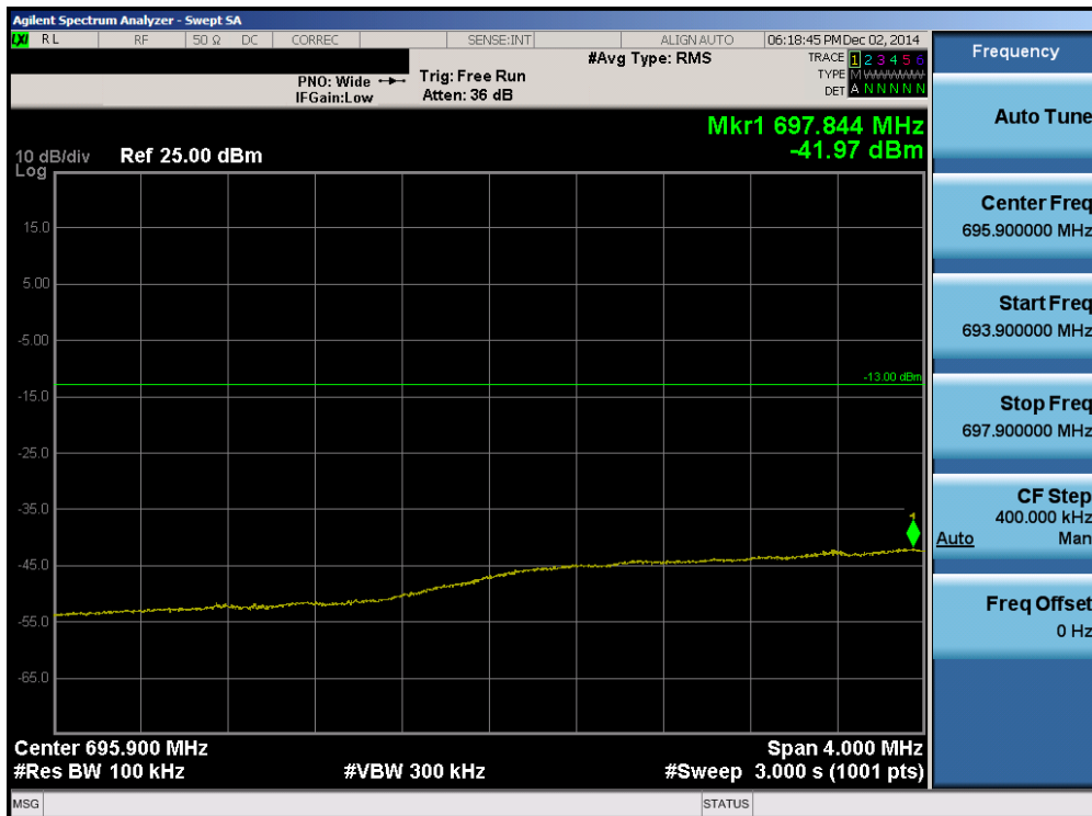
Plot 6-48. Lower Extended Band Edge Plot (Band 17 – 5.0MHz QPSK – RB Size 25)
