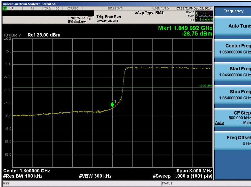
Plot 6-91. Lower Band Edge Plot (Band 2 – 10.0MHz QPSK – RB Size 50)
