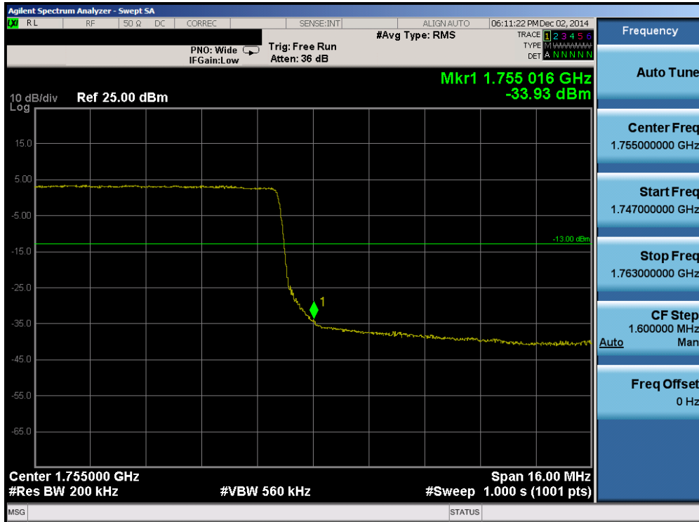
Plot 6-77. Upper Band Edge Plot (Band 4 – 20.0MHz QPSK – RB Size 100)
