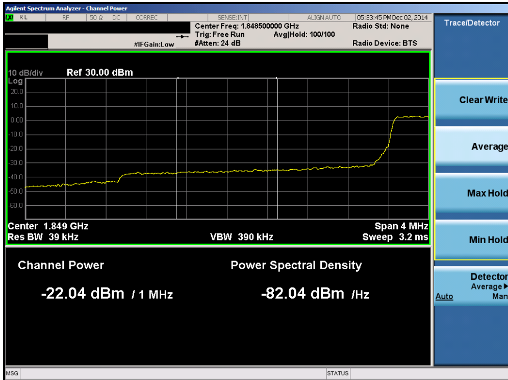
Plot 6-84. Lower Extended Band Edge Plot (Band 2 – 3.0MHz QPSK – RB Size 15)
