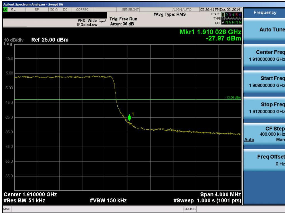
Plot 6-89. Upper Band Edge Plot (Band 2 – 5.0MHz QPSK – RB Size 25)
