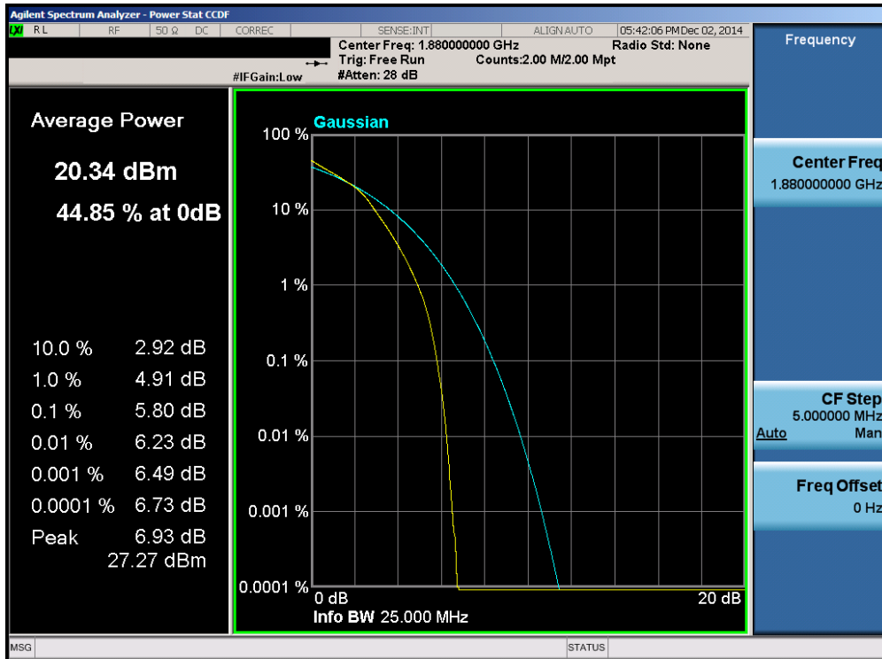
Plot 6-112. PAR Plot (Band 2 – 15.0MHz 16-QAM – RB Size 75)
