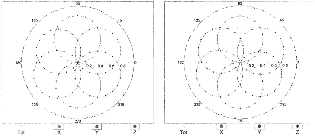
f=600 MHz,TEM
