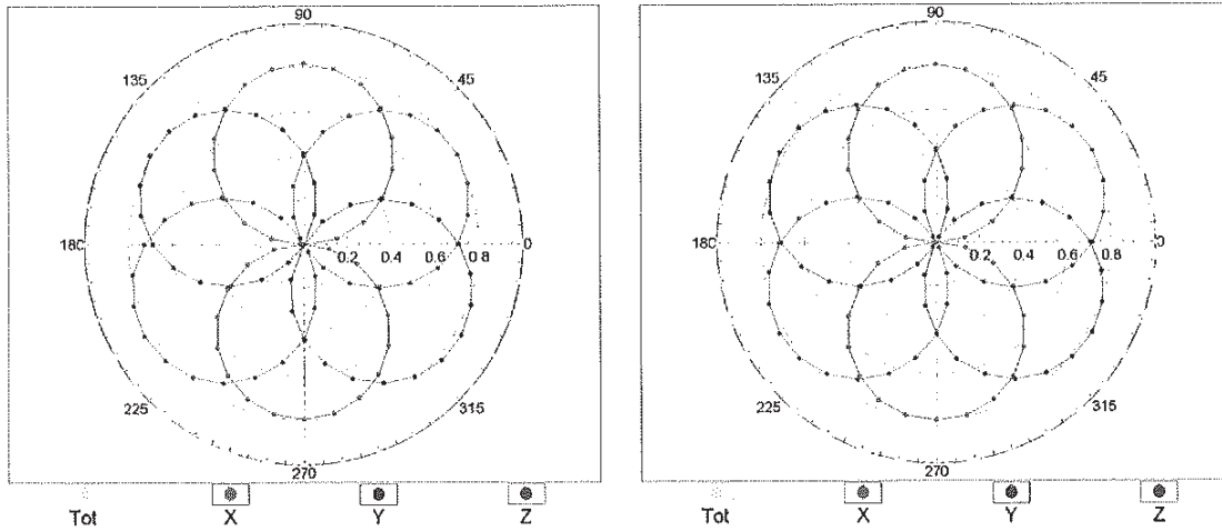
f=600 MHz,TEM
