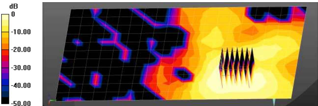
0 dB = 0.321 W/kg = -4.93 dBW/kg
