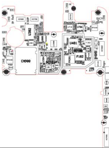
Rear of PCB
