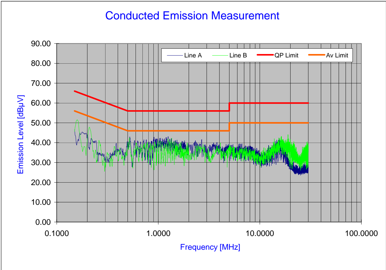
Plot 6-75. Line Conducted Plot with 802.11a (UNII Band 2C)
