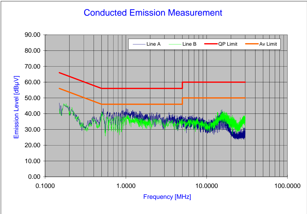
Plot 6-74. Line Conducted Plot with 802.11a (UNII Band 2A)
