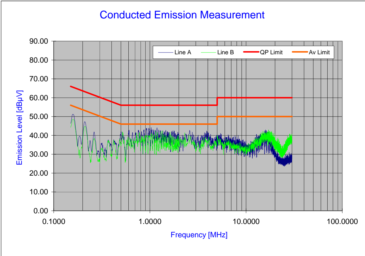
Plot 6-73. Line Conducted Plot with 802.11a (UNII Band 1)
