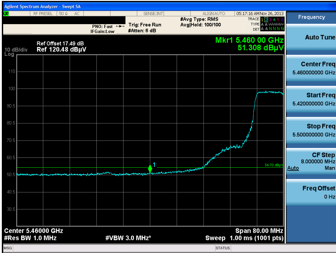
Plot 6-63. Radiated Restricted Lower Band Edge Plot (Average – UNII Band 2C)
