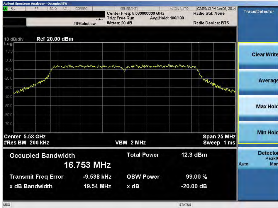
Plot 6-27. 20dB Bandwidth Plot (20MHz BW 802.11a (UNII Band 2B) – Ch. 116)
