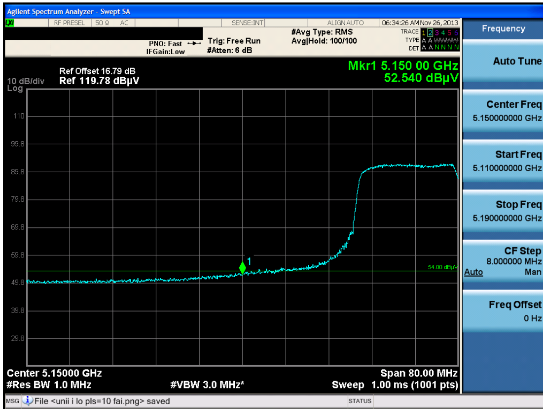
Plot 6-66. Radiated Restricted Lower Band Edge Plot (Average – UNII Band 1)
