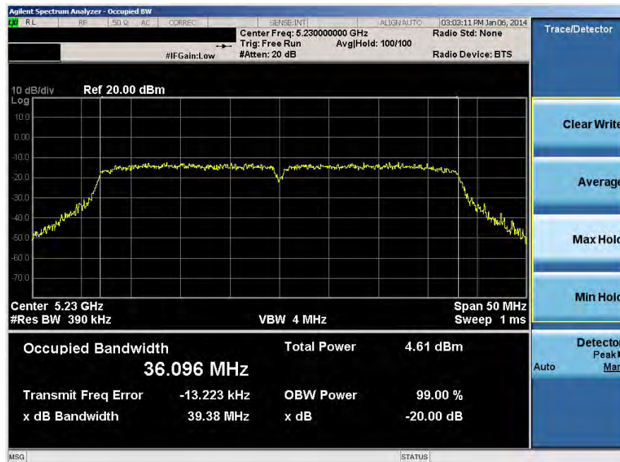
Plot 6-29. 20dB Bandwidth Plot (40MHz BW 802.11n (UNII Band 2A) – Ch. 46)
