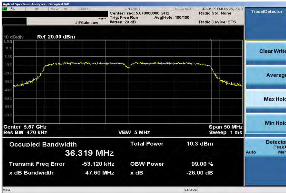
Plot 6-25. 26dB Bandwidth Plot (40MHz BW 802.11n (UNII Band 3) – Ch. 134)
