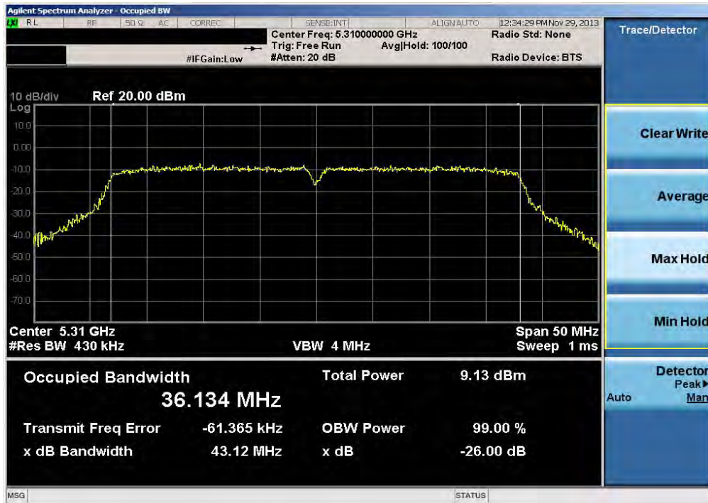
Plot 6-16. 26dB Bandwidth Plot (40MHz BW 802.11n (UNII Band 2A) – Ch. 62)
