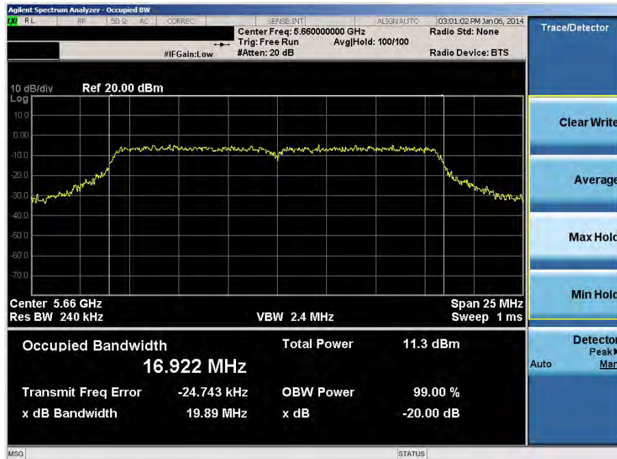
Plot 6-28. 20dB Bandwidth Plot (20MHz BW 802.11n (UNII Band 2A) – Ch. 132)
