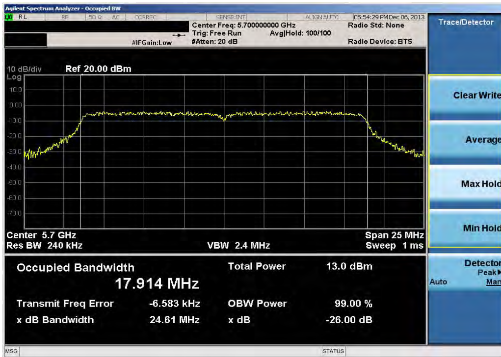
Plot 6-22. 26dB Bandwidth Plot (20MHz BW 802.11n (UNII Band 2C) – Ch. 140)
