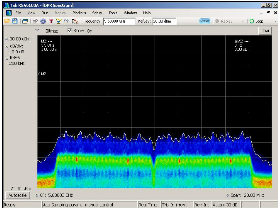
Figure 6-2. Real-Time Spectrum Display, WLAN Traffic (Streaming Video)
