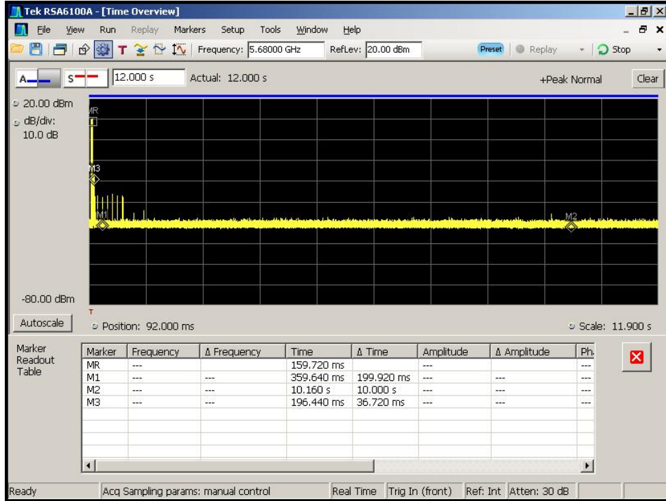
Figure 6-3. Channel Move Time (< 10sec)
