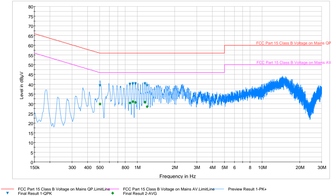
Plot 6-77. Line Conducted Plot with 802.11a UNII Band 2A (N)
