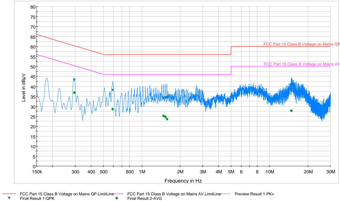
Plot 6-74. Line Conducted Plot with 802.11a UNII Band 3 (N)
