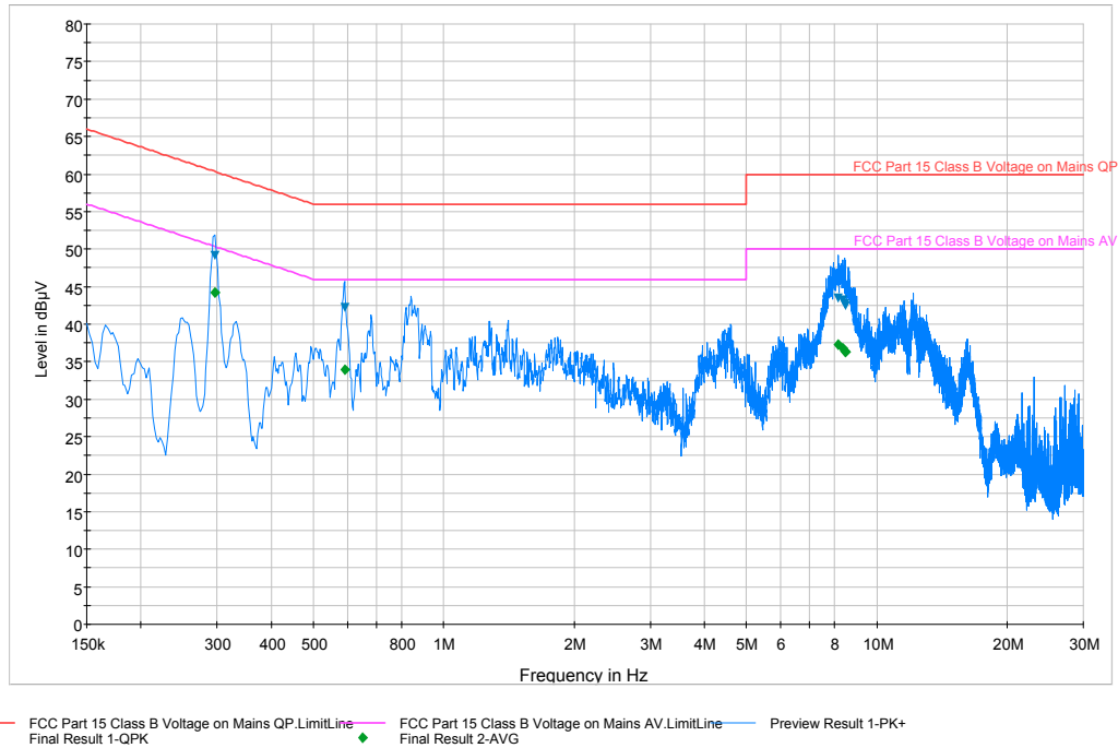
Plot 6-68. Line Conducted Plot with 802.11a (N)
