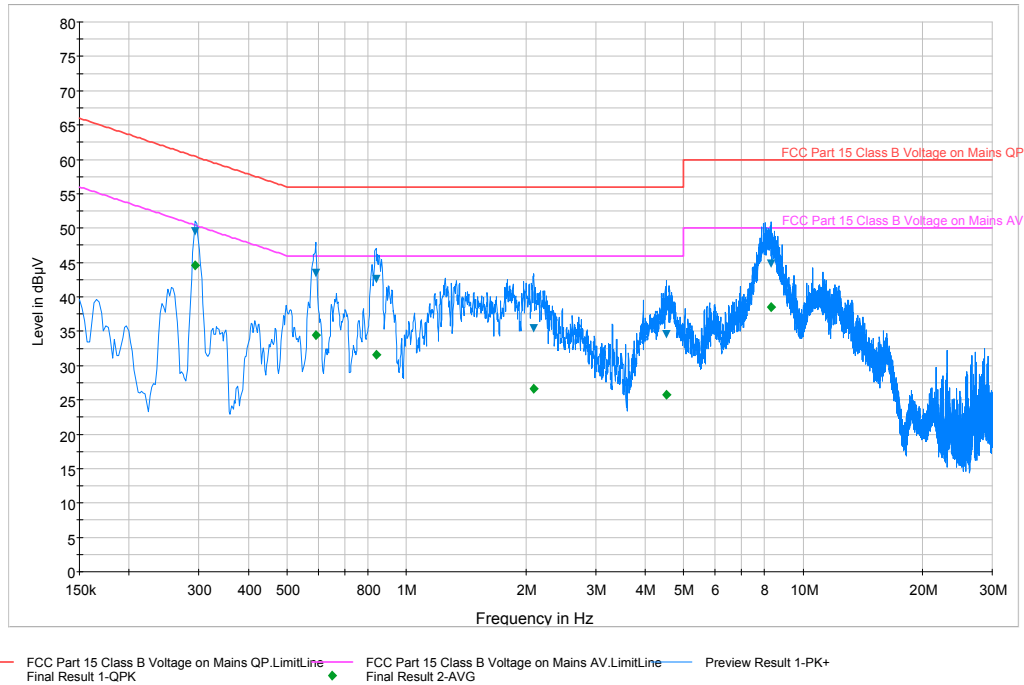
Plot 6-67. Line Conducted Plot with 802.11a (L1)
