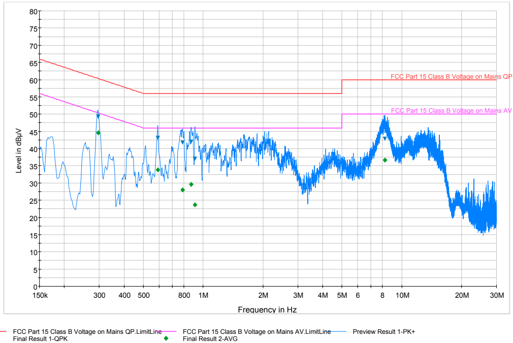
Plot 6-65. Line Conducted Plot with 802.11b (L1)
