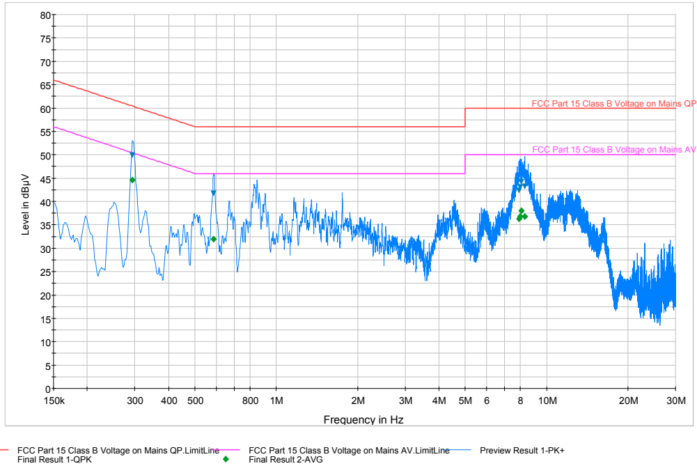
Plot 6-66. Line Conducted Plot with 802.11b (N)
