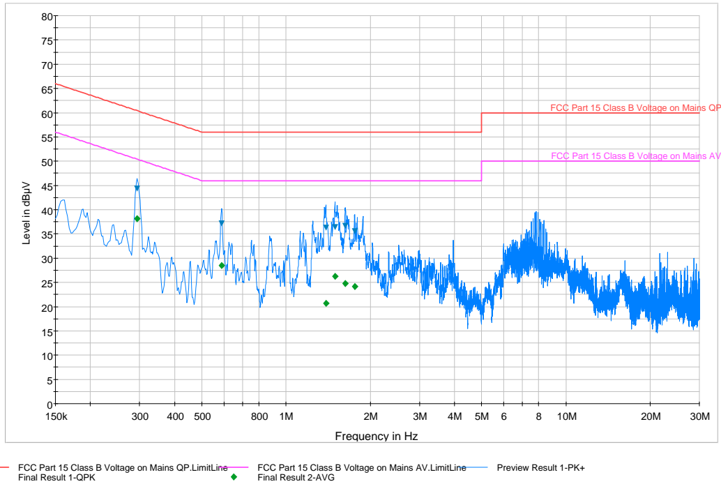
Plot 6-71. Line Conducted Plot with 802.11a UNII Band 1 (N)
