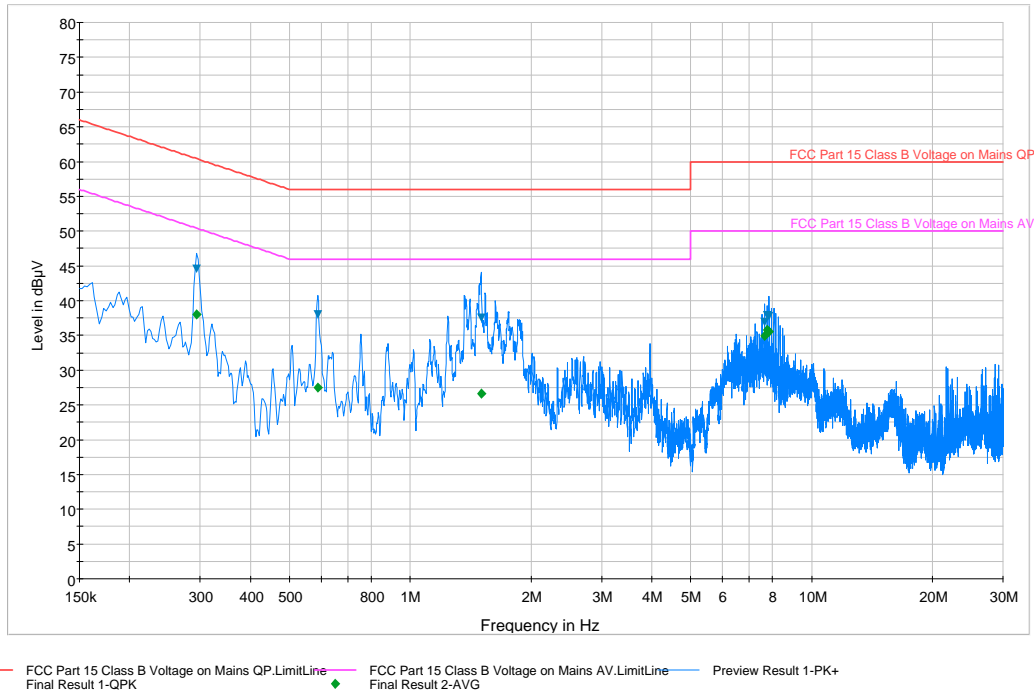
Plot 6-70. Line Conducted Plot with 802.11a UNII Band 1 (L1)
