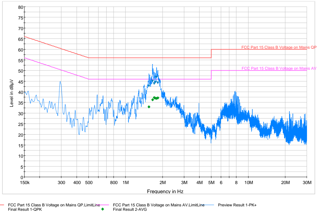
Plot 6-75. Line Conducted Plot with 802.11a UNII Band 2C (N)
