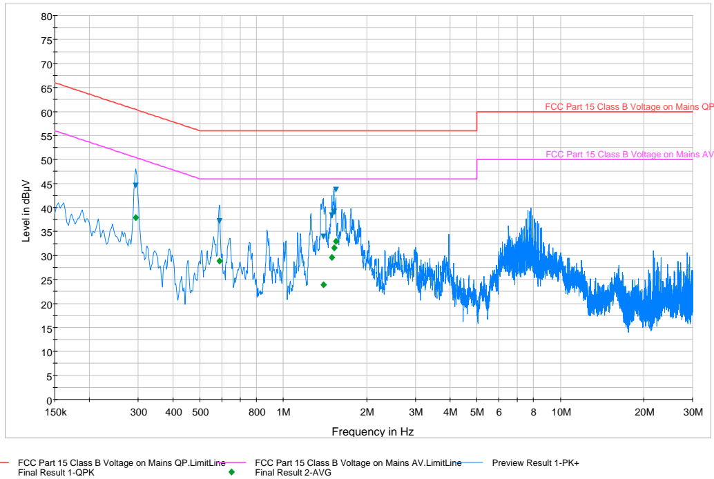
Plot 6-73. Line Conducted Plot with 802.11a UNII Band 2A (N)
