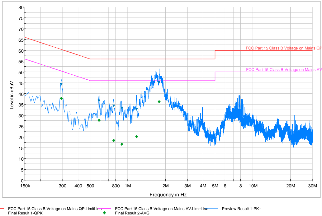
Plot 6-74. Line Conducted Plot with 802.11a UNII Band 2C (L1)
