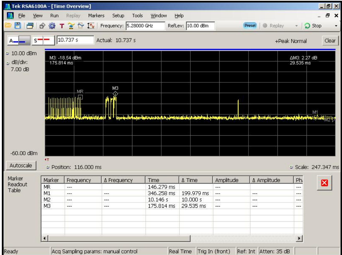
Figure 5-6. Last traffic burst from Client
