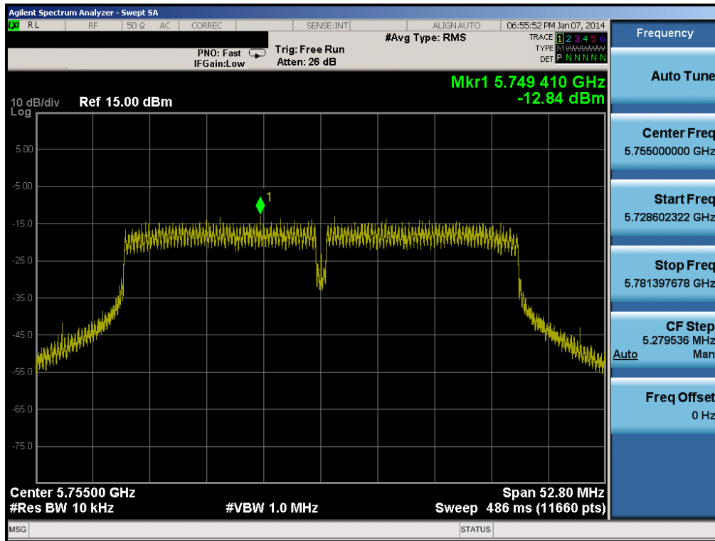
Plot 6-33. 6dB Bandwidth Plot (40MHz BW 802.11n (5.8GHz) – Ch. 151)
