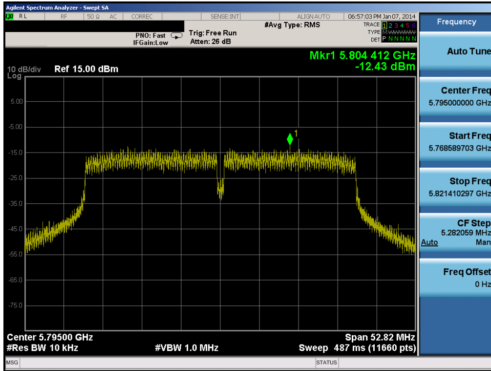
Plot 6-34. 6dB Bandwidth Plot (40MHz BW 802.11n (5.8GHz) – Ch. 159)
