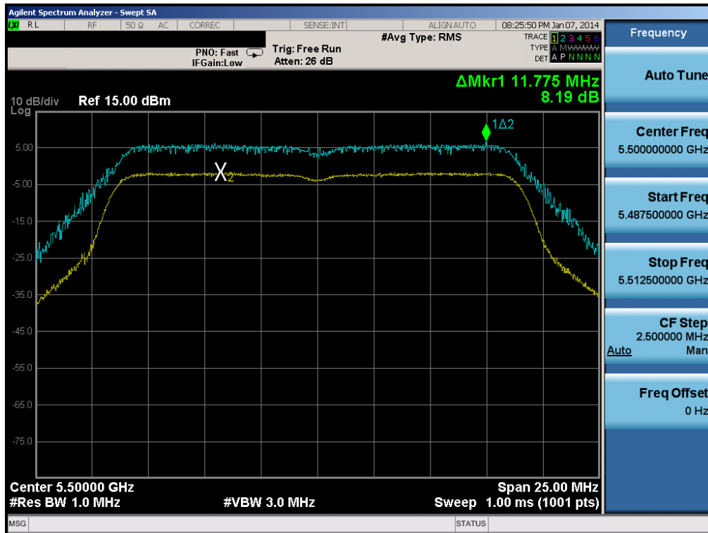
Plot 6-74. Peak Excursion Ratio Plot (20MHz BW 802.11n (UNII Band 2C) – Ch. 100)
