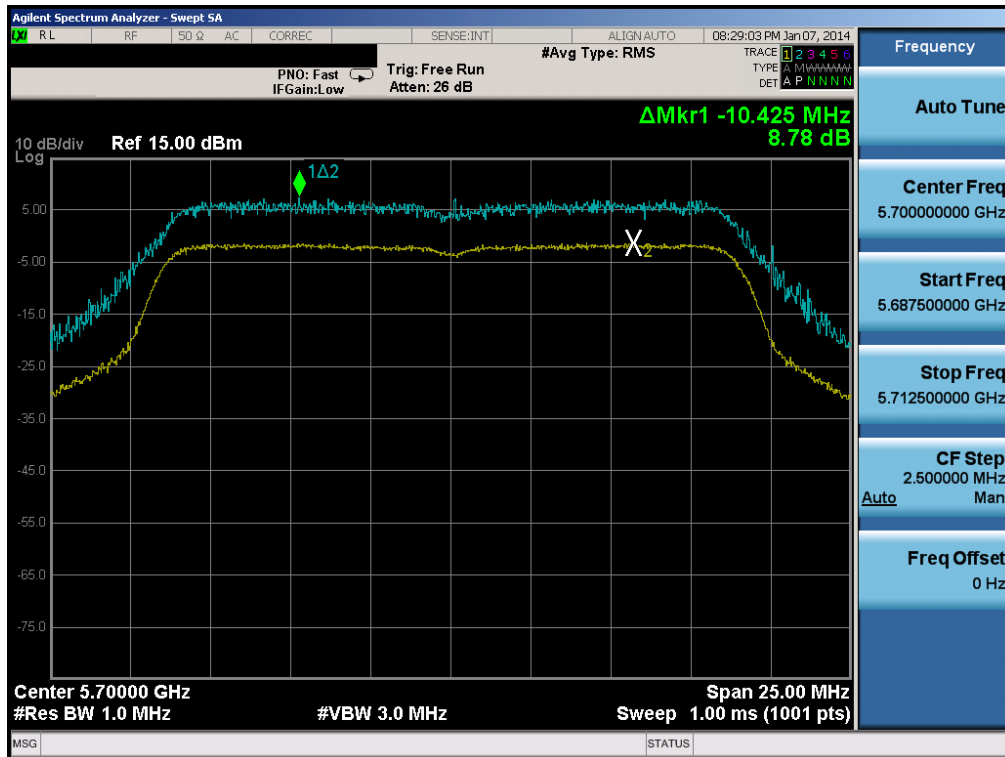
Plot 6-76. Peak Excursion Ratio Plot (20MHz BW 802.11n (UNII Band 2C) – Ch. 140)
