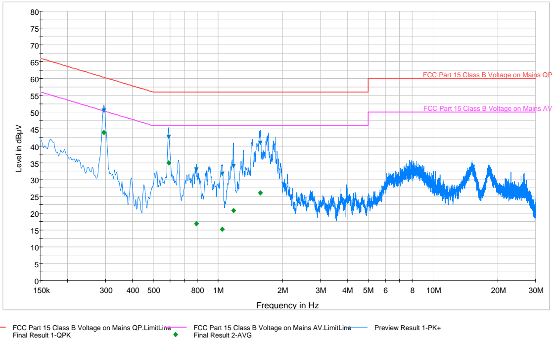
Plot 6-96. Line Conducted Plot with 802.11a UNII Band 2A (L1)
