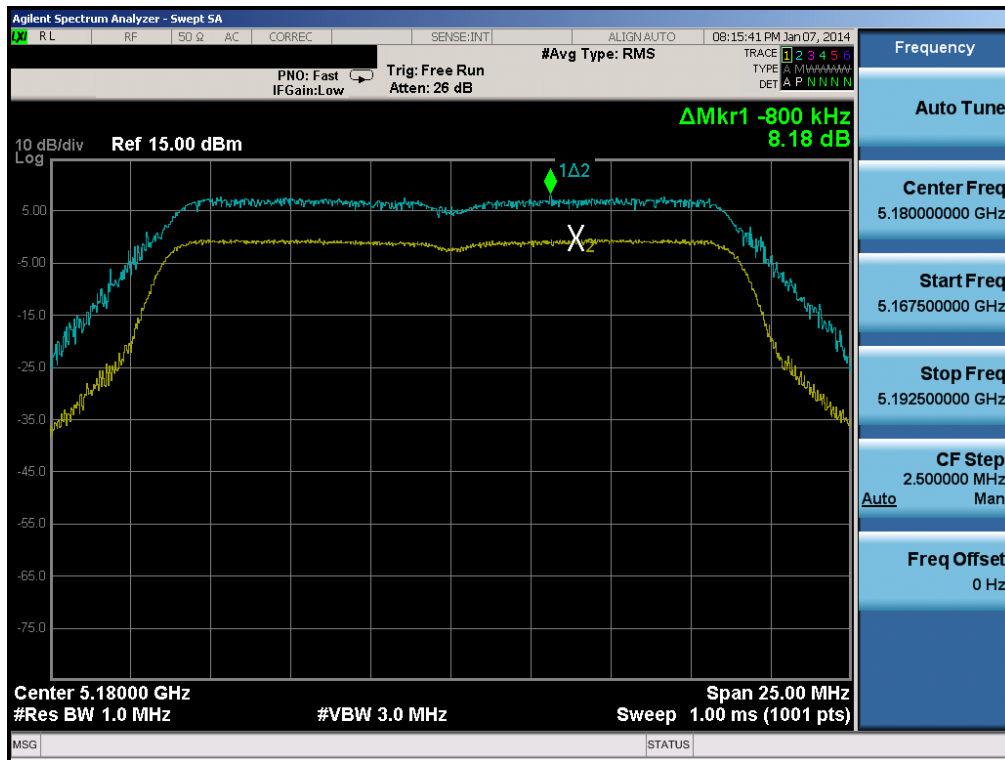
Plot 6-58. Peak Excursion Ratio Plot (20MHz BW 802.11n (UNII Band 1) – Ch. 36)
