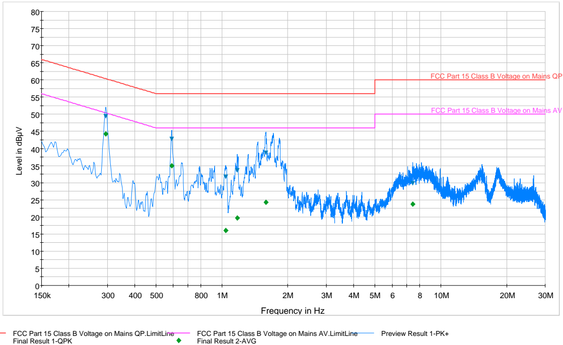
Plot 6-98. Line Conducted Plot with 802.11a UNII Band 2C (L1)
