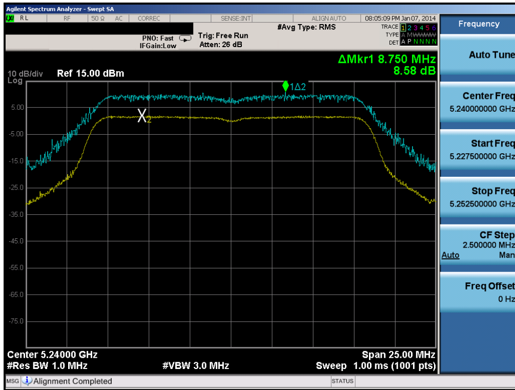
Plot 6-57. Peak Excursion Ratio Plot (802.11a (UNII Band 1) – Ch. 48)
