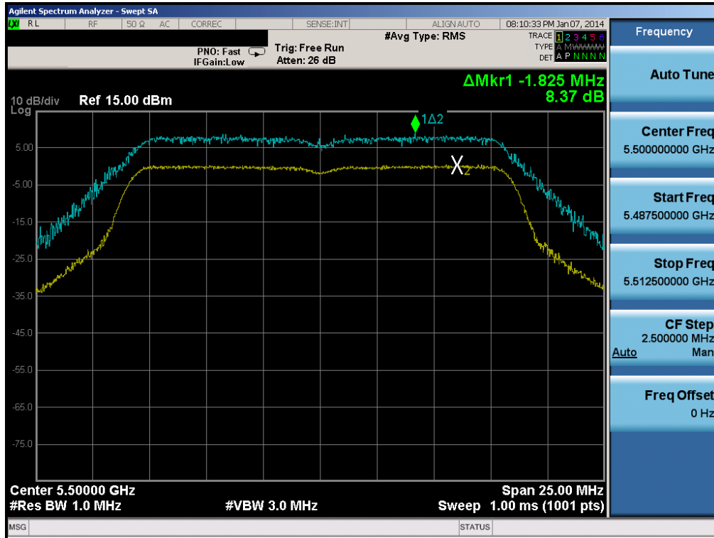
Plot 6-71. Peak Excursion Ratio Plot (802.11a (UNII Band 2C) – Ch. 100)
