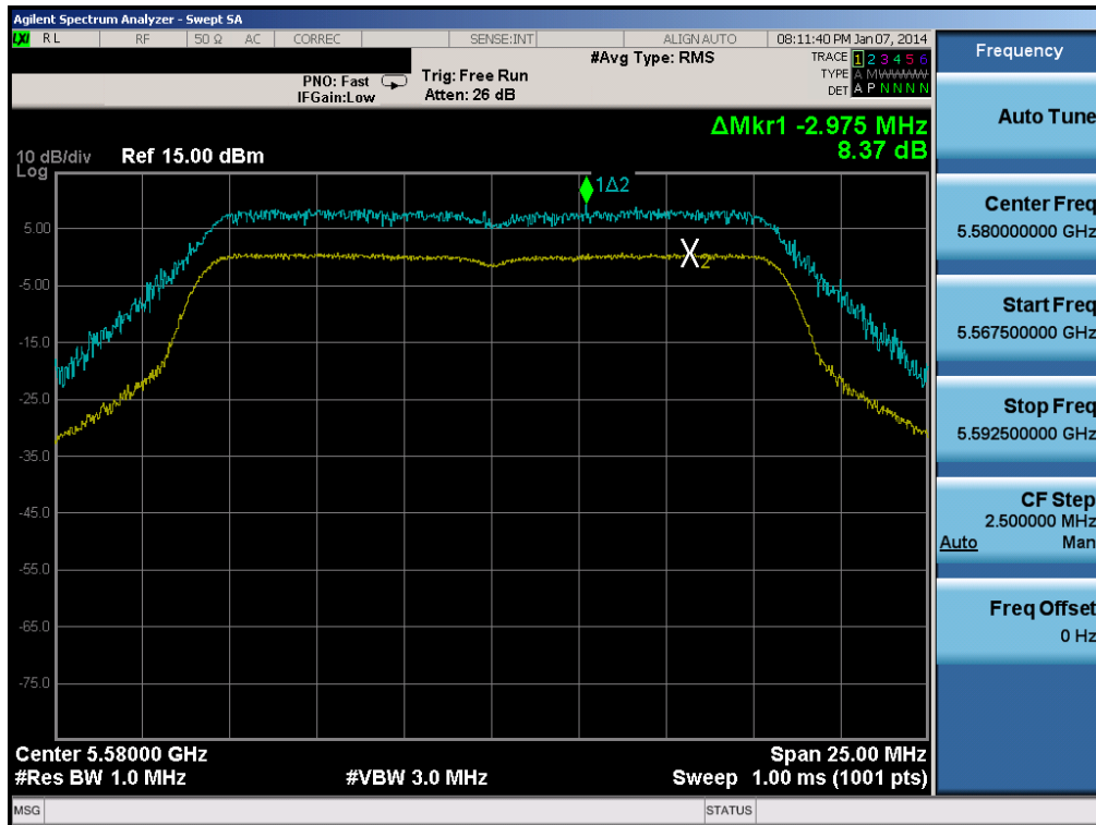
Plot 6-72. Peak Excursion Ratio Plot (802.11a (UNII Band 2C) – Ch. 116)
