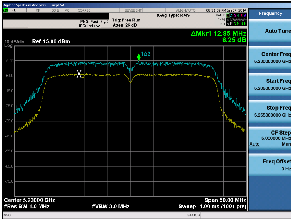
Plot 6-62. Peak Excursion Ratio Plot (40MHz BW 802.11n (UNII Band 1) – Ch. 46)
