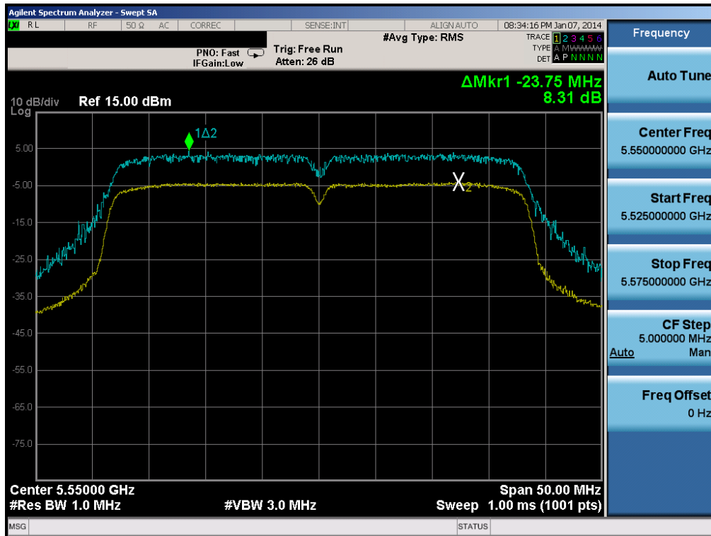
Plot 6-78. Peak Excursion Ratio Plot (40MHz BW 802.11n (UNII Band 2C) – Ch. 110)
