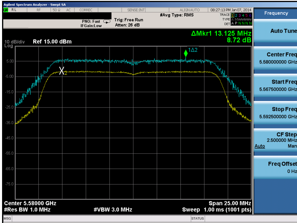
Plot 6-75. Peak Excursion Ratio Plot (20MHz BW 802.11n (UNII Band 2C) – Ch. 116)
