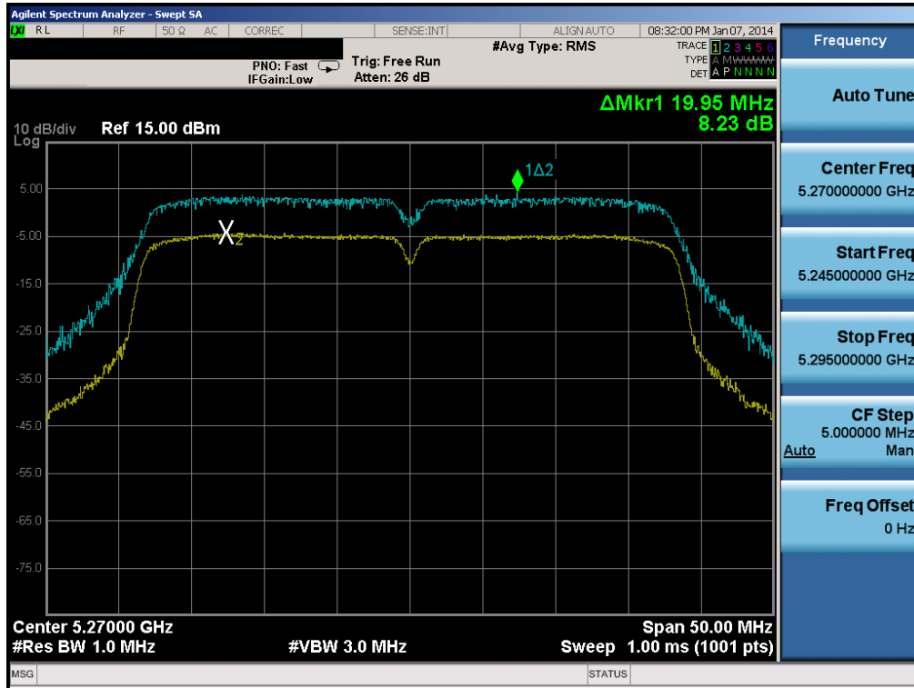
Plot 6-69. Peak Excursion Ratio Plot (40MHz BW 802.11n (UNII Band 2A) – Ch. 54)
