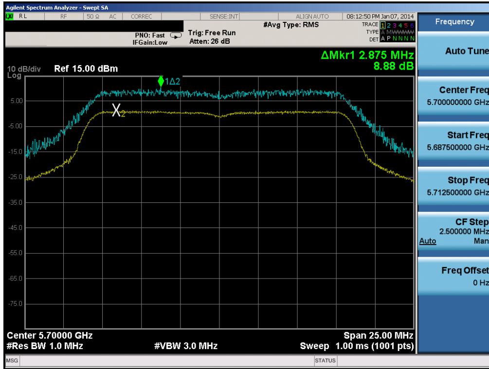
Plot 6-73. Peak Excursion Ratio Plot (802.11a (UNII Band 2C) – Ch. 140)
