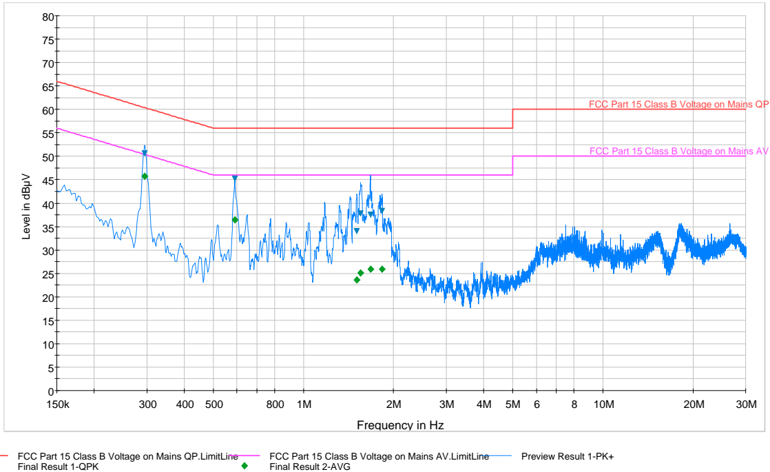
Plot 6-95. Line Conducted Plot with 802.11a UNII Band 1 (N)
