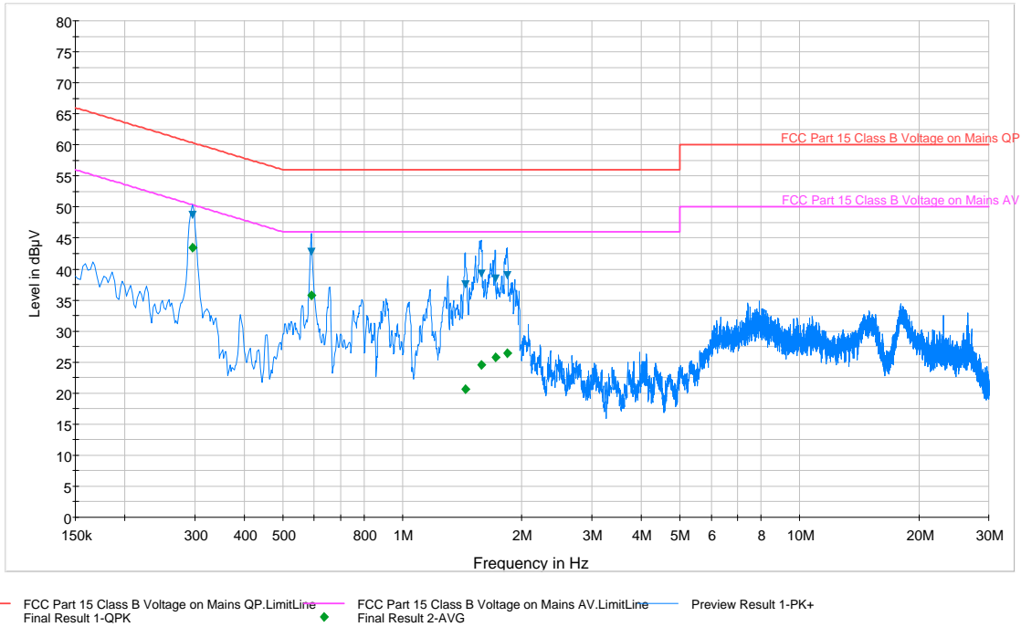
Plot 6-99. Line Conducted Plot with 802.11a UNII Band 2C (N)
