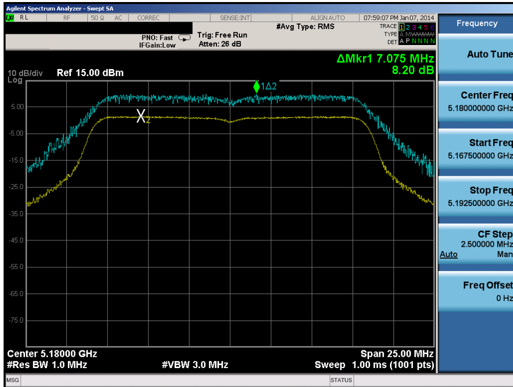
Plot 6-55. Peak Excursion Ratio Plot (802.11a (UNII Band 1) – Ch. 36)
