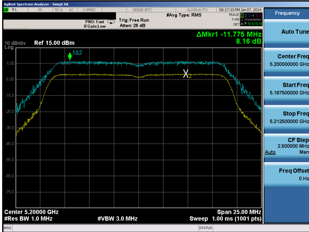
Plot 6-59. Peak Excursion Ratio Plot (20MHz BW 802.11n (UNII Band 1) – Ch. 40)
