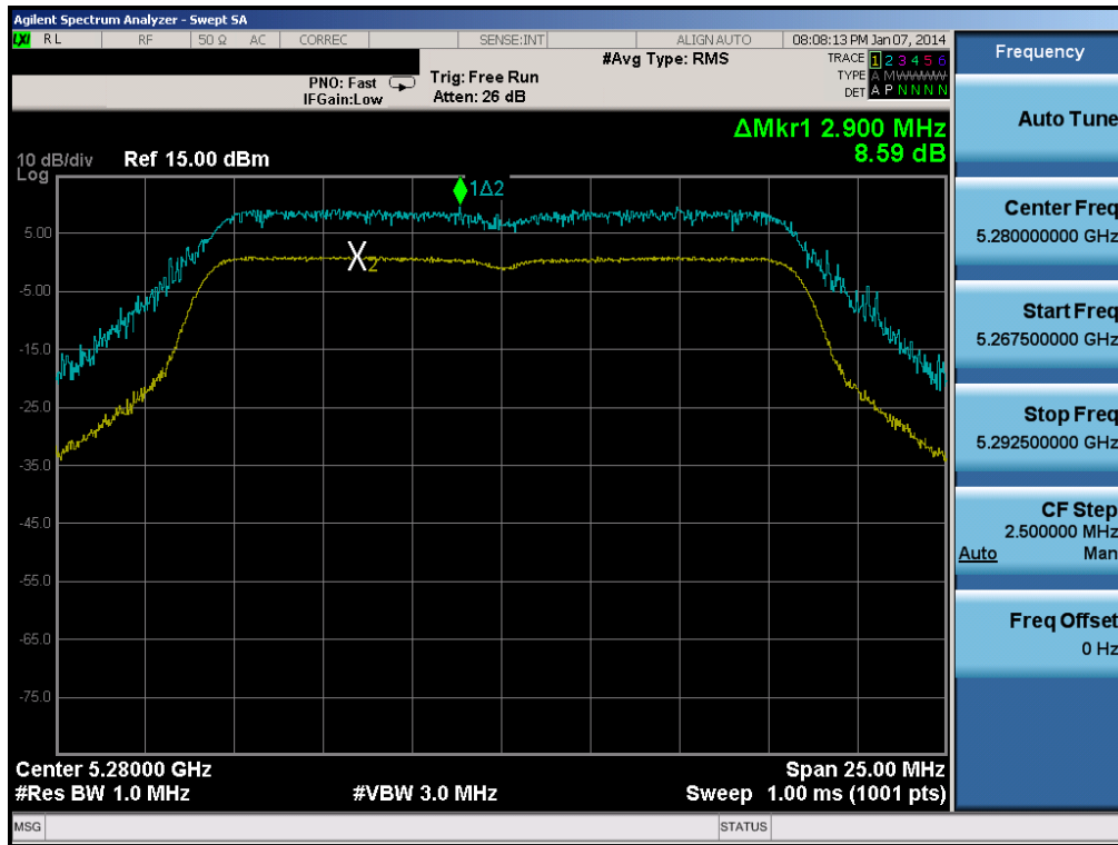
Plot 6-64. Peak Excursion Ratio Plot (802.11a (UNII Band 2A) – Ch. 56)
