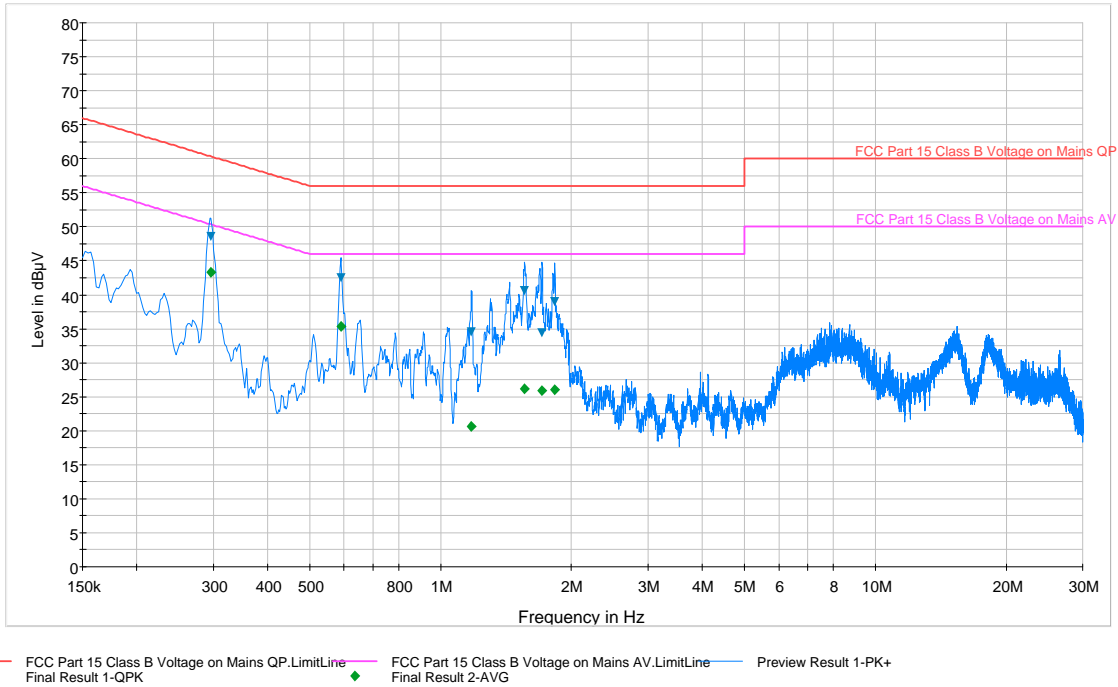
Plot 6-94. Line Conducted Plot with 802.11a UNII Band 1 (L1)
