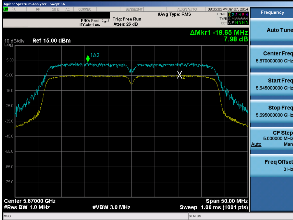
Plot 6-79. Peak Excursion Ratio Plot (40MHz BW 802.11n (UNII Band 2C) – Ch. 134)
