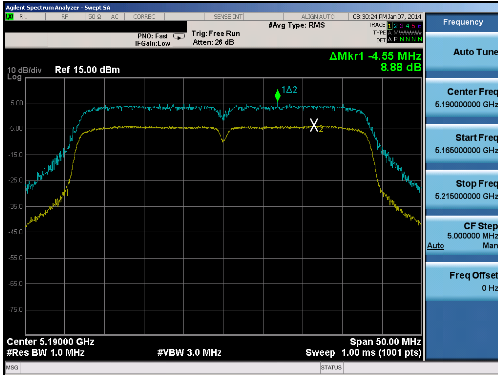
Plot 6-61. Peak Excursion Ratio Plot (40MHz BW 802.11n (UNII Band 1) – Ch. 38)
