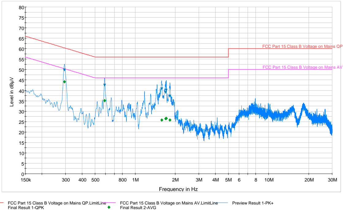
Plot 6-97. Line Conducted Plot with 802.11a UNII Band 2A (N)
