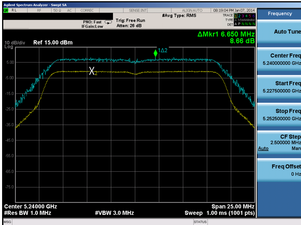
Plot 6-60. Peak Excursion Ratio Plot (20MHz BW 802.11n (UNII Band 1) – Ch. 48)
