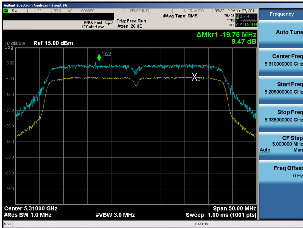
Plot 6-70. Peak Excursion Ratio Plot (40MHz BW 802.11n (UNII Band 2A) – Ch. 62)
