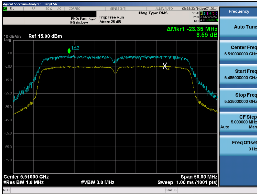
Plot 6-77. Peak Excursion Ratio Plot (40MHz BW 802.11n (UNII Band 2C) – Ch. 102)
