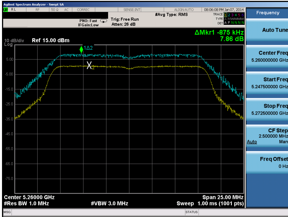
Plot 6-63. Peak Excursion Ratio Plot (802.11a (UNII Band 2A) – Ch. 52)
