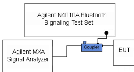
Figure 7-5. Test Instrument & Measurement Setup
