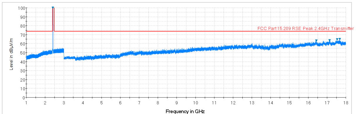
Plot 7-32. Radiated Spurious Plot above 1GHz (802.11b – Ch. 1, Ant. Pol. V)
