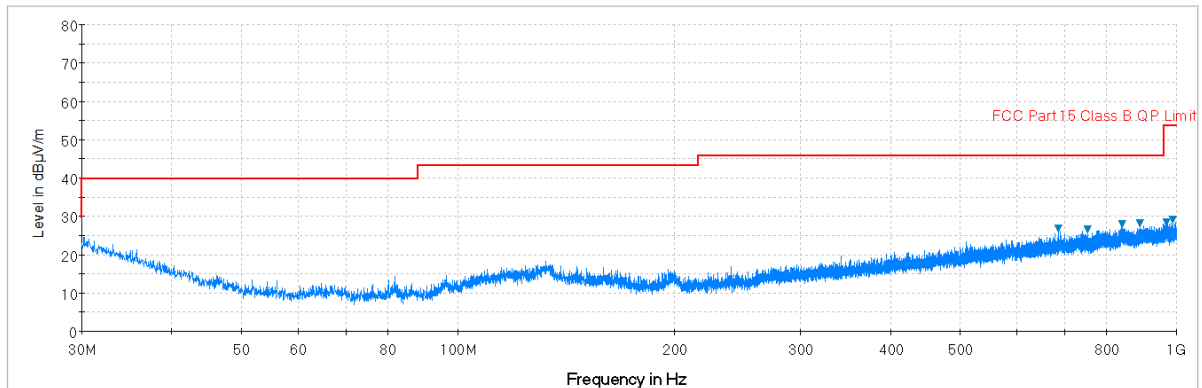
Plot 7-41. Radiated Spurious Plot below 1GHz (Pol. H)
