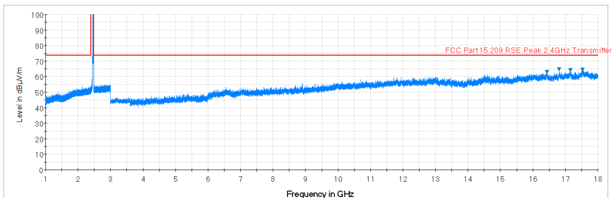
Plot 7-36. Radiated Spurious Plot above 1GHz (802.11b – Ch. 11, Ant. Pol. V)
