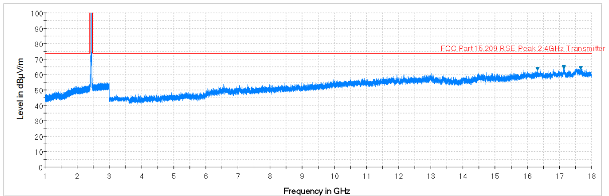
Plot 7-33. Radiated Spurious Plot above 1GHz (802.11b – Ch. 6, Ant. Pol. H)
