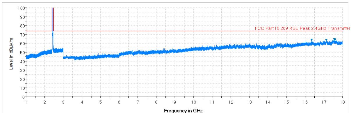
Plot 7-34. Radiated Spurious Plot above 1GHz (802.11b – Ch. 6, Ant. Pol. V)
