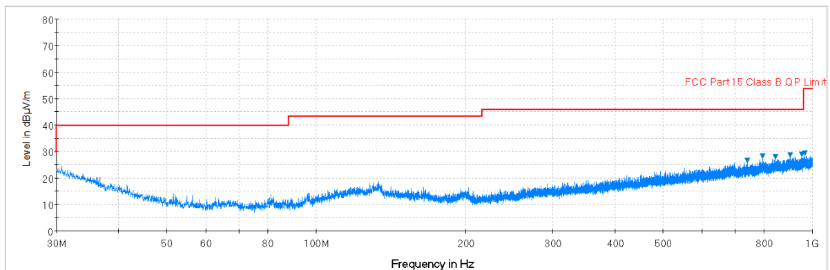
Plot 7-42. Radiated Spurious Plot below 1GHz (Pol. V)
