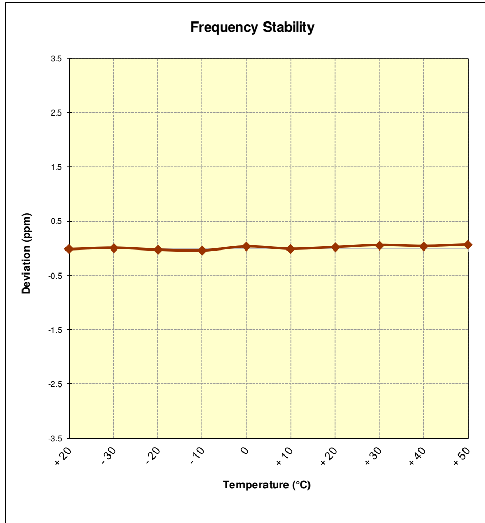
Figure 7-11. Frequency Stability Graph (PCS WCDMA Mode – Ch. 9400)
