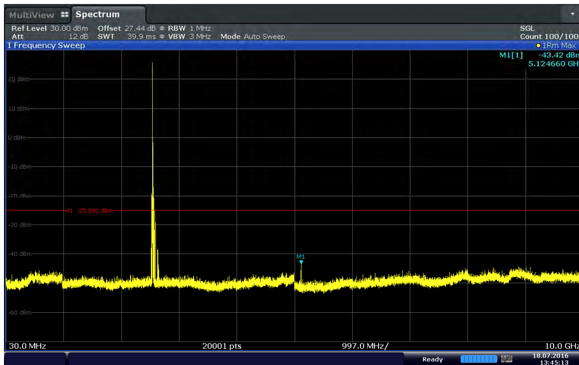
Plot 6-27. Conducted Spurious Plot (Band 41-15MHz-QPSK-RB Size 1-RB Offset 37-Ch.40315)
