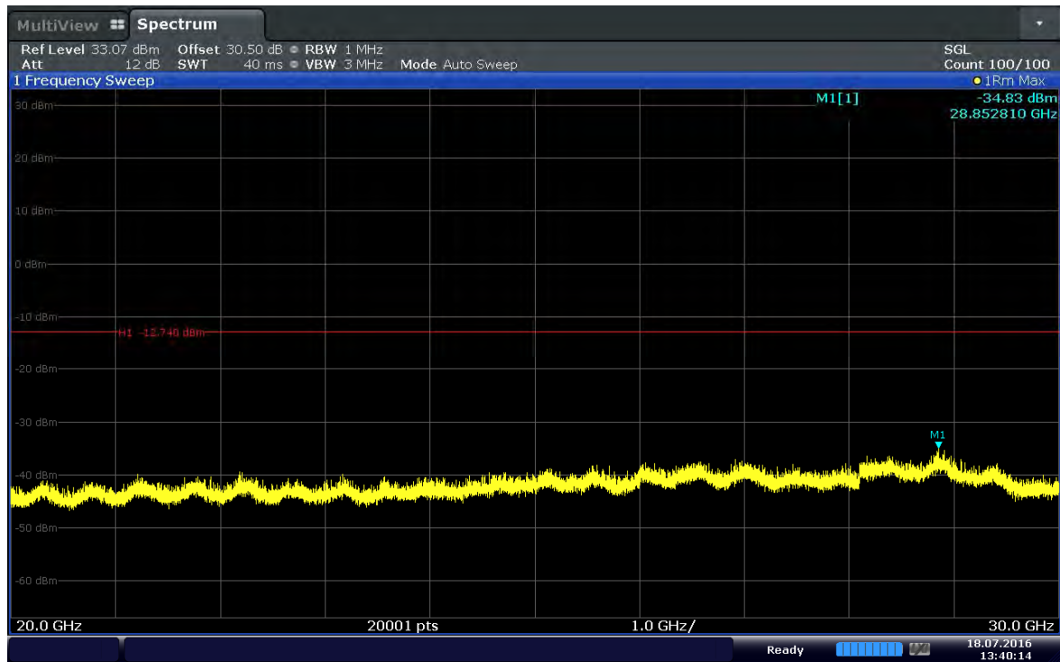
Plot 6-23. Conducted Spurious Plot (Band 41-10MHz-QPSK- RB Size 1-RB Offset 49-Ch.40740)
