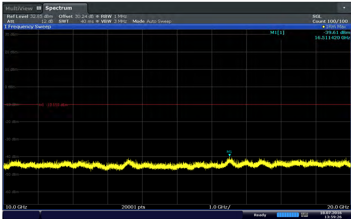
Plot 6-43. Conducted Spurious Plot (Band 41–20MHz–QPSK–RB Size 1–RB Offset 49–Ch.41140)
