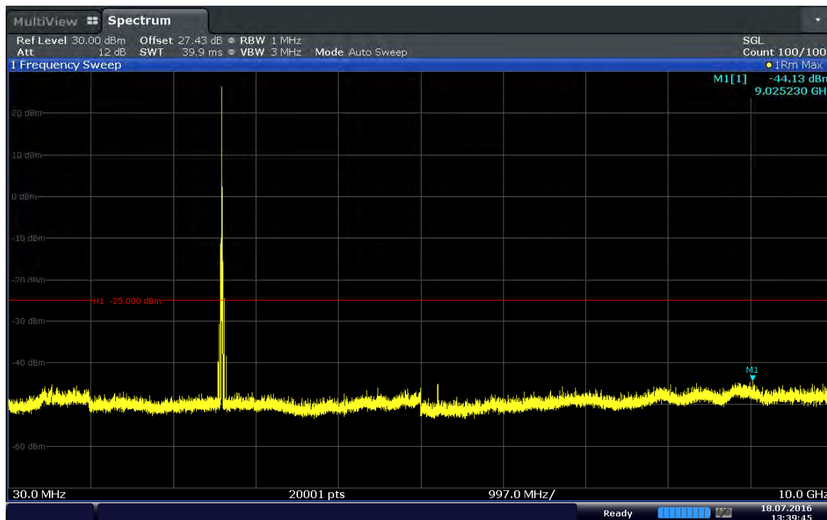
Plot 6-21. Conducted Spurious Plot (Band 41-10MHz-QPSK-RB Size 1-RB Offset 49-Ch.40740)
