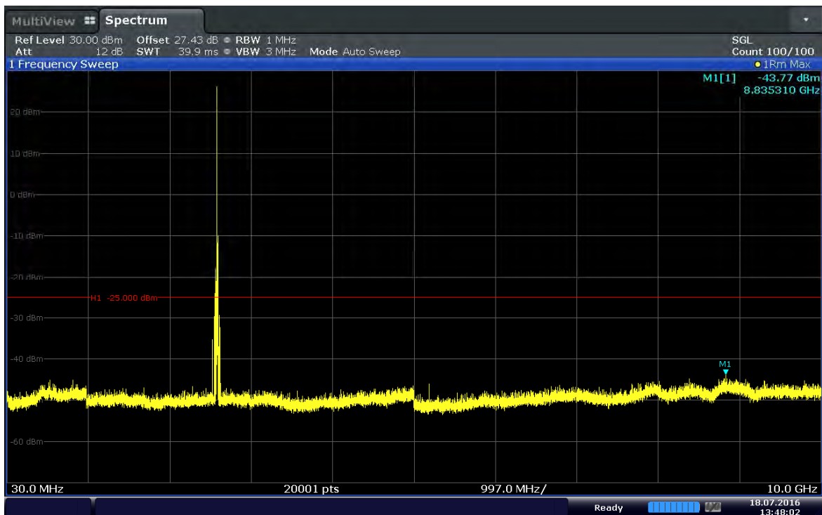
Plot 6-30. Conducted Spurious Plot (Band 41-15MHz-QPSK-RB Size 1-RB Offset 0-Ch.40740)
