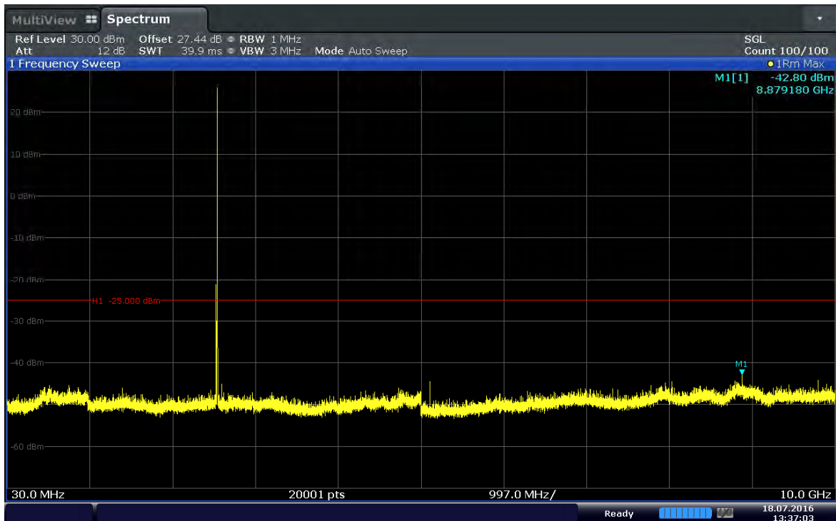
Plot 6-18. Conducted Spurious Plot (Band 41-10MHz-QPSK- RB Size 1-RB Offset 24-Ch.40290)
