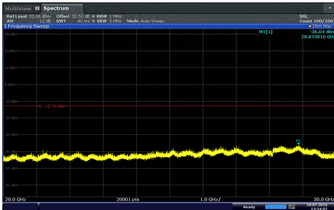
Plot 6-38. Conducted Spurious Plot (Band 41–20MHz–QPSK–RB Size 1–RB Offset 49–Ch.40340)
