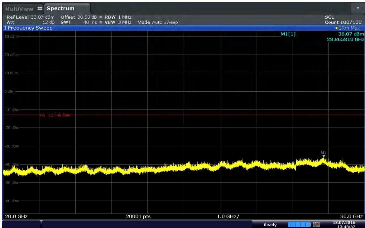
Plot 6-32. Conducted Spurious Plot (Band 41–15MHz–QPSK–RB Size 1–RB Offset 0–Ch.40740)
