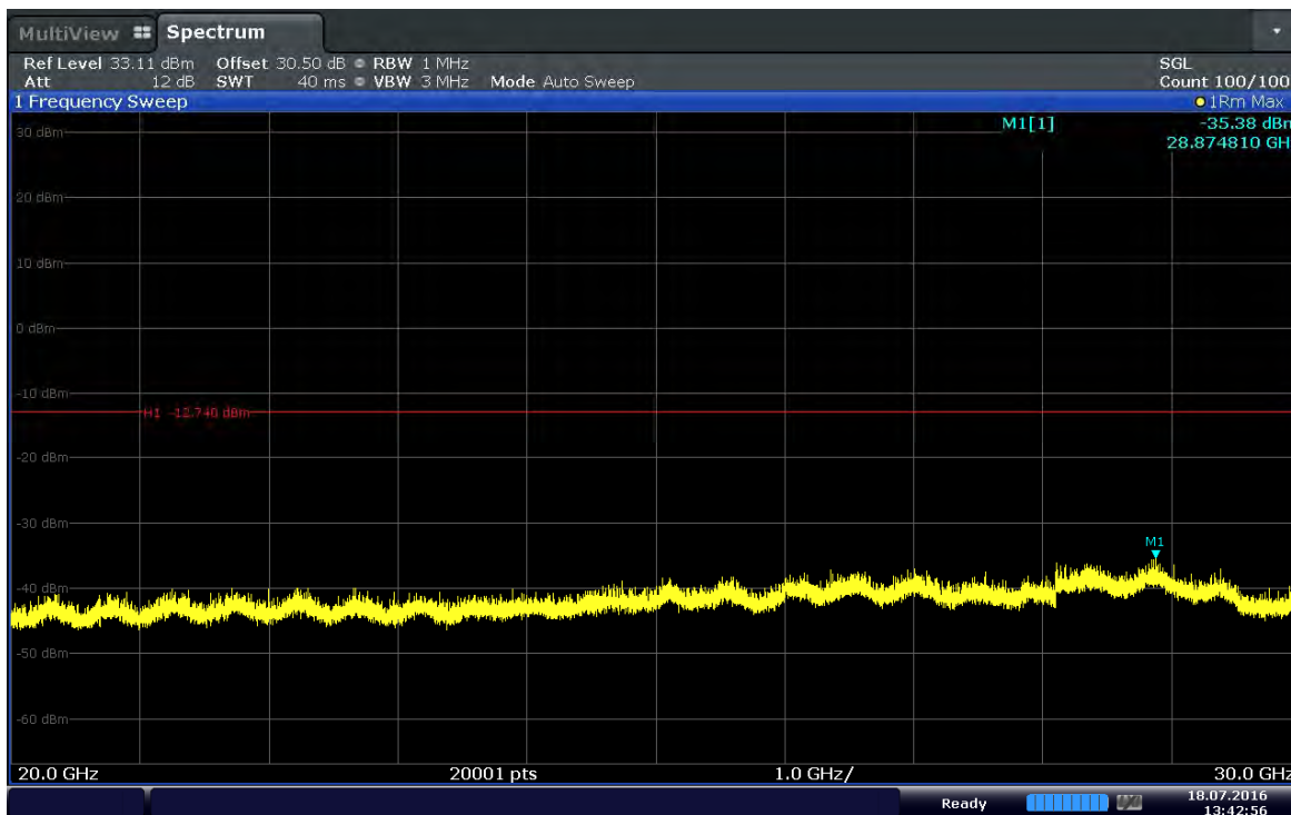
Plot 6-26. Conducted Spurious Plot (Band 41–10MHz–QPSK– RB Size 1–RB Offset 24–Ch.41190)
