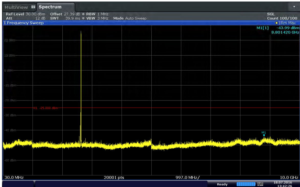
Plot 6-24. Conducted Spurious Plot (Band 41-10MHz-QPSK-RB Size 1-RB Offset 24-Ch.41190)
