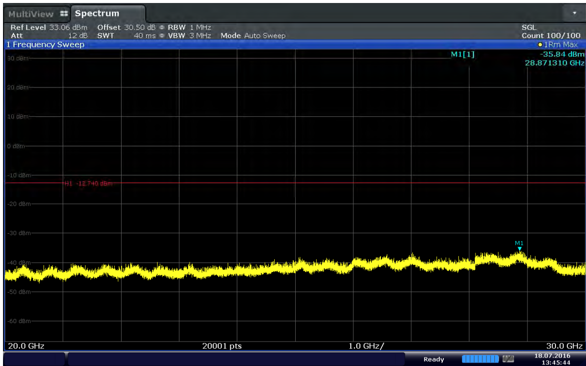
Plot 6-29. Conducted Spurious Plot (Band 41-15MHz-QPSK-RB Size 1-RB Offset 37-Ch.40315)
