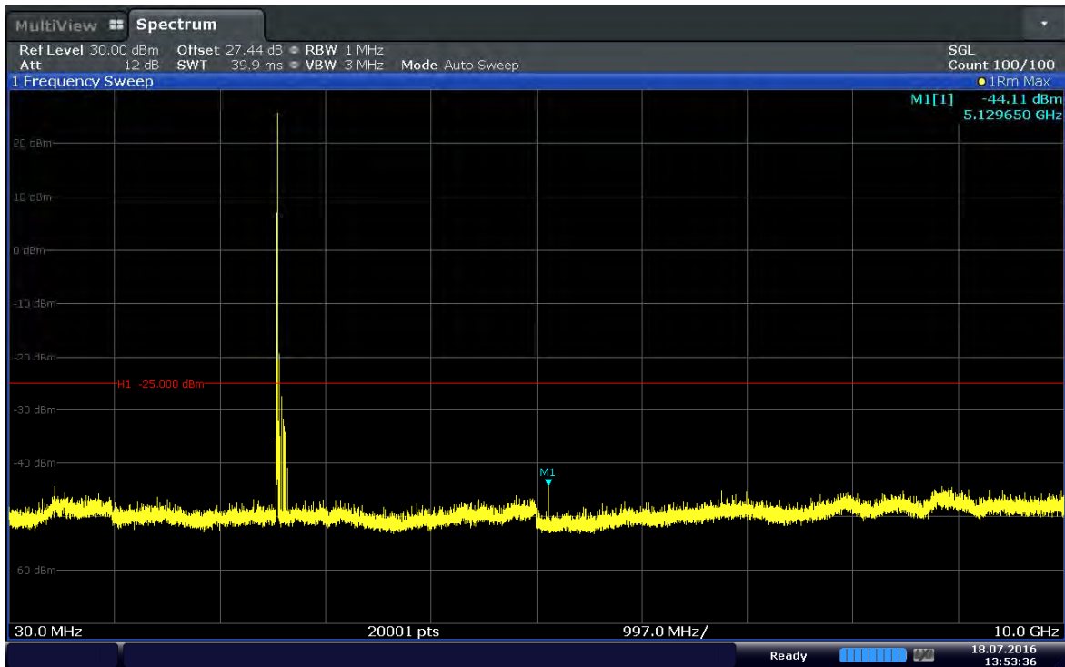
Plot 6-36. Conducted Spurious Plot (Band 41-20MHz-QPSK-RB Size 1-RB Offset 49-Ch.40340)
