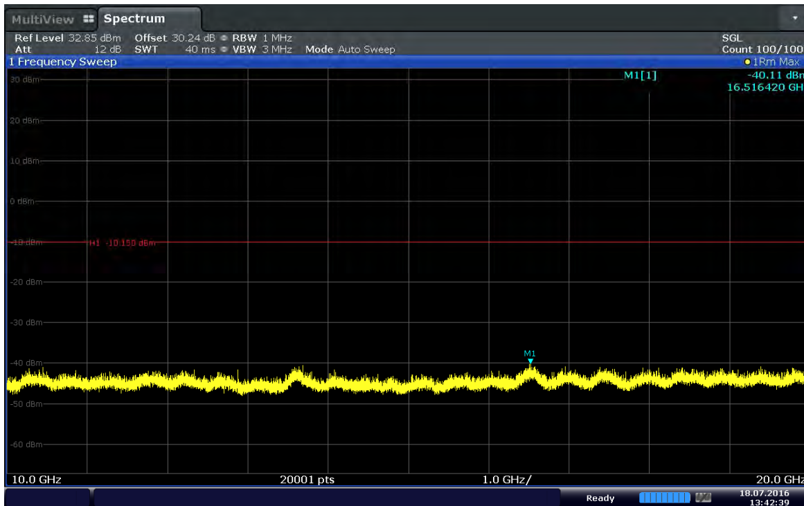
Plot 6-25. Conducted Spurious Plot (Band 41–10MHz–QPSK– RB Size 1–RB Offset 24–Ch.41190)
