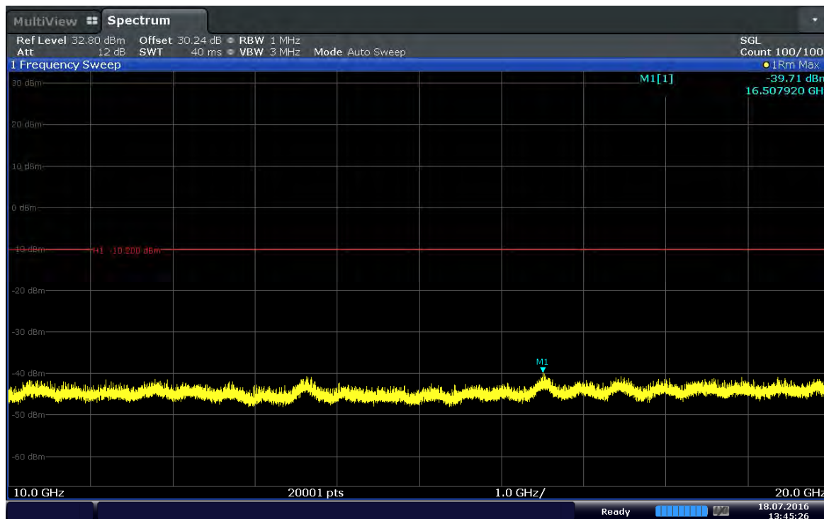
Plot 6-28. Conducted Spurious Plot (Band 41-15MHz-QPSK-RB Size 1-RB Offset 37-Ch.40315)
