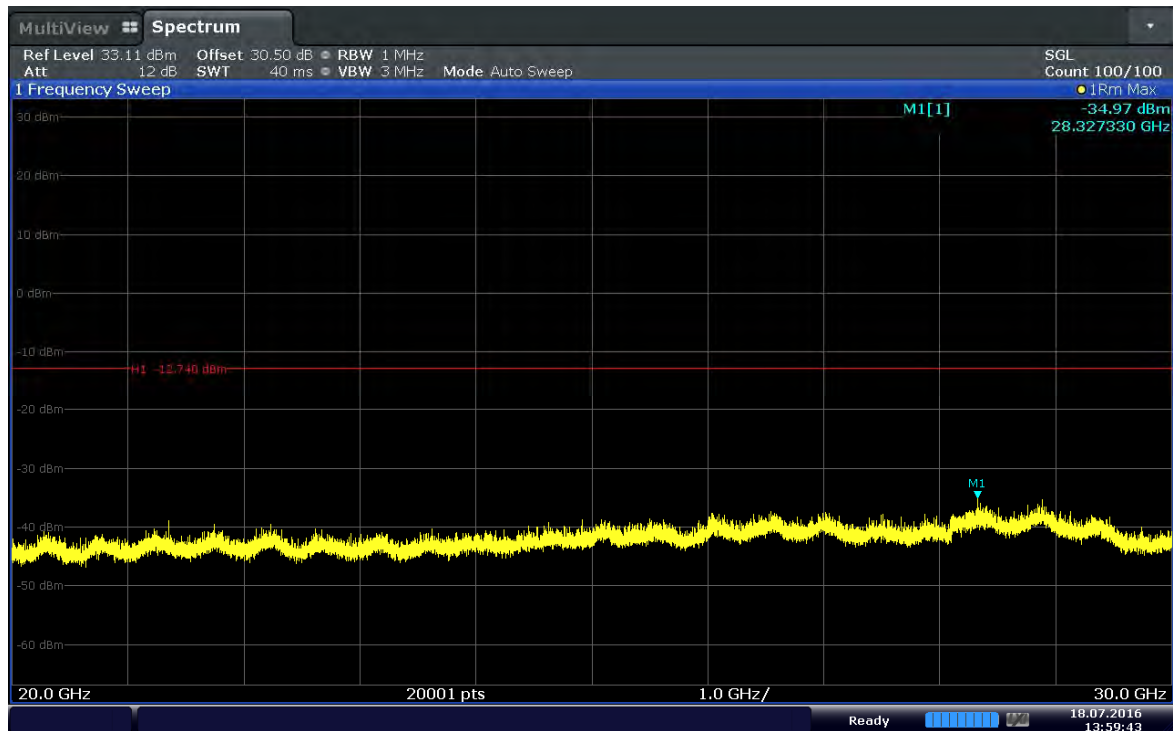
Plot 6-44. Conducted Spurious Plot (Band 41–20MHz–QPSK–RB Size 1–RB Offset 49–Ch.41140)
