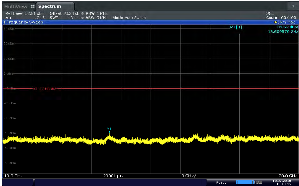
Plot 6-31. Conducted Spurious Plot (Band 41–15MHz–QPSK–RB Size 1–RB Offset 0–Ch.40740)
