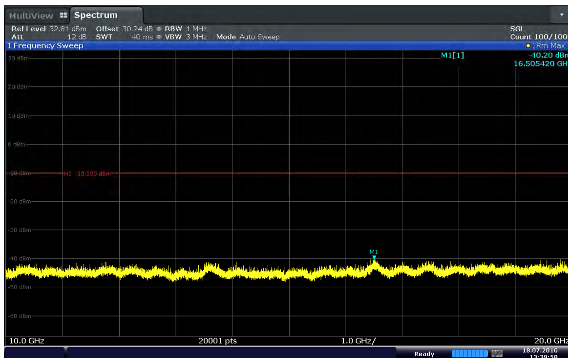
Plot 6-22. Conducted Spurious Plot (Band 41-10MHz-QPSK- RB Size 1-RB Offset 49-Ch.40740)
