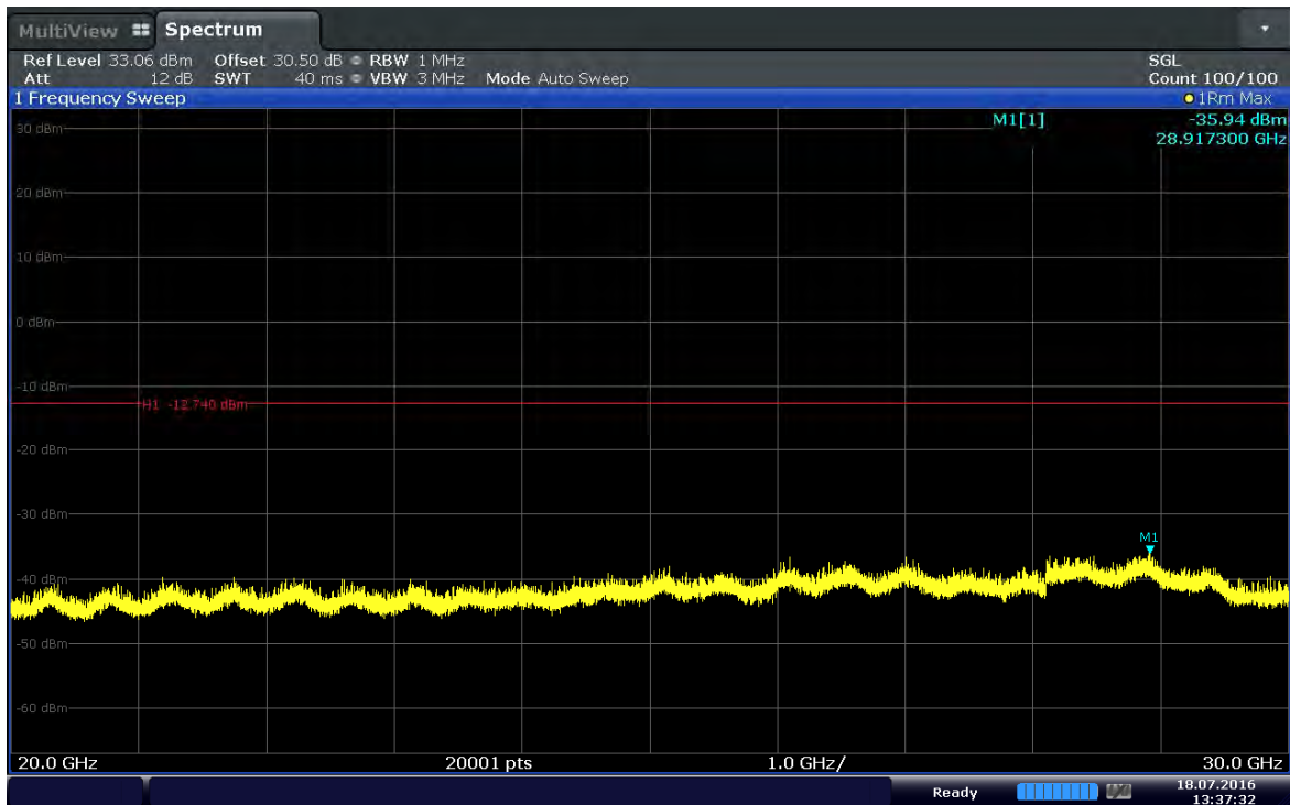
Plot 6-20. Conducted Spurious Plot (Band 41–10MHz–QPSK– RB Size 1–RB Offset 24–Ch.40290)
