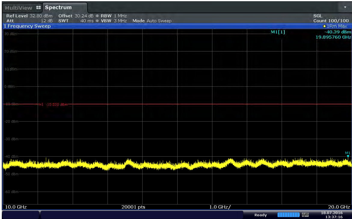
Plot 6-19. Conducted Spurious Plot (Band 41–10MHz–QPSK– RB Size 1–RB Offset 24–Ch.40290)
