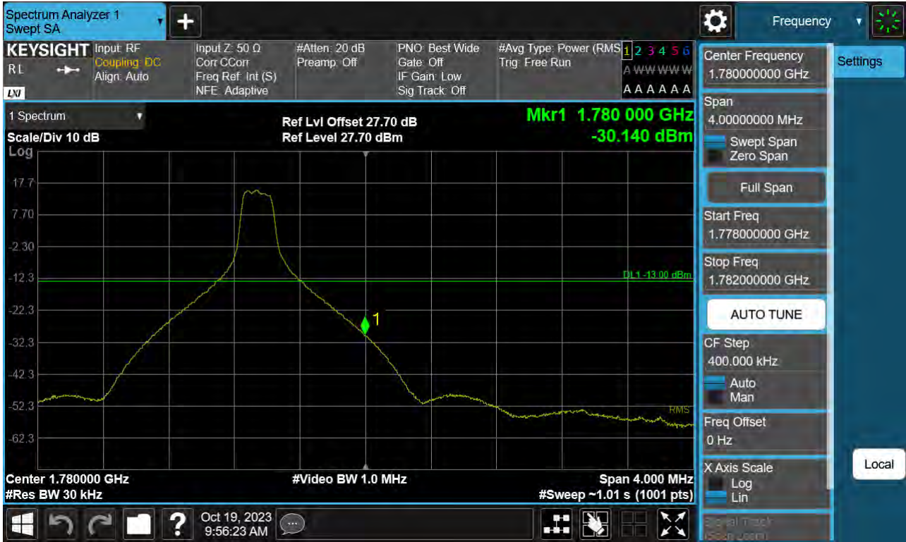
Sub6 n66. Upper Band Edge Plot (40 M BW Ch.342000 BPSK_RB1_Offset 105) -1
