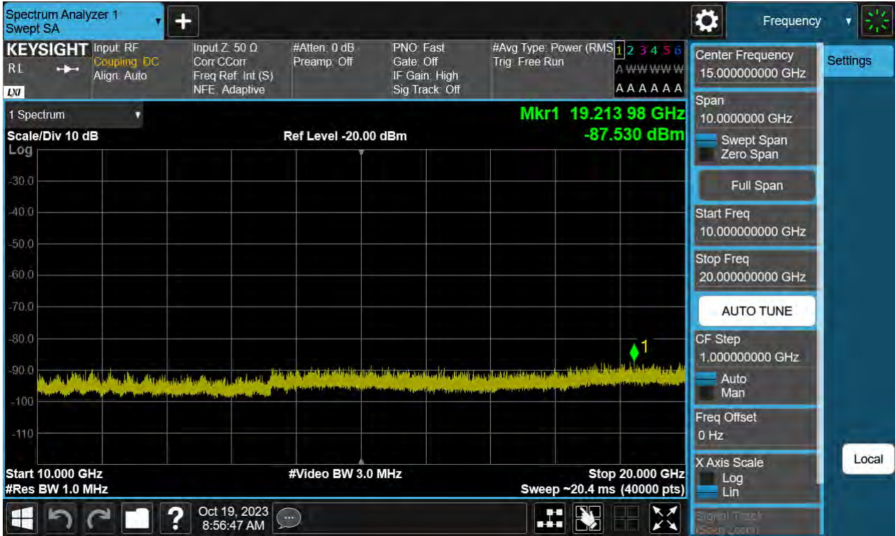
Sub6 n66. Conducted Spurious Plot_2 (344500ch_25 MHz_BPSK_RB 1_1)
