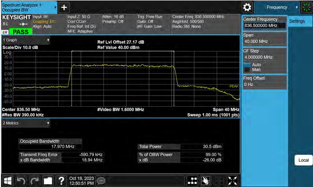
Sub6 n26. Occupied Bandwidth Plot (20 M BW Ch.167300 QPSK RB 100_0)
