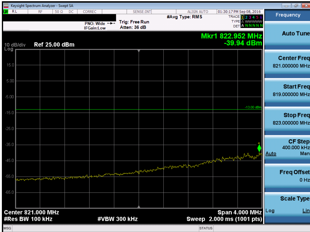
Plot 7-19. Lower Extended Band Edge Plot (Band 5 – 1.4MHz QPSK – RB Size 6)
