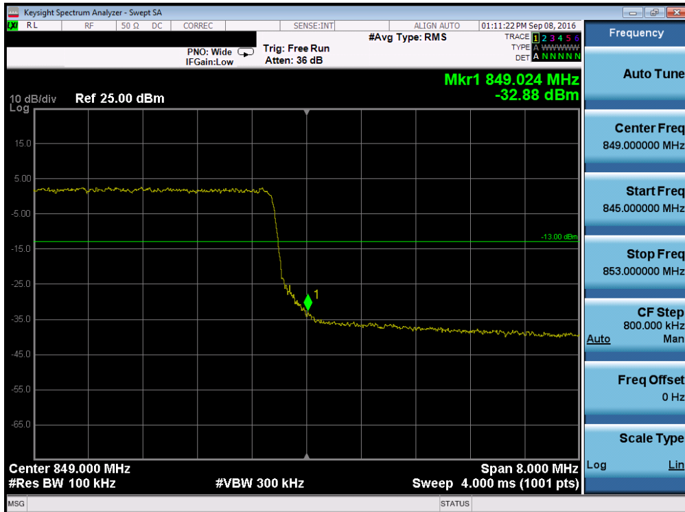
Plot 7-31. Upper Band Edge Plot (Band 5 – 10.0MHz QPSK – RB Size 50)
