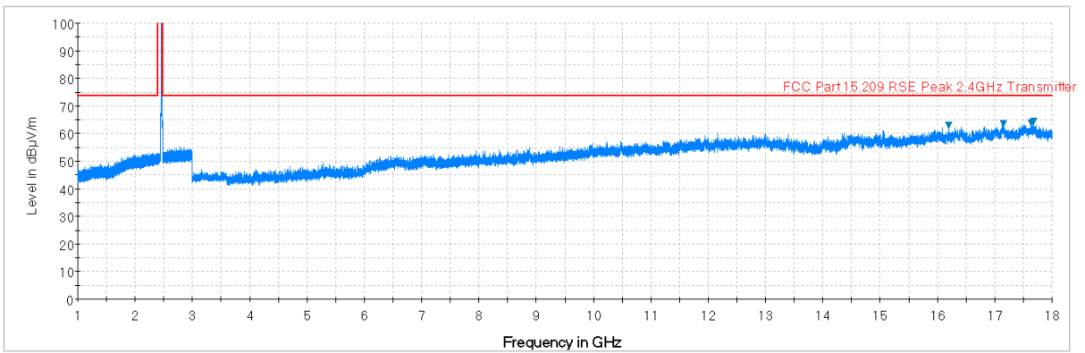
Plot 7-44. Radiated Spurious Plot above 1GHz (802.11b – Ch. 11, Ant. Pol. H)
