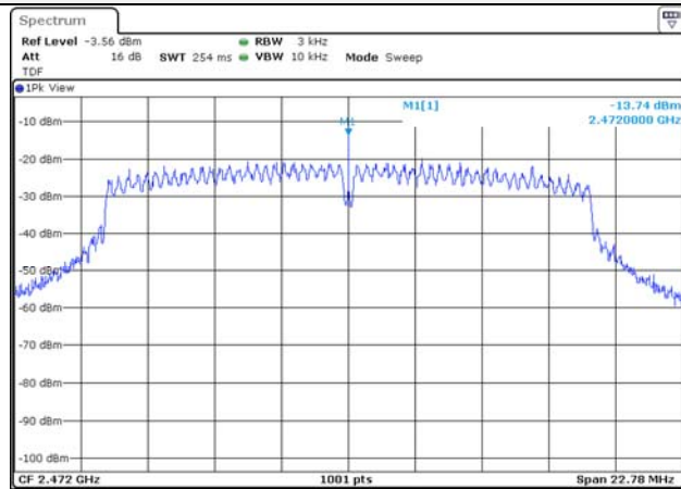
802.11g / 2 472 MHz
