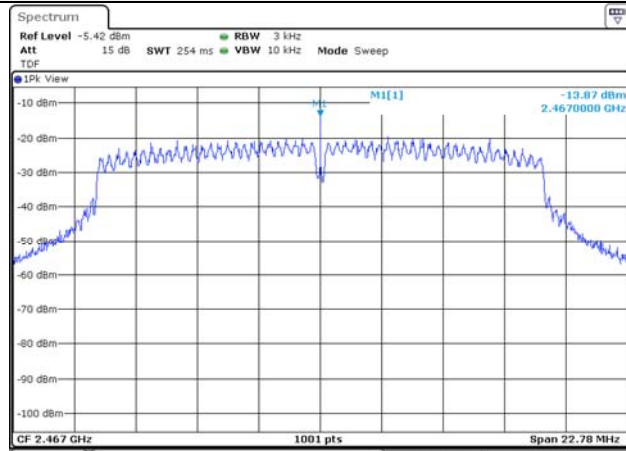
802.11g / 2 467 MHz
