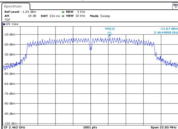
802.11g / 2 462 MHz
