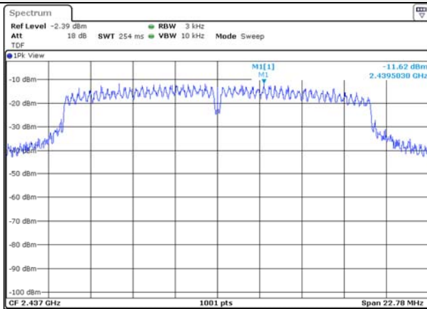
802.11g / 2 437 MHz
