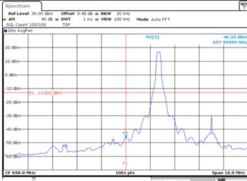
5M BW QPSK Low ch. FRB
