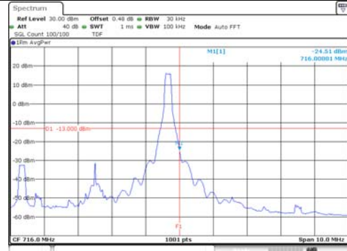
5M BW QPSK High ch. FRB
