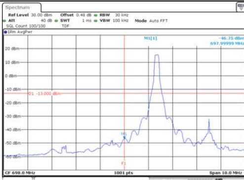
5M BW 16QAM Low ch. FRB
