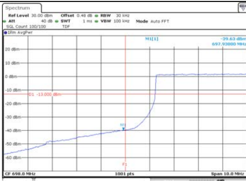
5M BW 16QAM Low ch. 1RB
