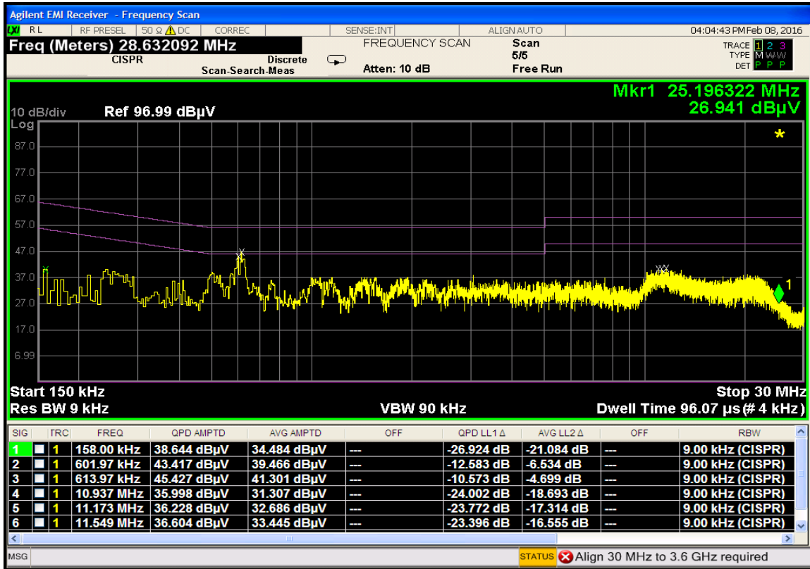
Plot 7-52. Line Conducted Plot with 802.11b (N)
