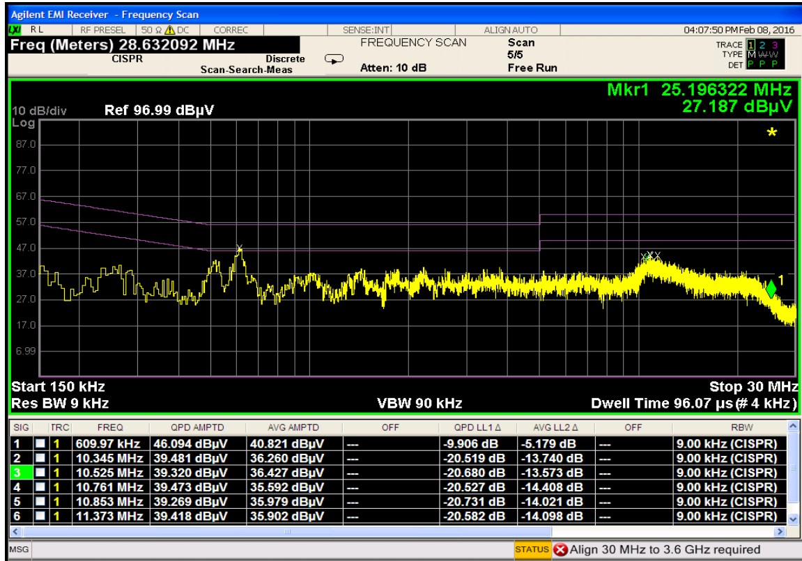
Plot 7-51. Line Conducted Plot with 802.11b (L1)
