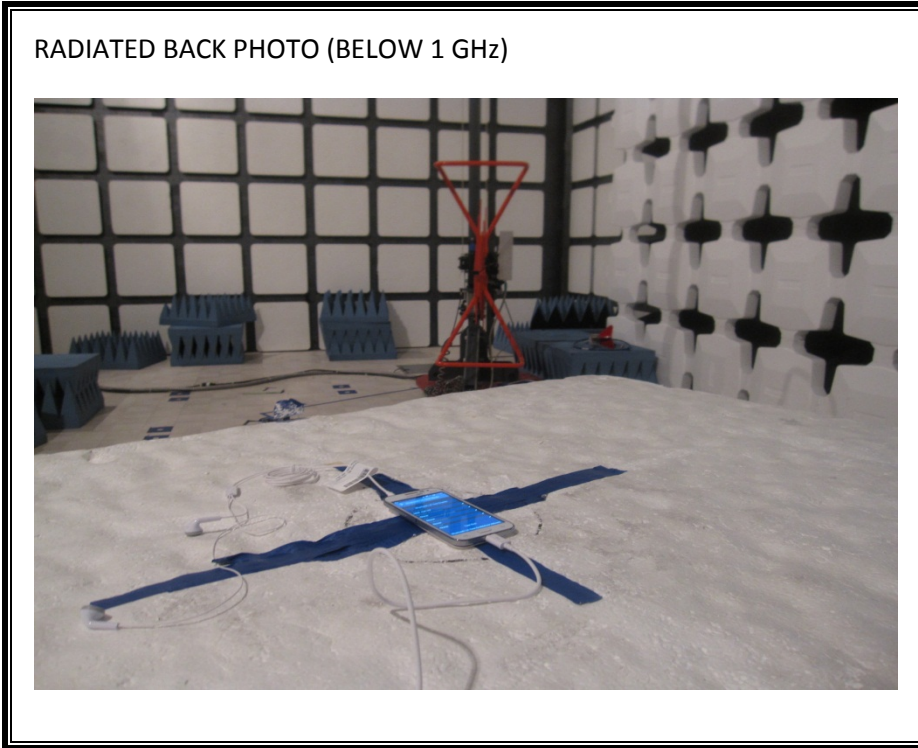
RADIATED RF MEASUREMENT SETUP (ABOVE 1 GHz)
