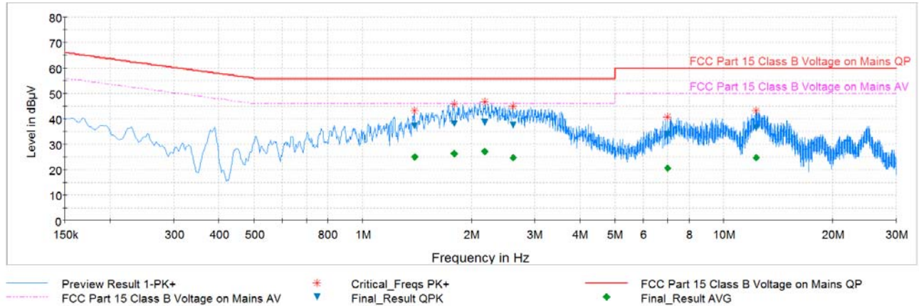
Plot 6-36. Line Conducted Plot with 802.11b (N)
