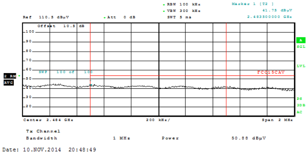
Plot 6-33. Radiated Restricted Upper Band Edge Measurement (Average)
