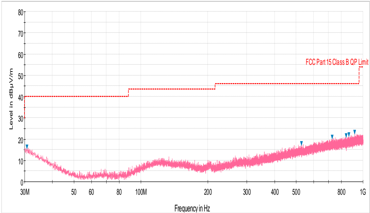
Plot 6-42. Radiated Spurious Plot below 1GHz (Pol. V)
