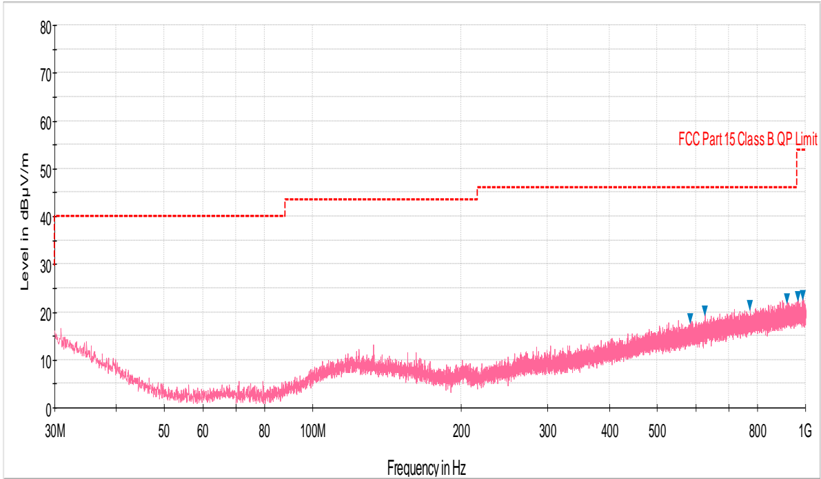
Plot 6-41. Radiated Spurious Plot below 1GHz (Pol. H)
