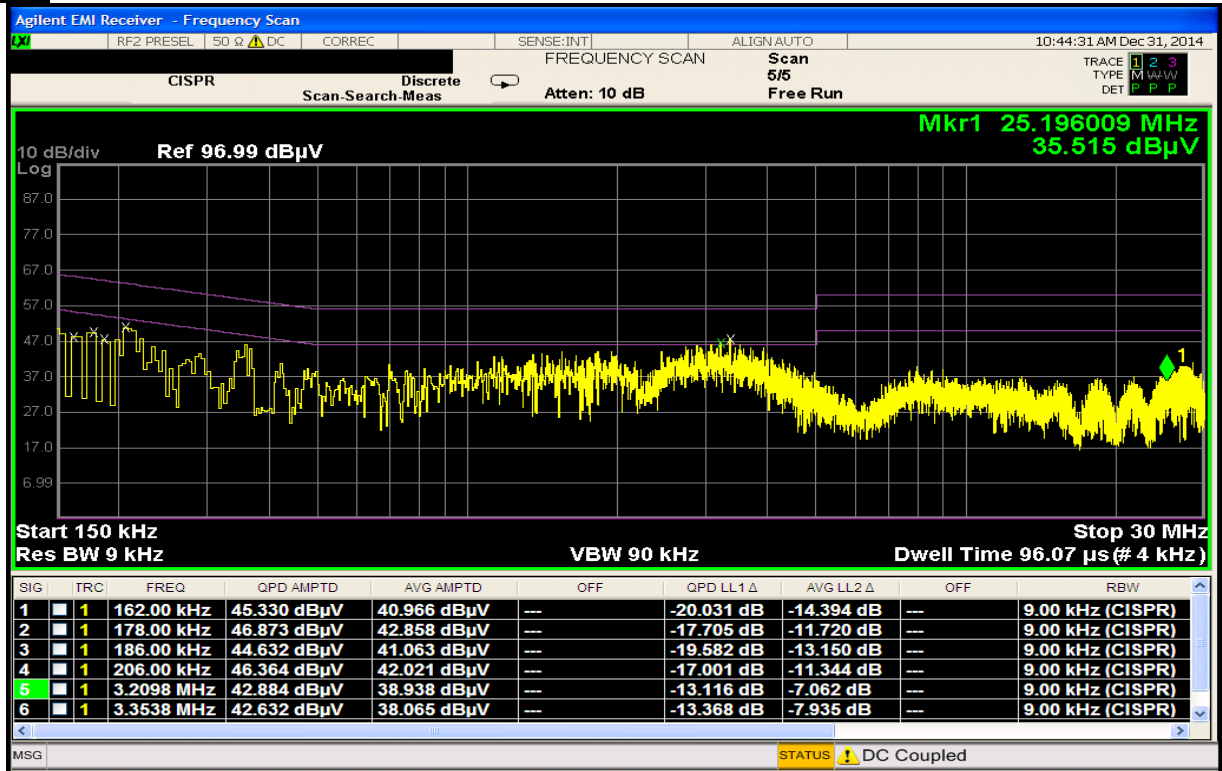
Plot 6-43. Line Conducted Plot with 802.11b (L1)
