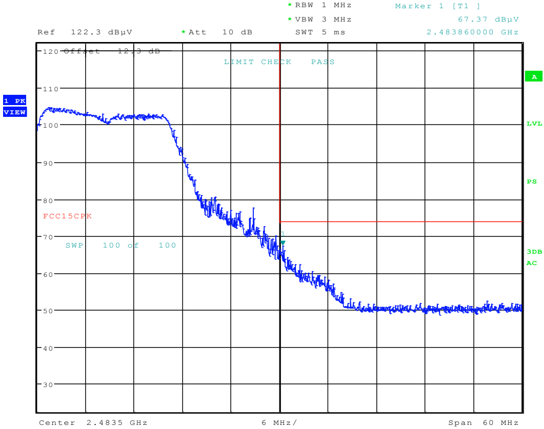
Plot 6-40. Radiated Restricted Upper Band Edge Measurement (Peak)
