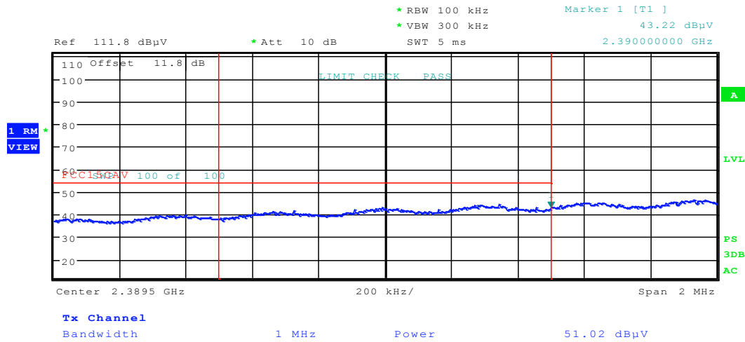
Plot 6-37. Radiated Restricted Lower Band Edge Measurement (Average)
