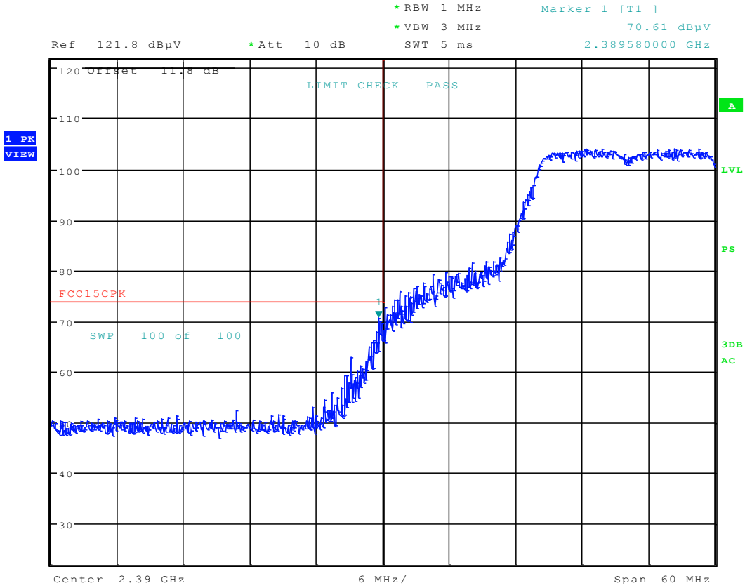
Plot 6-38. Radiated Restricted Lower Band Edge Measurement (Peak)
