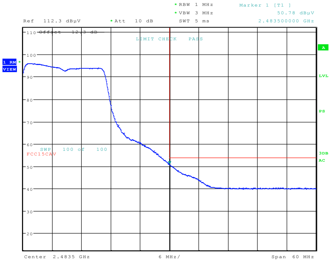
Plot 6-39. Radiated Restricted Upper Band Edge Measurement (Average)
