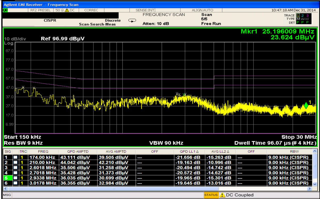
Plot 6-44. Line Conducted Plot with 802.11b (N)
